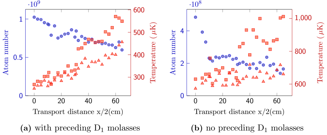
Figure 5.14: Magnetic transport round-trip experiments for ^{40}\text{K} . Atom number (dots) and temperature in x- and z-direction (squares and triangles, respectively) as functions of the transport distance. After the atoms reach the final transport position, the transport sequence is inverted and brings the atoms back to the MOT position x=0 , where the temperature and atom number are measured. (a) Roundtrip experiment with preceding D_1 molasses phase. The atom number decreases from 1 \times 10^9 to 6 \times 10^8 atoms for a complete round-trip from the MOT- to the science-chamber and back, yielding a transport efficiency of \sim 80\% . For a complete round-trip the temperature increases by 200(250) \mu\text{K} in z(x)-direction. The heating in x-direction is more pronounced, because of the direction change at the elbow. (b) Roundtrip experiment without preceding D_1 molasses phase. Compared to (a), the initial atom number is two times smaller, whereas the initial temperature is two times larger. The high initial temperature leads to a large atom loss until \sim 15 cm and leads to a more pronounced heating in x-direction.
