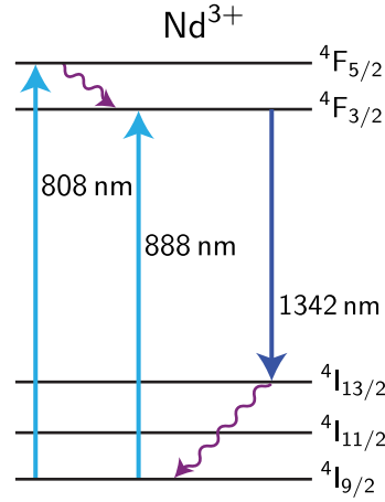
Figure 3.2: Simplified level scheme of the neodymium ion ( \text{Nd}^{3+} ) in the \text{YVO}_4 host crystal. The straight and wavy arrows denote photonic- and vibrational transitions, respectively. The laser source operates on the ^4F_{3/2} \rightarrow ^4I_{13/2} transition at 1342 nm. The metastable ^4F_{3/2} level can be pumped with 808 nm or 888 nm. The former transition has a significant higher absorption coefficient (see Fig. 3.4), and higher heating per cycle.
