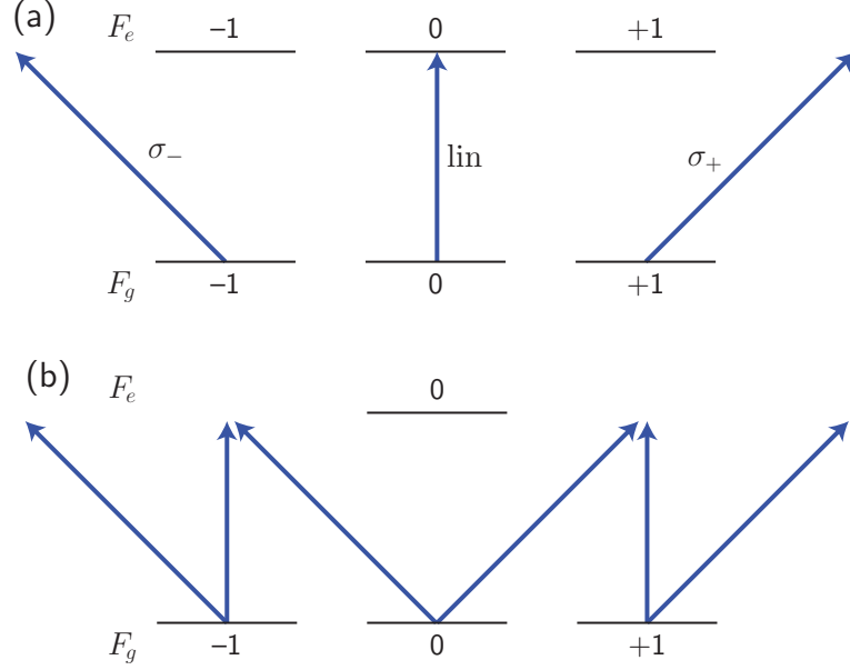
Figure 4.5: Dark states for a F \rightarrow F and F \rightarrow F - 1 transition. (a) F \rightarrow F : The atom interacts with \sigma_+ , \sigma_- and \pi polarized light. In each case a pure state exists that can not be excited by the light. For an arbitrary polarization there always exists a linear combination of the lower states forming a dark state. (b) F \rightarrow F - 1 : For any polarization two dark states are present.
