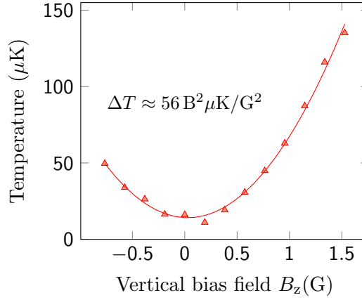
Figure 4.15: ^{40}\text{K} D_1 molasses temperature as a function of a vertical magnetic field bias B_z . The temperature has a minimum of \sim 11 \mu\text{K} and increases quadratically with \Delta T \approx 56 B^2 \mu\text{K}/\text{G}^2 . The number of atoms in the molasses is 3.2 \times 10^9 .
