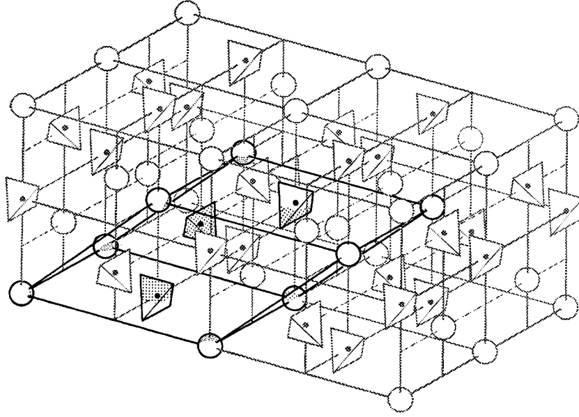
Figure 3.3: Zircon type crystal structure of \text{YVO}_4 (from [181]). The unit cell is marked in bold lines. Tetrahedra represent the \text{VO}_4^{3-} ions and balls indicate yttrium atoms.
