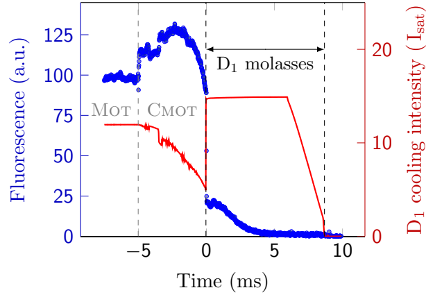
Figure 4.10: Measured fluorescence during the MOT, CMOT and the D_1 molasses phases (blue) for ^{40}\text{K} . The D_1 cooling intensity (Time>0, red) stays constant for 6 ms, I_{\text{cool}} = 14.7I_{\text{sat}} , and is linearly ramped to 0.8 I_{\text{sat}} in 3 ms. \delta = 2.3\Gamma and I_{\text{rep}} = I_{\text{cool}}/8 .
