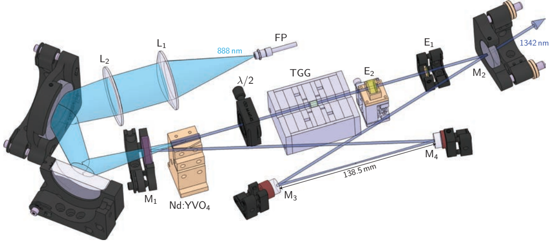
Figure 3.12: Design of the third laser generation. The fiber coupled pump source is labeled FP. Two lenses L_{1,2} focus the pump beam in the Nd:YVO 4 active medium. The zero-lens cavity mirrors M_1 compensates for thermal lensing of the cavity mode in the laser crystal. The \lambda/2 wave plate and the TGG Faraday crystal in a magnet force unidirectional operation. Two etalons E_{1,2} enable single-mode operation and tunability. The optical path of the generated laser beam is depicted in green. For some mechanical components (mirror mounts, Nd:YVO 4 mount, TGG magnets and E_2 mount) we show a sectional view to improve visibility of the beam path. The distance between the curved cavity mirrors M_1 and M_2 is 138.5 mm. The output beam is transmitted through M_2 ( \mathcal{T}_{\text{out}} = 7.5\% ). For a schematic drawing of the resonator setup see Fig. 3.11
