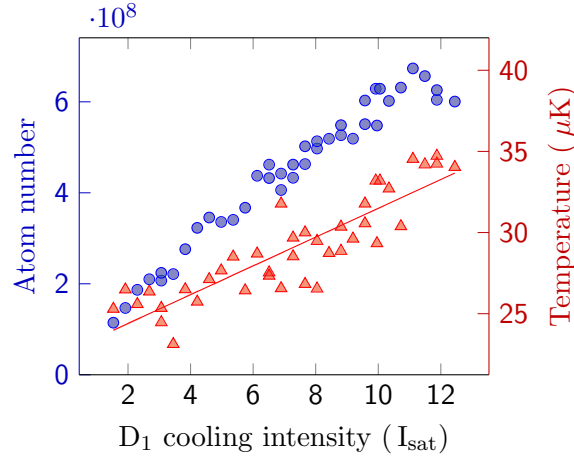
Figure 4.11: Number of atoms captured in the D_1 molasses (circles) and their temperature (triangles) as a function of the ^{40}\text{K} D_1 cooling beam intensity for \delta = 2.3\Gamma and I_{\text{rep}} = I_{\text{cool}}/8 . The number of atoms in the compressed MOT was 6.5 \times 10^8 and the capture efficiency reaches \sim 100\% for I \geq 11I_{\text{sat}}
