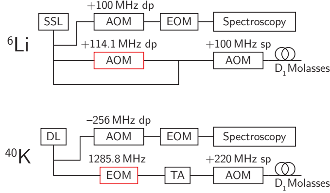
Figure 2.11: Laser systems of the D 1 molasses cooling schemes for ^6\text{Li} and ^{40}\text{K} . The frequencies and amplitudes of the various beams are controlled by AOMs in single pass (sp) or double pass (dp) configuration. An EOM creates the repumping frequency in the ^{40}\text{K} setup. The EOMs in the spectroscopy phase modulate a part of the beam for the laser's frequency stabilization. Single mode polarization maintaining fibers couple the beams to the experimental setup. The indicated AOM frequencies allow the generation of the beam frequencies required for the molasses cooling (see Fig. 2.3).
