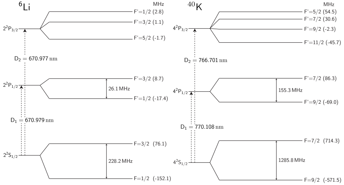
Figure 2.2: Level diagrams for the ^6\text{Li} and ^{40}\text{K} D 2 and D 1 lines with their respective hyperfine structures. The D lines of lithium lie in the red-, those for potassium in the near infrared spectral region. Note the small hyperfine splitting of the 2^2P_{3/2} manifold of ^6\text{Li} .
