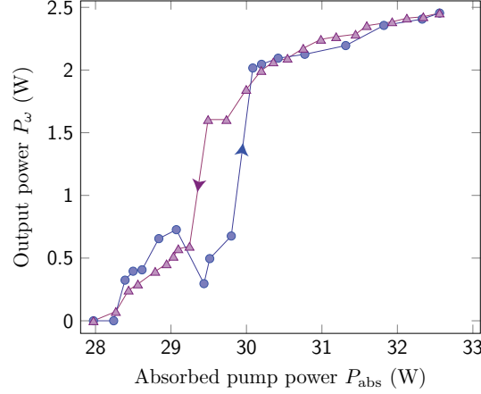
Figure 3.7: Infrared unidirectional output power P_\omega as a function of the absorbed pump power P_{\text{abs}} . The setup is optimized for the maximal absorbed pump power P_{\text{abs,max}} = 32.5 W. The oscillation threshold is found at P_{\text{abs}} \sim 28 W. The data shows hysteresis between P_{\text{abs}} = 29 W and 30 W, as indicated by the arrows for increasing or decreasing pump power. This behavior is typical for high-power designs. After a sudden rise the output power increases only slowly until it eventually reaches the maximum of 2.5 W at P_{\text{abs,max}} . Lines are guides to the eye only.
