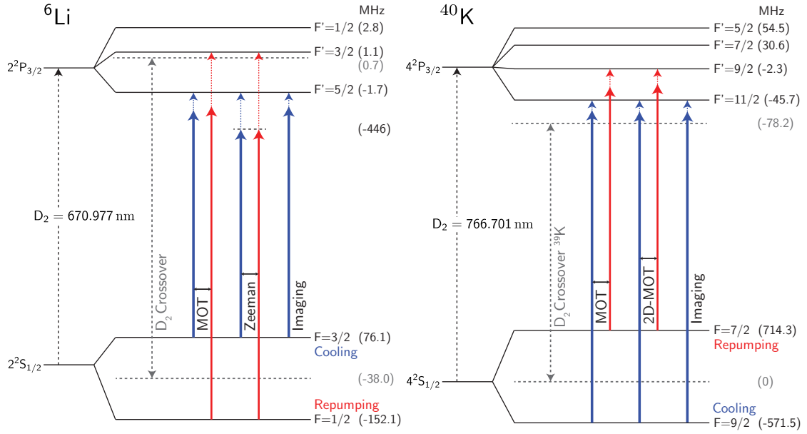
Figure 2.3: D 2 laser scheme for ^6\text{Li} and ^{40}\text{K} . Solid arrows illustrate the frequencies required for the dual-species MOT operation. Dashed arrows indicate the detunings from the corresponding transitions. The diode lasers are locked to the saturated absorption crossover signals 2^2S_{1/2} (|F = 1/2\rangle, |F = 3/2\rangle) \rightarrow 2^2P_{3/2} of ^6\text{Li} and 4^2S_{1/2} (|F = 1\rangle, |F = 2\rangle) \rightarrow 4^2P_{3/2} of ^{39}\text{K} .
