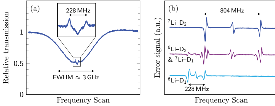
Figure 3.10: Doppler-free saturated absorption spectroscopy of the lithium D-lines. (a) Sample scan over the entire ^6\text{Li} \text{D}_1 Doppler-broadened absorption peak. The inset shows the sub-Doppler features. Similar spectra are obtained for all lithium D lines. (b) Error signals of all lithium D line transitions, generated by phase modulation spectroscopy. These signals provide an excellent reference for frequency-locking of the laser.
