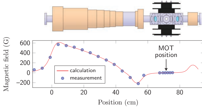
Figure 2.5: ^6\text{Li} Zeeman slower coil assembly (top) and generated axial magnetic field profile (bottom). The thermal atoms coming from the ^6\text{Li} -oven enter the coil assembly at the position 0, and a fraction of them is slowed down and finally captured in the ^6\text{Li} -MOT, which is located at 71.4 cm. A compensation coil placed on the opposite side of the MOT (at 84.1 cm) ensures that the magnetic field at the position of the MOT is zero. The coil assembly extends over 55 cm. (see [148])
