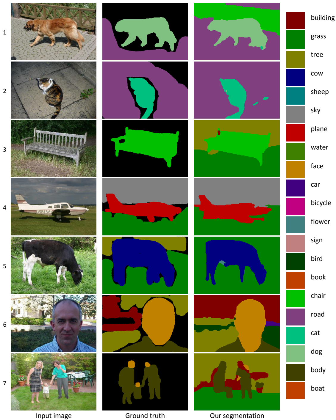
Figure 4.7: Some examples of semantic segmentation results on MSRC-21 dataset.
