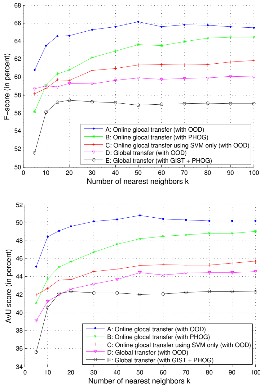
Figure 3.4: F-score (top) and AvU score (down) on Pascal VOC 2011 by varying the number of nearest neighbors k . The curve A shows the performance of our full method of online glocal transfer. The curve B shows the performance of online glocal transfer using PHOG for image retrieval rather than using OOD. The curve C shows the performance of online glocal transfer using only SVM prediction (without MRF optimization). The curve D shows the performance of global transfer [67] with the proposed OOD for image retrieval. The curve E shows the performance of original global transfer [67]. All results are computed by setting difficult areas of ground-truth as background.
