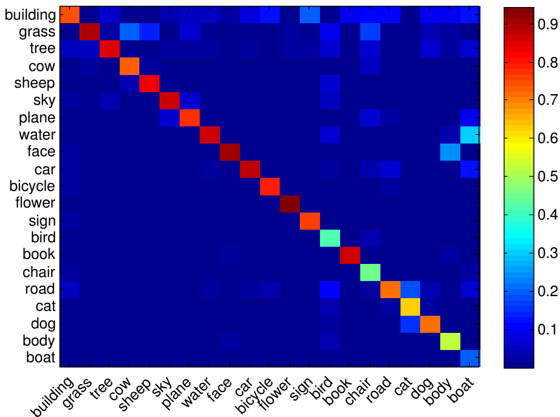
Figure 4.5: Confusion matrix of the proposed sparse-based approach on MSRC-21 dataset.
