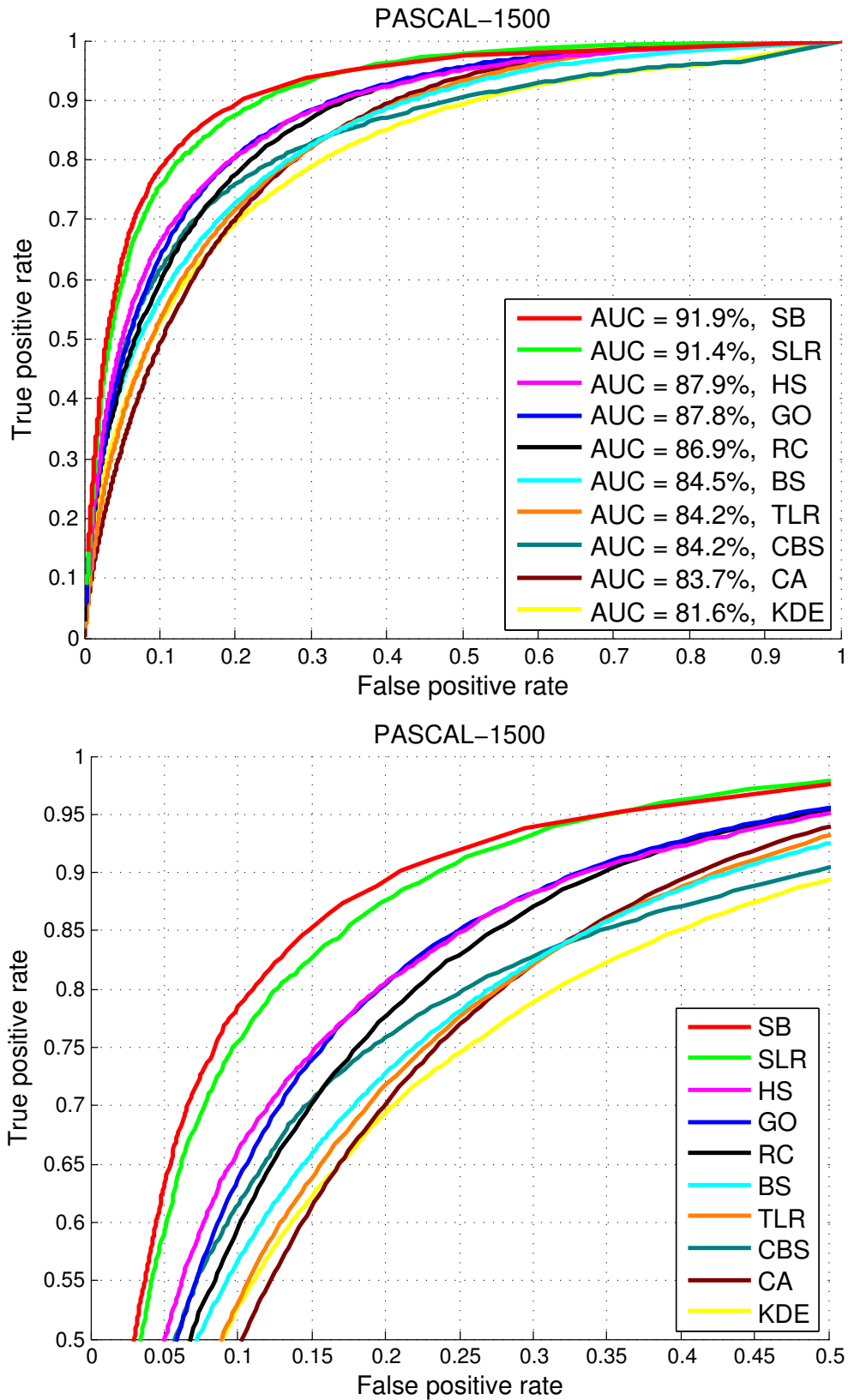
Figure 2.7: ROC curves and AUC scores of different models on PASCAL-1500 dataset. Top: complete ROC curves; Bottom: the zoomed top left corner of ROC curves. The models are ranked based on AUC scores in the legend.
