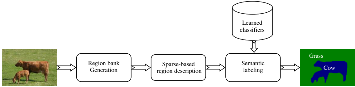
Figure 4.1: Framework of the proposed semantic image segmentation approach.
