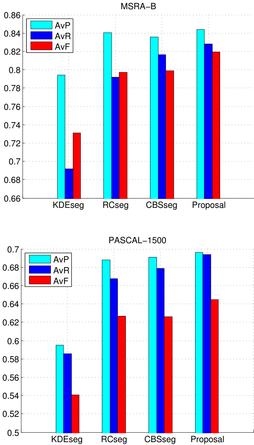
Figure 2.9: Average precision, recall and F-score for different saliency-based segmentation methods on MSRA-B (top) and PASCAL-1500 (bottom) datasets.
