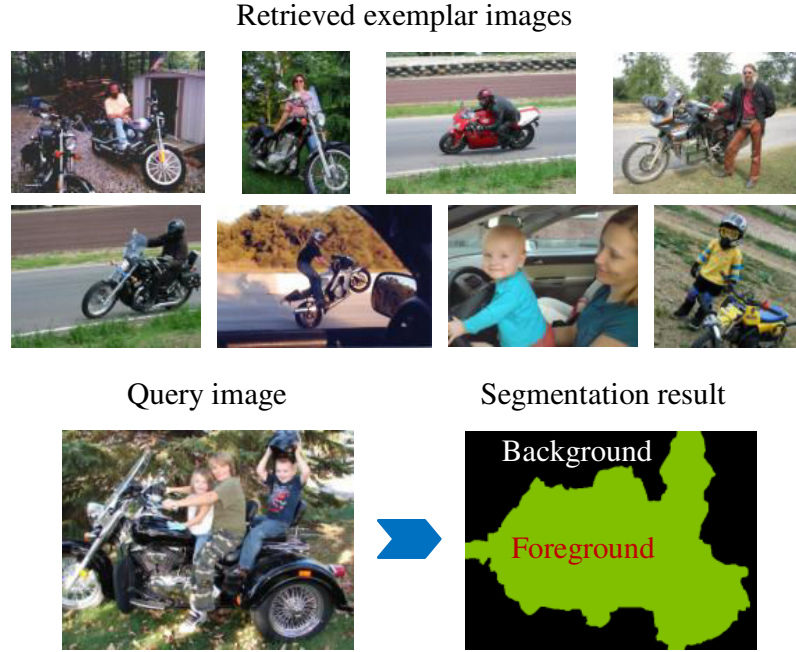
Figure 3.1: Given a query image (bottom left), we first retrieve globally similar exemplars in the annotated dataset (top) and then transfer their segmentation masks to the query image (bottom right).
