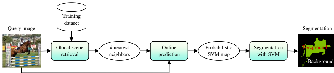
Figure 3.2: Generic framework of online glocal transfer which consists of three core algorithmic modules: glocal scene retrieval, online prediction and segmentation with SVM prior.
