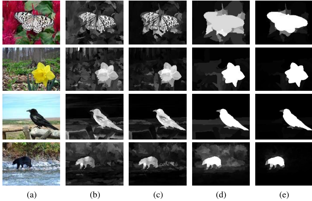
Figure 2.5: Some examples of saliency maps generated by the proposed saliency model with different configurations. (a) input image; (b) results of LRMR model using raw feature only; (c) results of LRMR model with segmentation prior; (d) results of full SLR model: LRMR model with segmentation prior and post-smoothing component; (e) results of SLR-based saliency boosting (SB) model.
