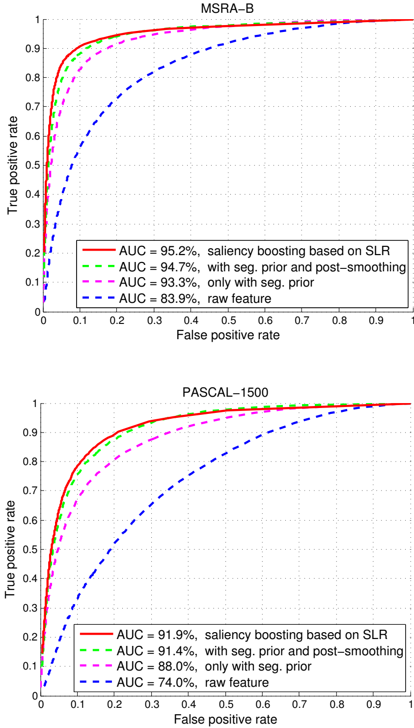
Figure 2.4: ROC curves and AUC scores OF the proposed model with different configurations on MSRA-B (top) and PASCAL-1500 (bottom) datasets. the dashed curves show the performance of SLR model using different components. The solid curve shows the performance of SB model.
