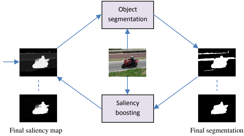
Figure 2.3: Unified framework of joint object segmentation and saliency boosting.
