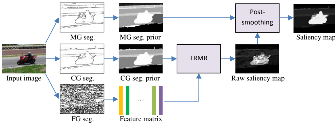
Figure 2.1: Framework of the proposed saliency model. Input image is firstly segmented into three levels. Feature descriptors are accumulated within superpixels of fine-grained (FG) segmentation. Segmentation priors are derived from the medium-grained (MG) segmentation and coarse-grained (CG) segmentation, respectively. The final saliency map is obtained by smoothing the raw saliency map generated by LRMR model with the MG segmentation prior.
