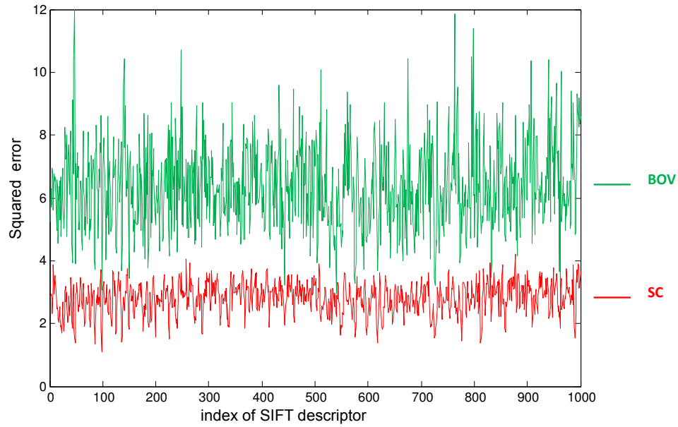
Figure 4.3: Squared errors generated by bag of visual-words (BOV) and sparse coding (SC) for randomly selected SIFT descriptors.
