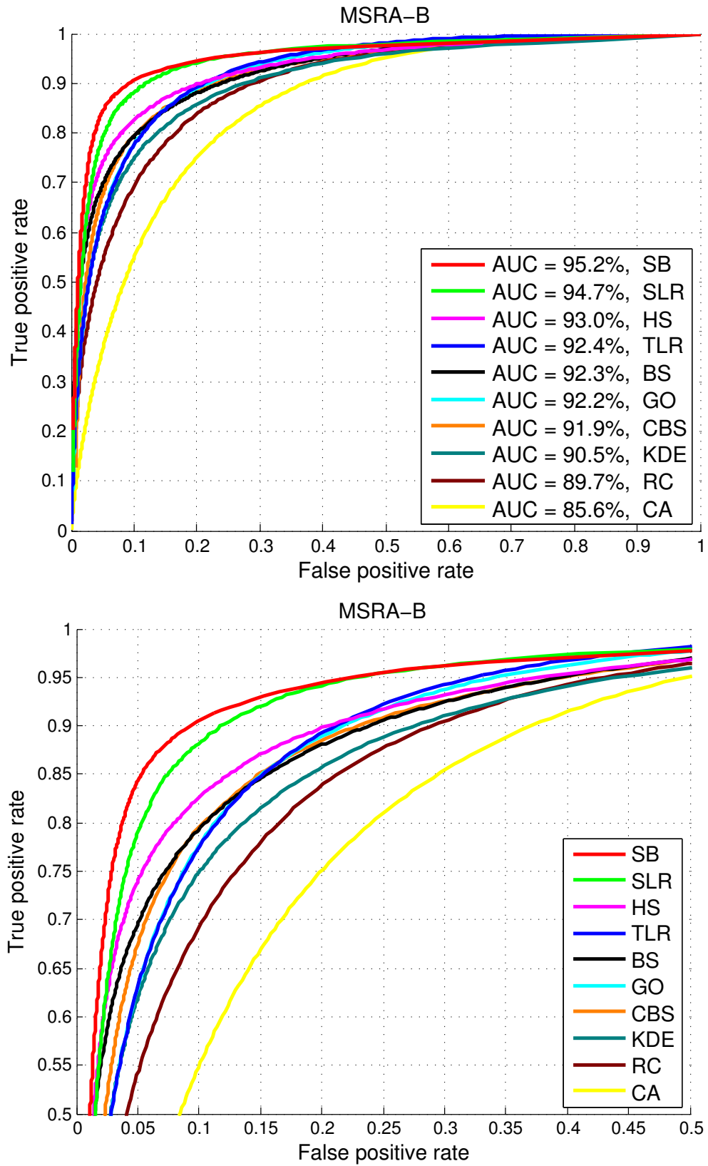
Figure 2.6: ROC curves and AUC scores of different models on MSRA-B dataset. Top: complete ROC curves; Bottom: the zoomed top left corner of ROC curves. The models are ranked based on AUC scores in the legend.
