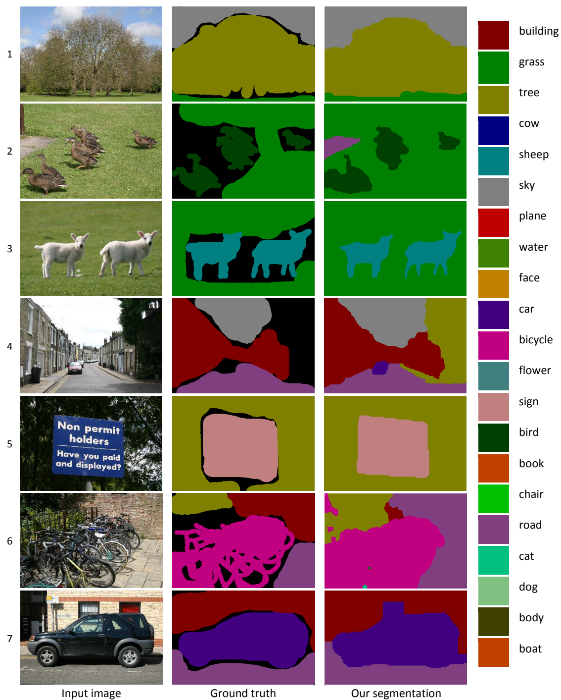
Figure 4.6: Some examples of semantic segmentation results on MSRC-21 dataset.
