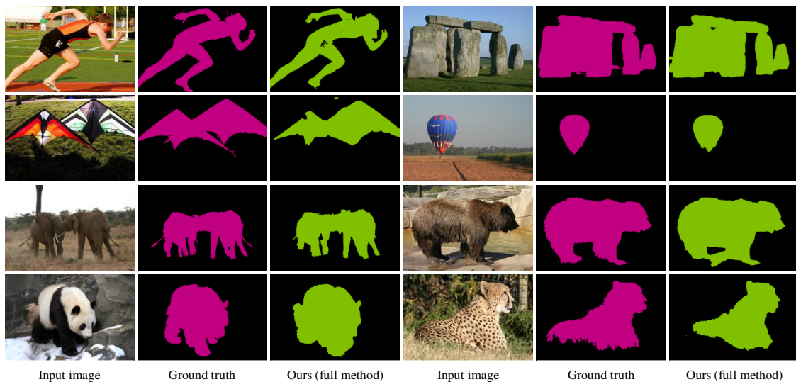
Figure 3.7: Some segmentation results on iCoseg dataset produced by the proposed approach. All results are generated by transferring exemplar segmentations of Pascal VOC 2011 to images of iCoseg dataset.
