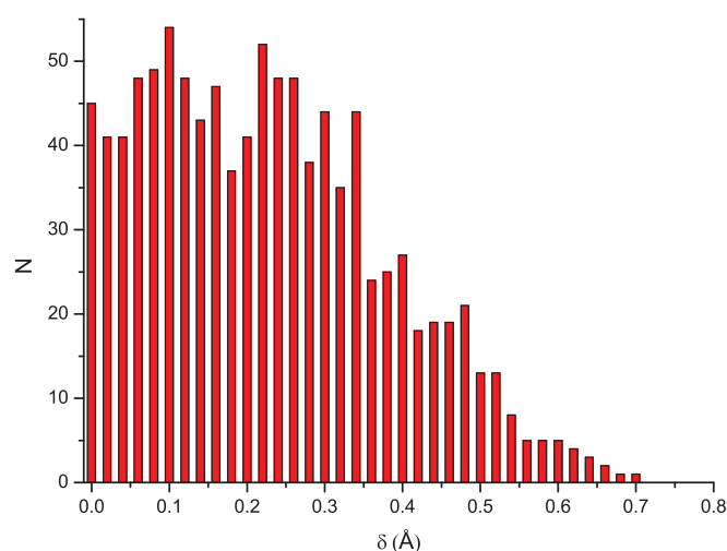
Figure 4.14: Distribution of the differences in bond lengths \delta for all BO atoms in the modelled glass.
