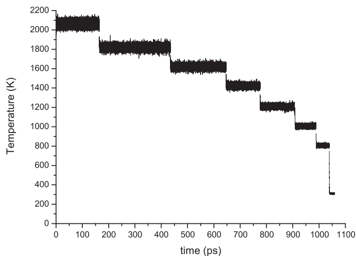
Figure 4.3: Temperature as a function of time in the test TeO 2 glass preparation procedure.
