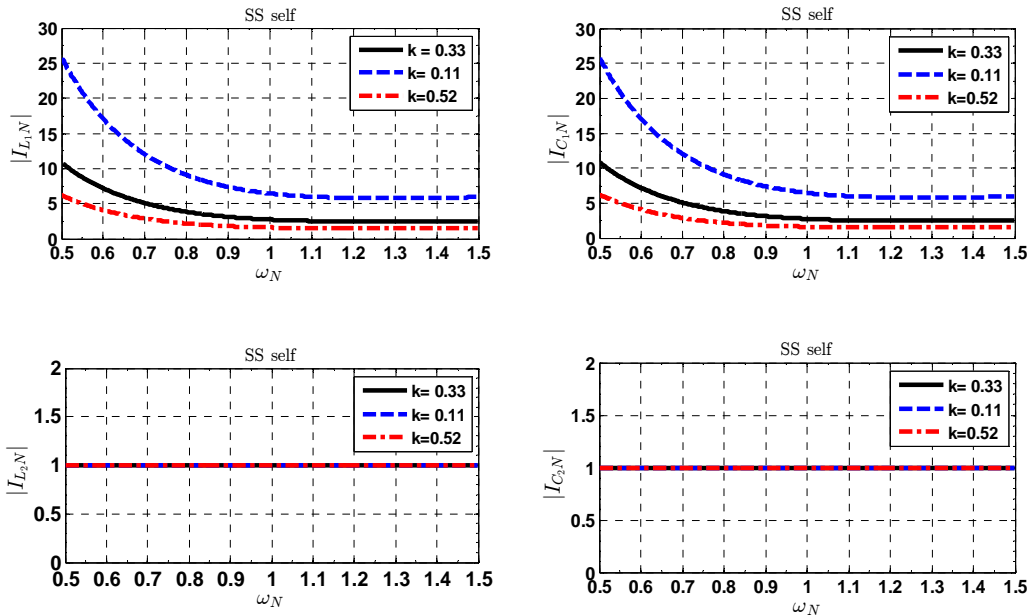
Fig. B.4: SS leakage compensation topology normalized L's and C's Currents of the resonant circuit as a function of the normalized frequency \omega_N for different k
