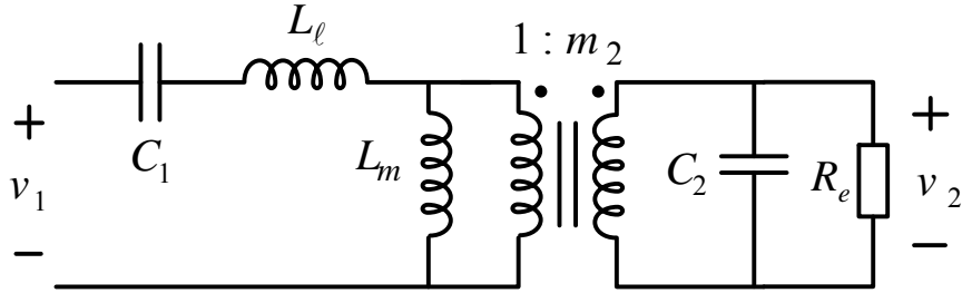
Fig. I.14: SP compensation
