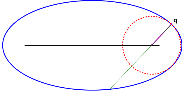
Figure 5-1: Thickness on an ellipse. The medial axis is depicted in black. The thickness (purple line) is defined as the radius of the maximal inscribed ball (red dotted line) associated to a boundary point \mathbf{q} . The diameter is depicted in green. Notice that taking half the diameter value is different from the computing the thickness, as it yields a larger value.
