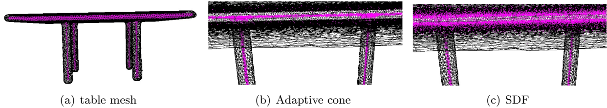
Figure 5-3: Half diameter cloud resulting from the SDF estimation and our procedure. 5-3(a) : half-diameter points for a mesh of a table. 5-3(b) : close-up on the points (purple), representing projections of samples at half their estimated \delta value along the normal, using the adaptive-opening cone algorithm. This configuration corresponds to the parallel planes case. 5-3(c) : same close-up, but points are the centers of facets projected at half their SDF value. In this case, two distinct parallel planes of points are created, due to the systematic overestimation of the actual diameter.
