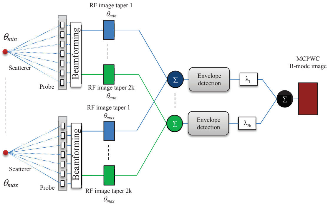
Figure 3.14: B-mode image reconstruction strategies for multitaper coherent plane wave compounding (MCPWC). The RF images of all illuminations with different angles and built for the same taper are averaged. After the envelope detection, the B-mode images obtained with different tapers are averaged to produce the final MCPWC B-mode image.
