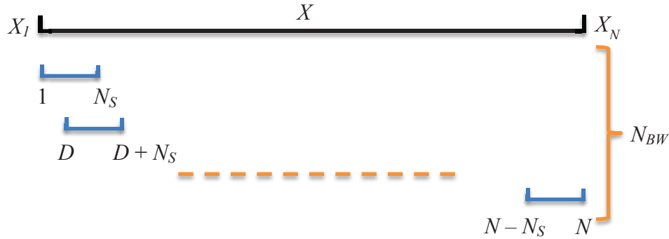
Figure B. 1: Illustration of the segmentation for a time series X with the Welch periodogram method. The times series has N points and the Welch method has N_{BW} segments with a size N_S and the overlapped segments start at the position D of the time series.
