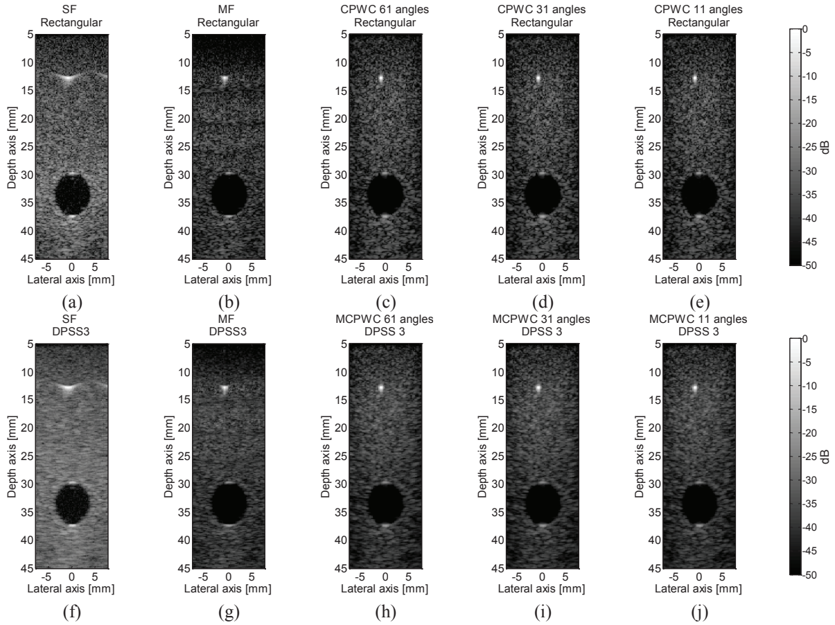
Figure E. 2: Log compressed images of hypo echoic cyst obtained by the ULA-OP scanner, (a, f) one focal depth at 32.5 mm without and with three apodization tapers on reception, (b, g) MF without and with three apodization tapers on reception, (c-e) CPWC and (h-j) MCPWC with three apodization tapers on reception and 61, 31 and 11 transmitted angles.
