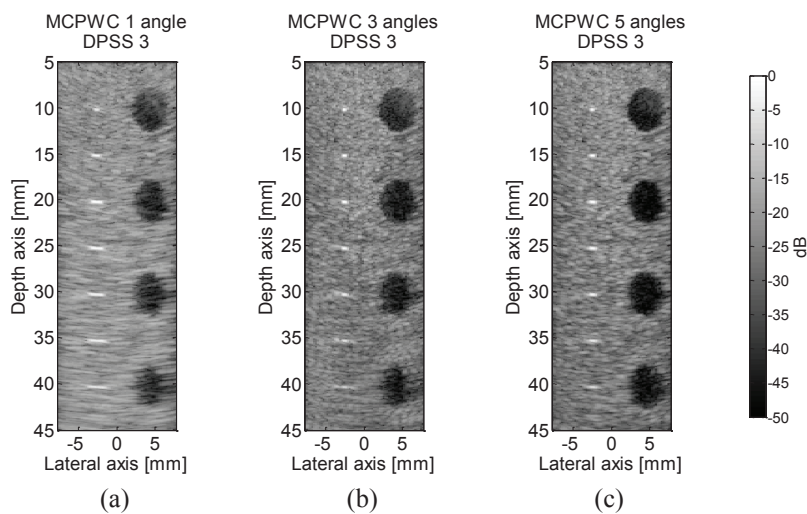
Figure 3.15: MCPWC Log compressed ultrasound images of wires and hypoechoic cysts simulated by CREANUIS, for (a) one transmitted angle, (b) three transmitted angles and (c) five transmitted angles.
