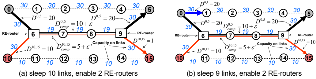
Figure 3.2: GreenRE with 50% of traffic redundancy
