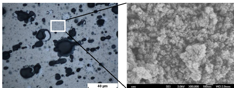
Figure 3.54: Coating obtained at the moment of maximum arc voltage, shown in Figure 3.53, measured by the optical microscope, using the objective magnification 100x, with the marked region measured by SEM and presented on the right.
