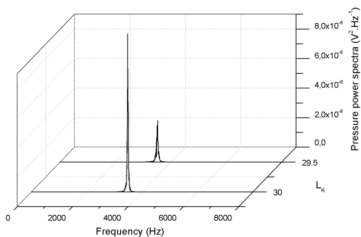
Figure 2.23: Pressure power spectra of filtered Helmholtz mode for L_k : 30 and 29.5 mm [74].
