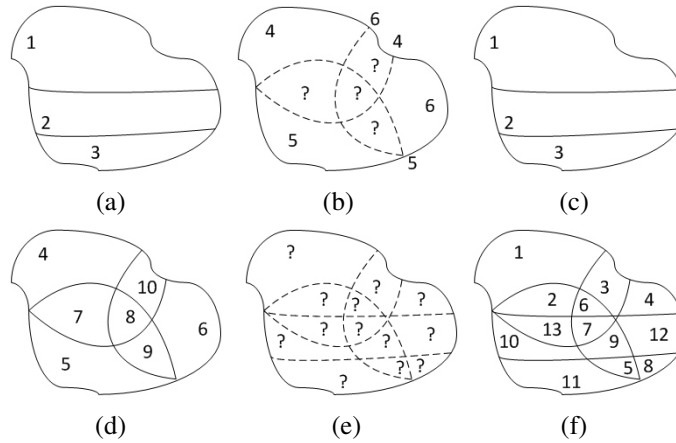
Figure 8.4: Overlapping and partitions when generating test models.
