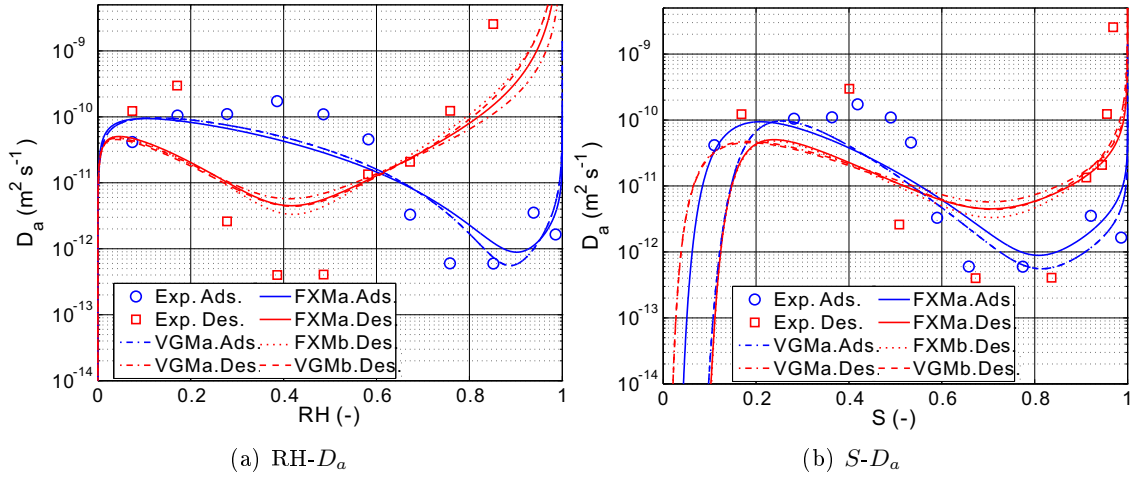
Figure 6.3: Fitted D_a curves for Paste2 during both desorption and adsorption processes.
