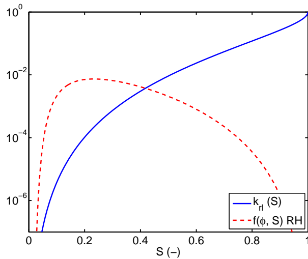
Figure 2.15: Relationships of f(\phi, S)RH(S) vs. S and k_{rl}(S) vs. S for Paste4.
