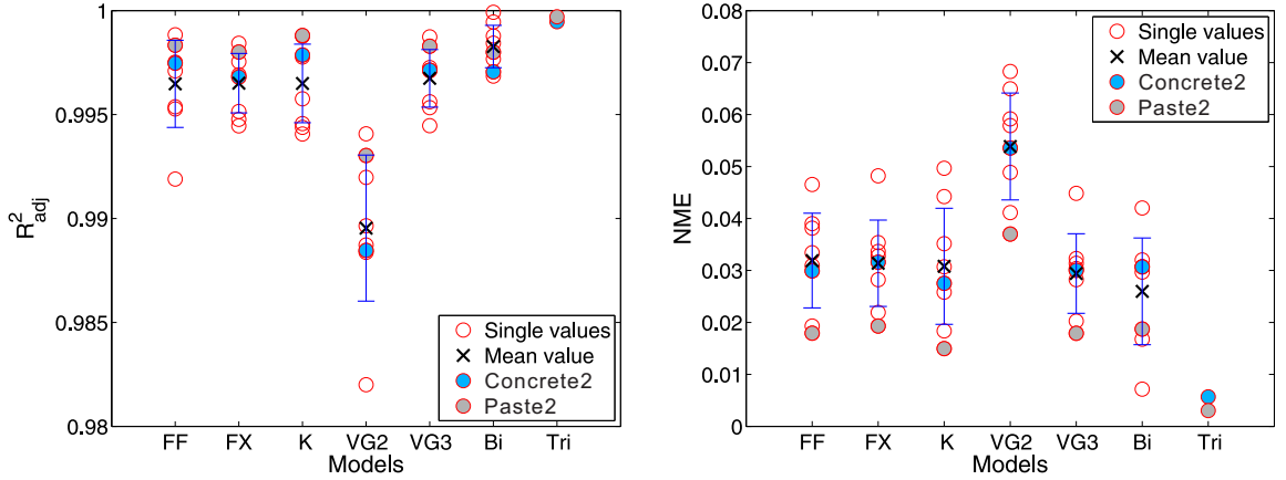
Figure 3.4: Comparison of R_{adj}^2 and NME for the main adsorption isotherms. Each circle (o) in the figure stands for one material (see Table 3.2). Concrete2 and Paste2 are highlighted. The error bars represent the standard deviation for each studied statistical criteria ( R_{adj}^2 and NME) and each model.
