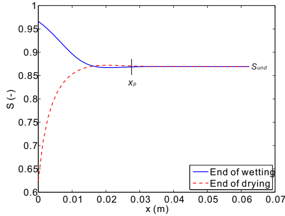
Figure 5.20: Definitions of the undisturbed saturation S_{und} and the moisture penetration depth x_p after a number of cycles.
