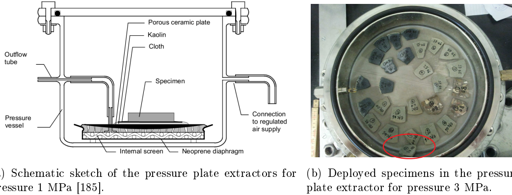
Figure 4.8: Pressure plate extractors used in measurements at Lund University. The circled specimen was blown away from the center due to the suddenly increased gas pressure.
