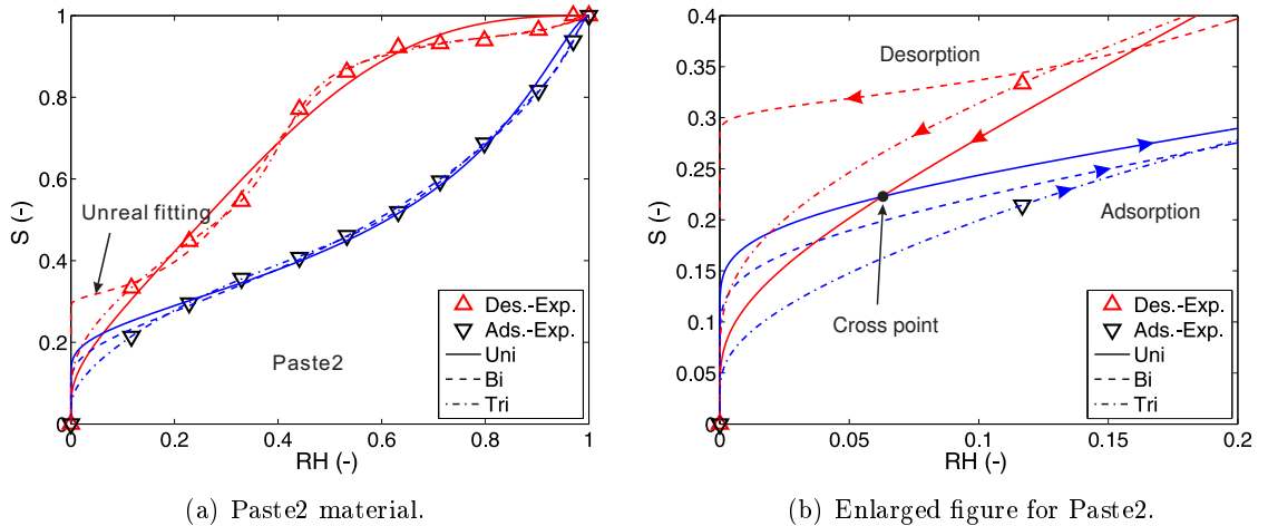
Figure 3.5: Fitting results for Paste2 material to compare results of uni-(VG2), bi- and tri-modal models. Fitting results for low RH values are shown in the enlarged figure.
