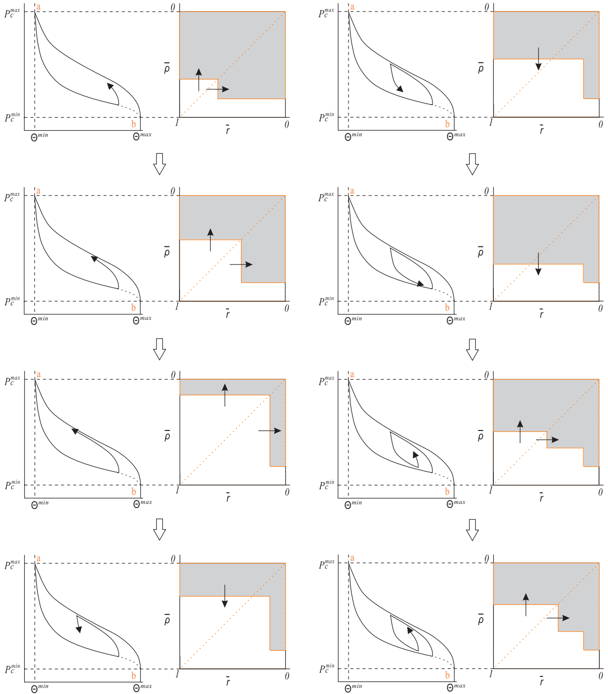
Figure 3.10: The scanning loops simulated by Mualem's diagram. The first drying, second wetting and third drying scanning curves are shown in this figure.
