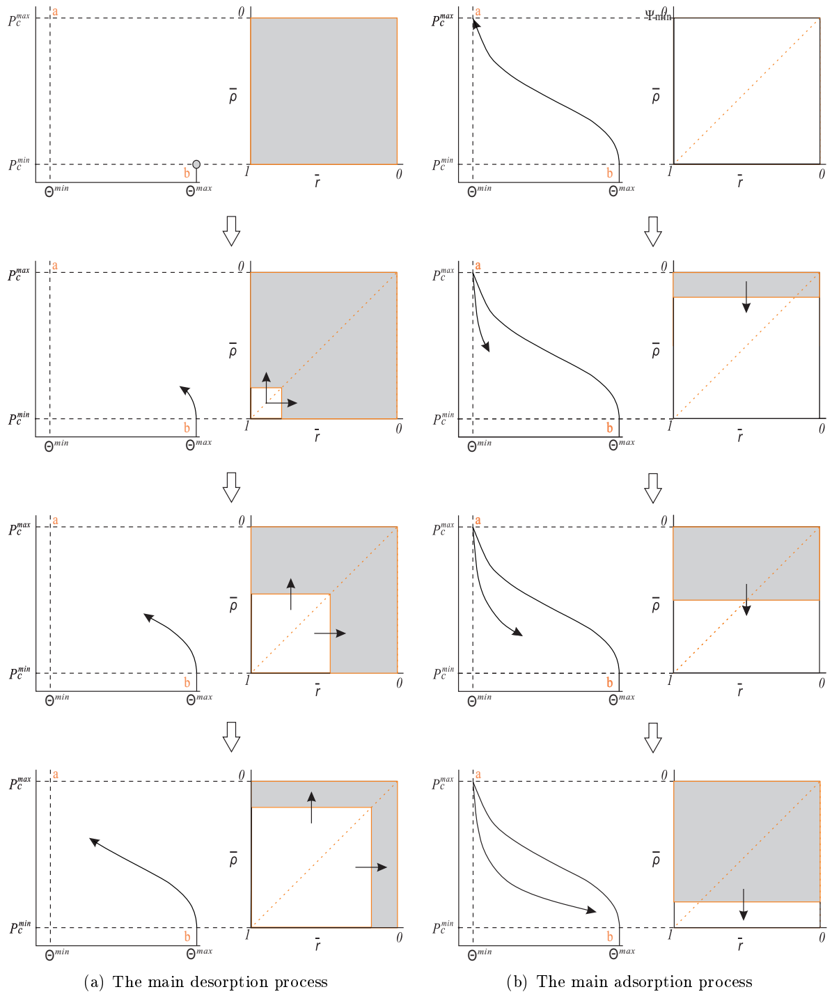
Figure 3.2: Schematic representation of Mualem's diagram [53] for the main desorption and adsorption processes. The gray domain represents completely-filled pores and the blank domain stands for fully-dried pores.
