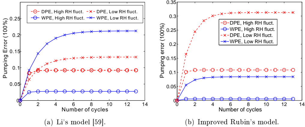
Figure 3.20: The evolution of PEs calculated based on two RH fluctuations.
