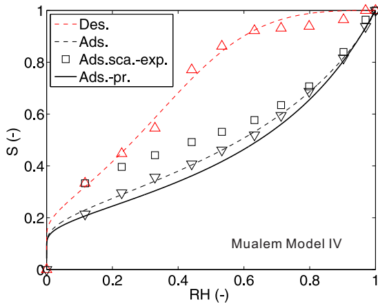
(c) Mualem Model IV [167], RH_1 = 12\% .
