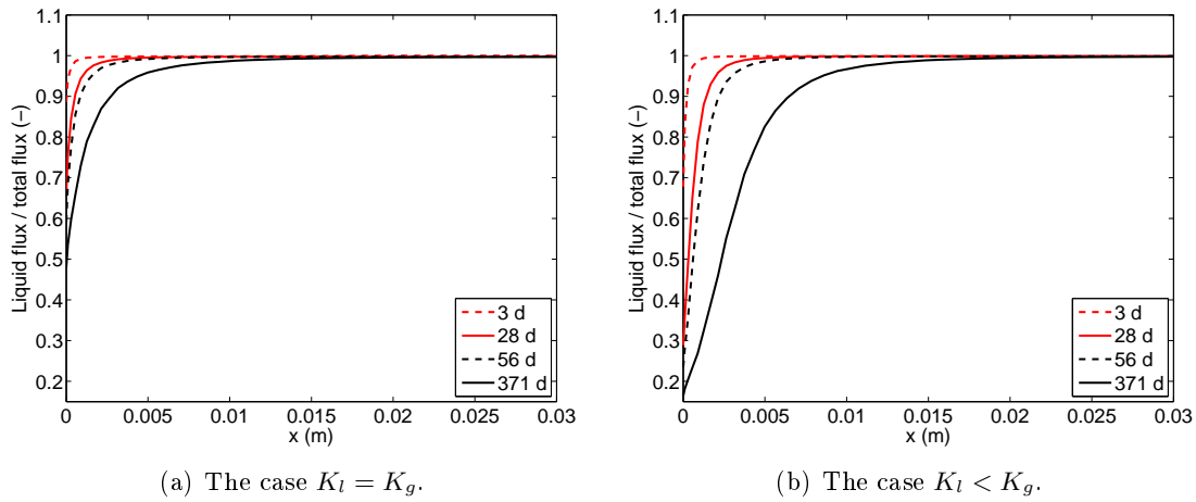
Figure 2.18: Ratio of liquid-water flux to the total flux in the material during drying of Paste4 ( RH_0 = 89\% and RH^e = 53.5\% ).
