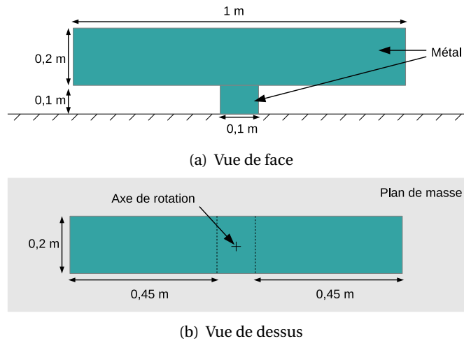
FIGURE 2.10 – Élément diffractant
