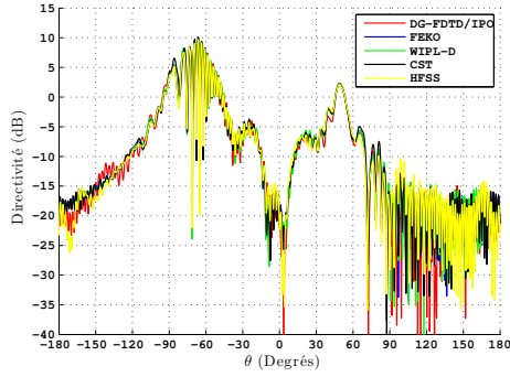
(a) CO-polar ( E_\theta ), plan ( x_0z ).
