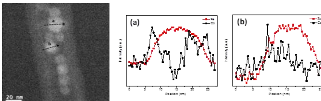
Figure IV.16. (Left) STEM dark-field image of \text{Fe}_{3-x}\text{O}_4/\text{CoO}@/\text{NPs} inside CNTs showing the position of NPs [(a) and (b)] along line a and b: corresponding Fe and Co atoms amounts (%) as a function of the NP section.
