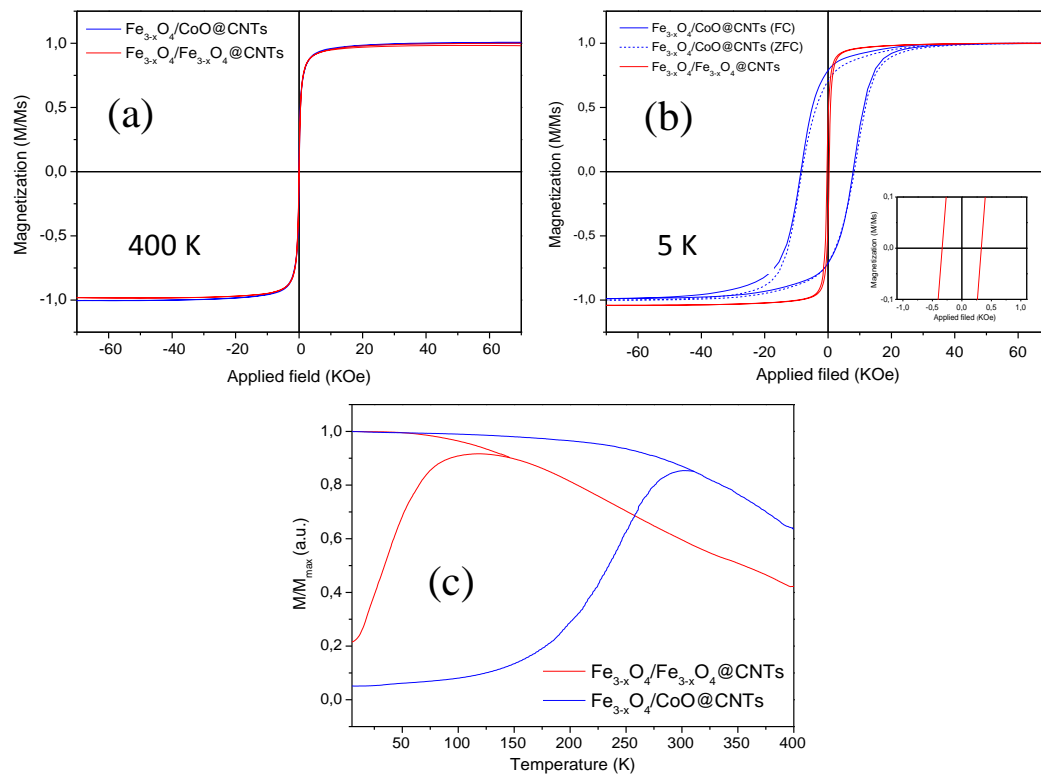
Figure IV.18. (a) Magnetization curves of \text{Fe}_{3-x}\text{O}_4/\text{CoO}@CNTs and \text{Fe}_{3-x}\text{O}_4/\text{Fe}_{3-x}\text{O}_4@CNTs at 400K and (b) before (ZFC) and after (FC) cooling from 400 K to 5 K under magnetic field and \text{Fe}_{3-x}\text{O}_4/\text{Fe}_{3-x}\text{O}_4@CNTs at 5K (Inset: enlargement of curve of \text{Fe}_{3-x}\text{O}_4/\text{Fe}_{3-x}\text{O}_4@CNTs ). (c) Magnetization versus temperature (ZFC -blue - and FC - red - curves) of \text{Fe}_{3-x}\text{O}_4/\text{CoO}@CNTs and \text{Fe}_{3-x}\text{O}_4/\text{Fe}_{3-x}\text{O}_4@CNTs .
