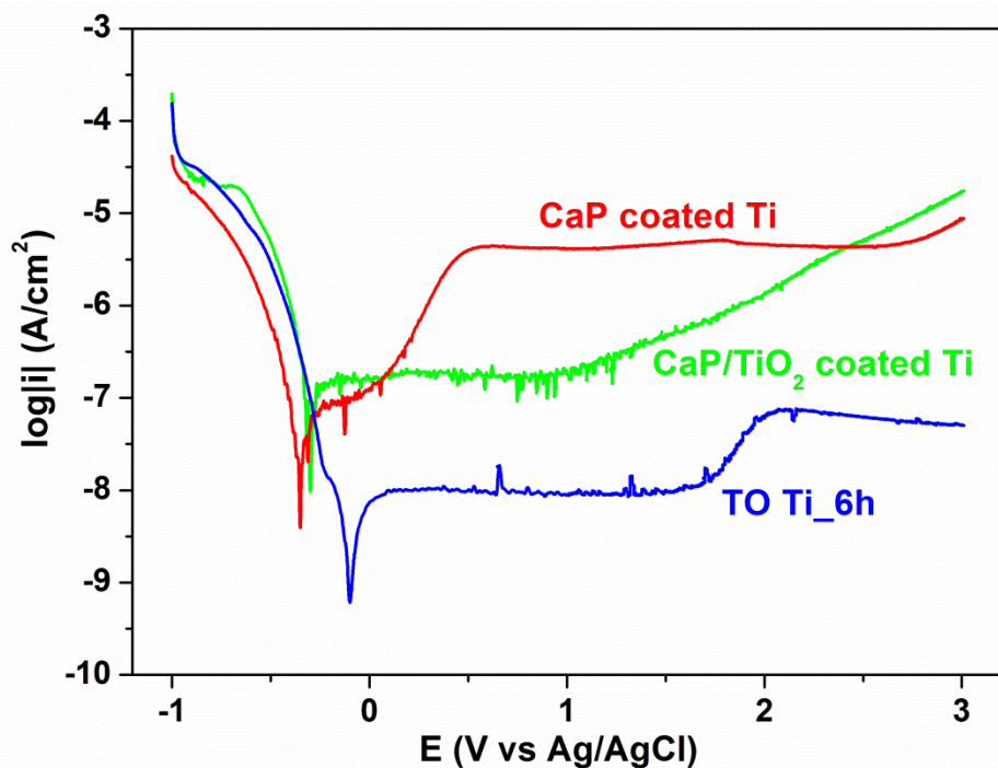
Figure 7-6 Potentiodynamic polarization curve of CaP/TiO 2 bioceramic film coated Ti (green line), CaP bioactive film coated Ti (red line) and TO Ti 6 h (blue line) from -1 V to 3 V vs. Ag/AgCl at a scan rate of 1 mV/s measured at immersion time of 3 h under static condition in the PBS solution.
