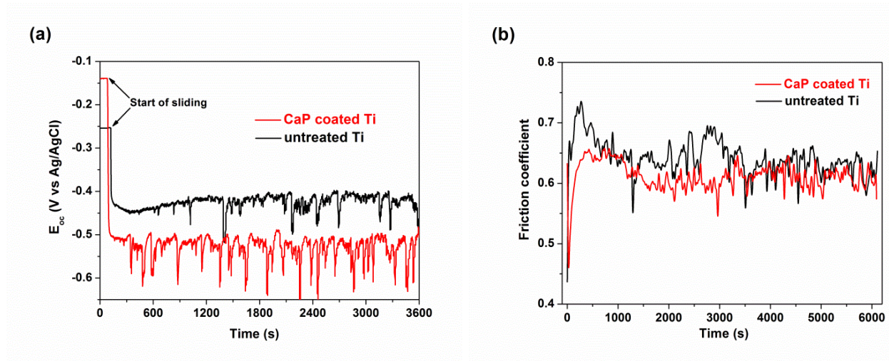
Figure 6-12 OCP evolution (a) and friction coefficient (b) of CaP bioactive film coated Ti (red line) and untreated Ti (black line) during continuous unidirectional sliding tests performed at F_n of 500 mN.
