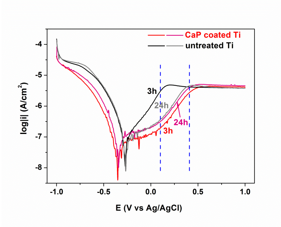
Figure 6-10 Potentiodynamic polarization curves of CaP bioactive film coated Ti and untreated Ti from -1 V to 1 V vs. Ag/AgCl at a scan rate of 1 mV/s measured at immersion time of 3 h and 24 h under static condition in the PBS solution.
