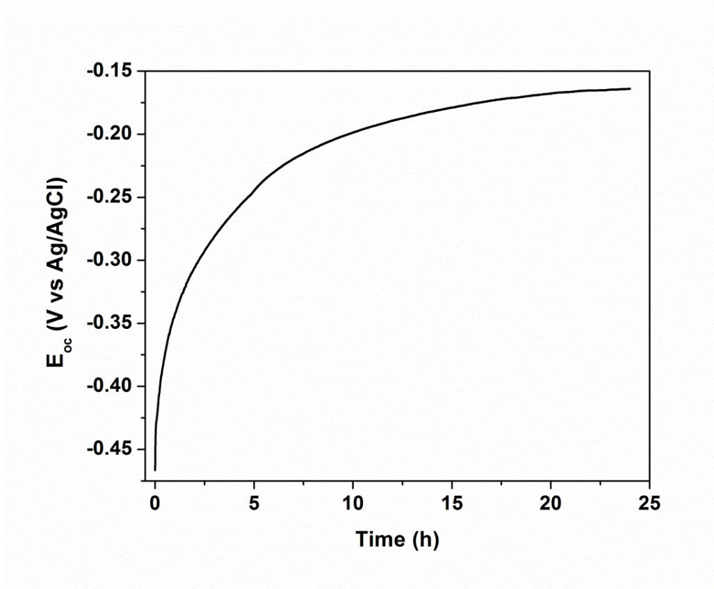
Figure 4-1 OCP evolution of cp Ti within 24 h under static condition in the PBS solution.
