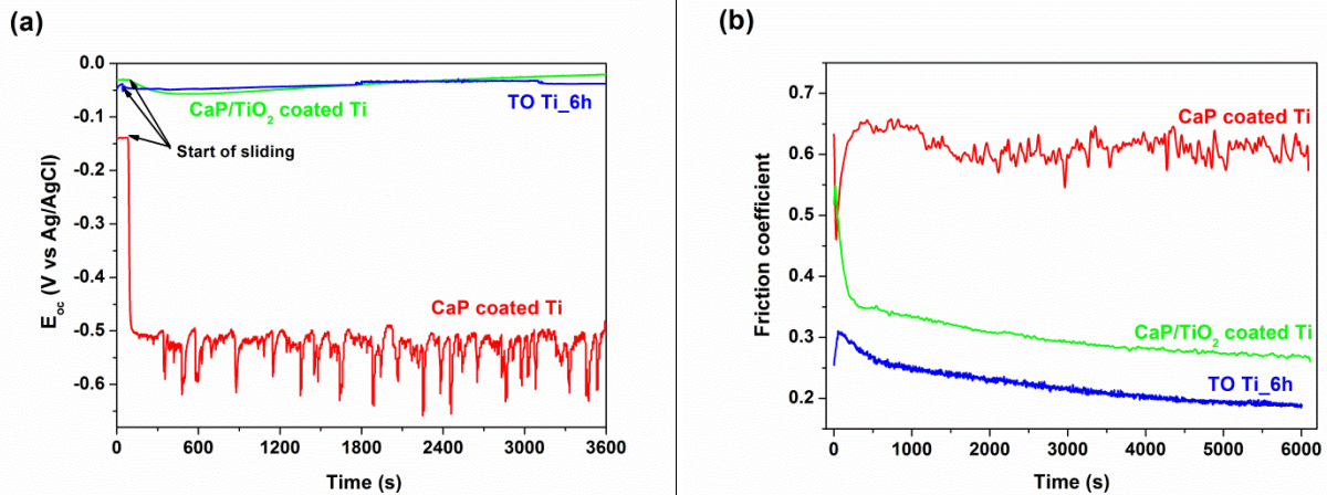
Figure 7-9 OCP evolution (a) and friction coefficient (b) of CaP/TiO 2 bioceramic film coated Ti (green line), CaP bioactive film coated Ti (red line) and TO Ti_6h (blue line) during continuous unidirectional sliding tests performed at F_n of 500 mN.
