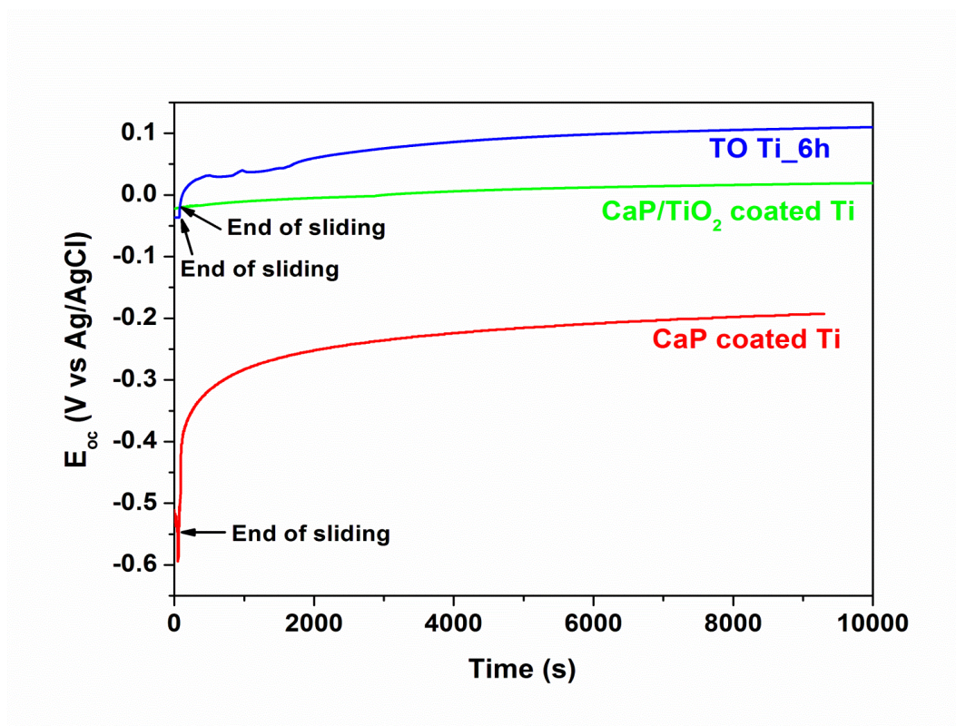
Figure 7-11 OCP evolution of CaP/TiO 2 bioceramic film coated Ti (green line), CaP bioactive film coated Ti (red line) and TO Ti 6h (blue line) after continuous unidirectional sliding tests.
