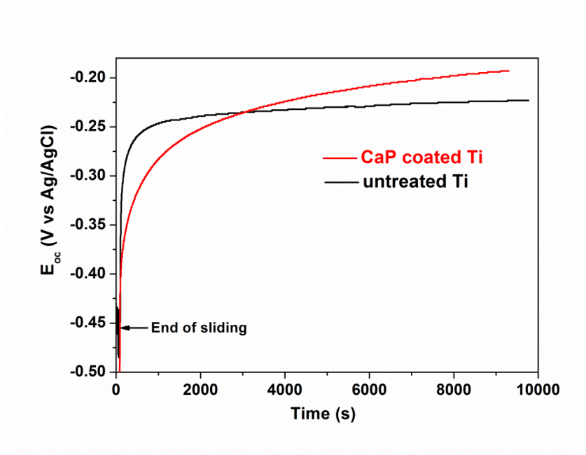
Figure 6-13 OCP evolution of CaP bioactive film coated Ti (red line) and untreated Ti (black line) after continuous unidirectional sliding tests.
