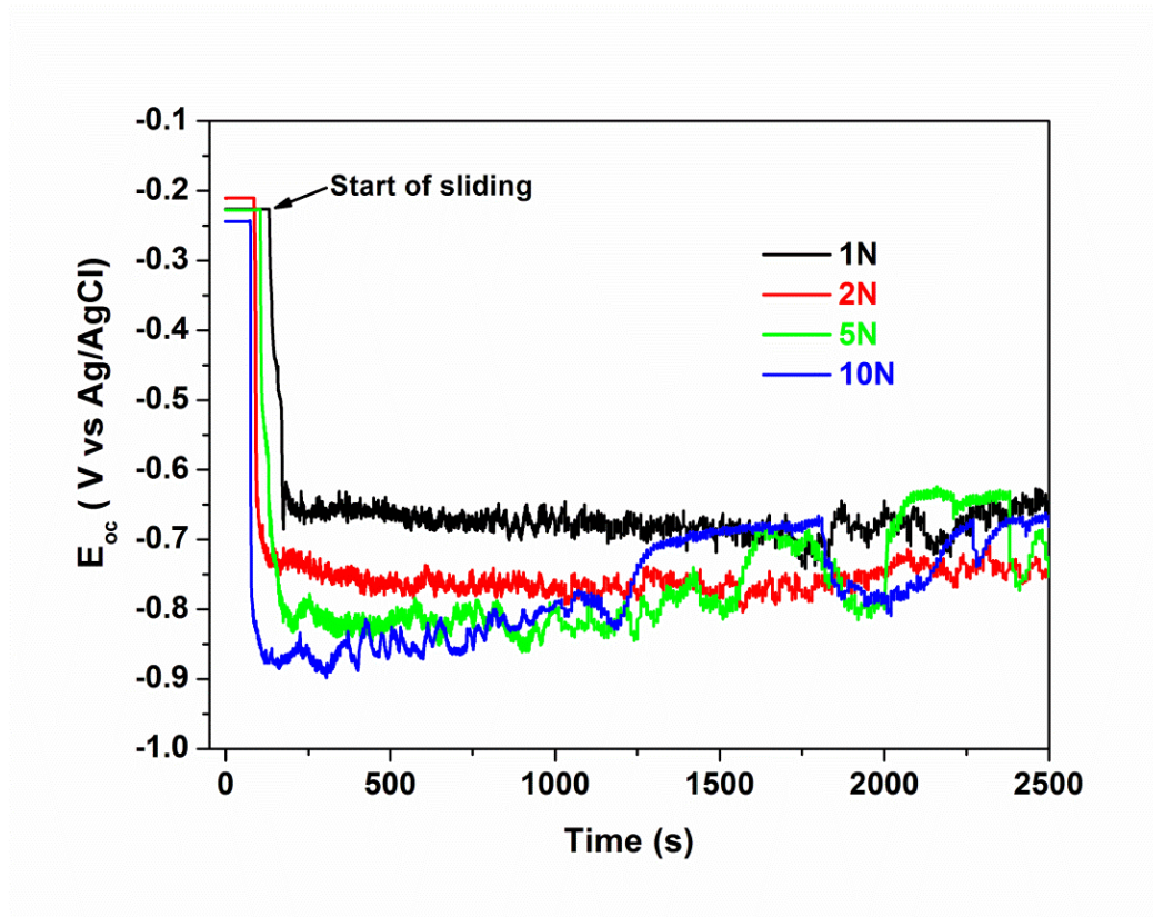
Figure 4-7 OCP evolution of cp Ti during continuous unidirectional sliding tests performed at different F_n of 1 N, 2 N, 5 N and 10 N.
