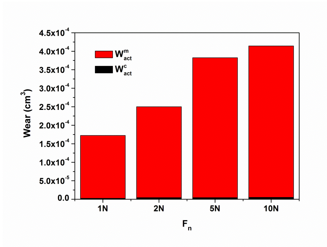
Figure 4-14 Contribution of two different tribocorrosion components to the total volumetric material loss inside the sliding track of cp Ti under continuous mechanical loaded condition at different F_n from 1 N to 10 N in the PBS solution.
