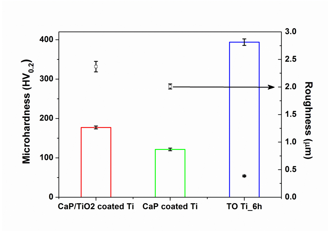
Figure 7-2 Microhardness and surface roughness of CaP/TiO 2 bioceramic film coated Ti, CaP bioactive film coated Ti and TO Ti_6h.
