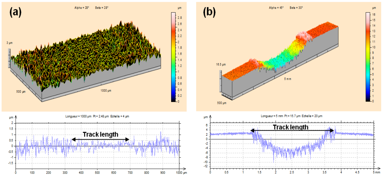
Figure 5-14 Profiles of TO Ti prepared at 650 °C for 48 h (a) and untreated Ti (b) after continuous unidirectional sliding tests at F_n of 5 N in the PBS solution.
