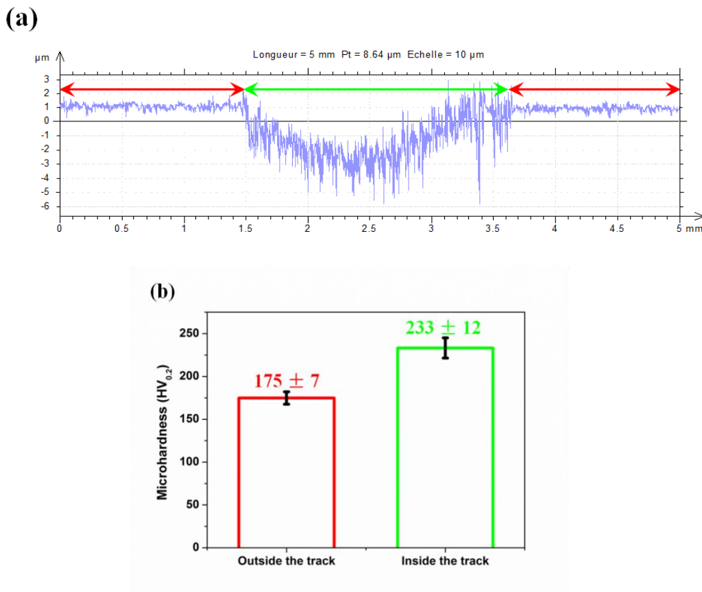
Figure 4-13 Profile of the track (a) and microhardness (b) of cp Ti outside (red line), inside (green line) the track area after tribocorrosion test at F_n of 1 N.
