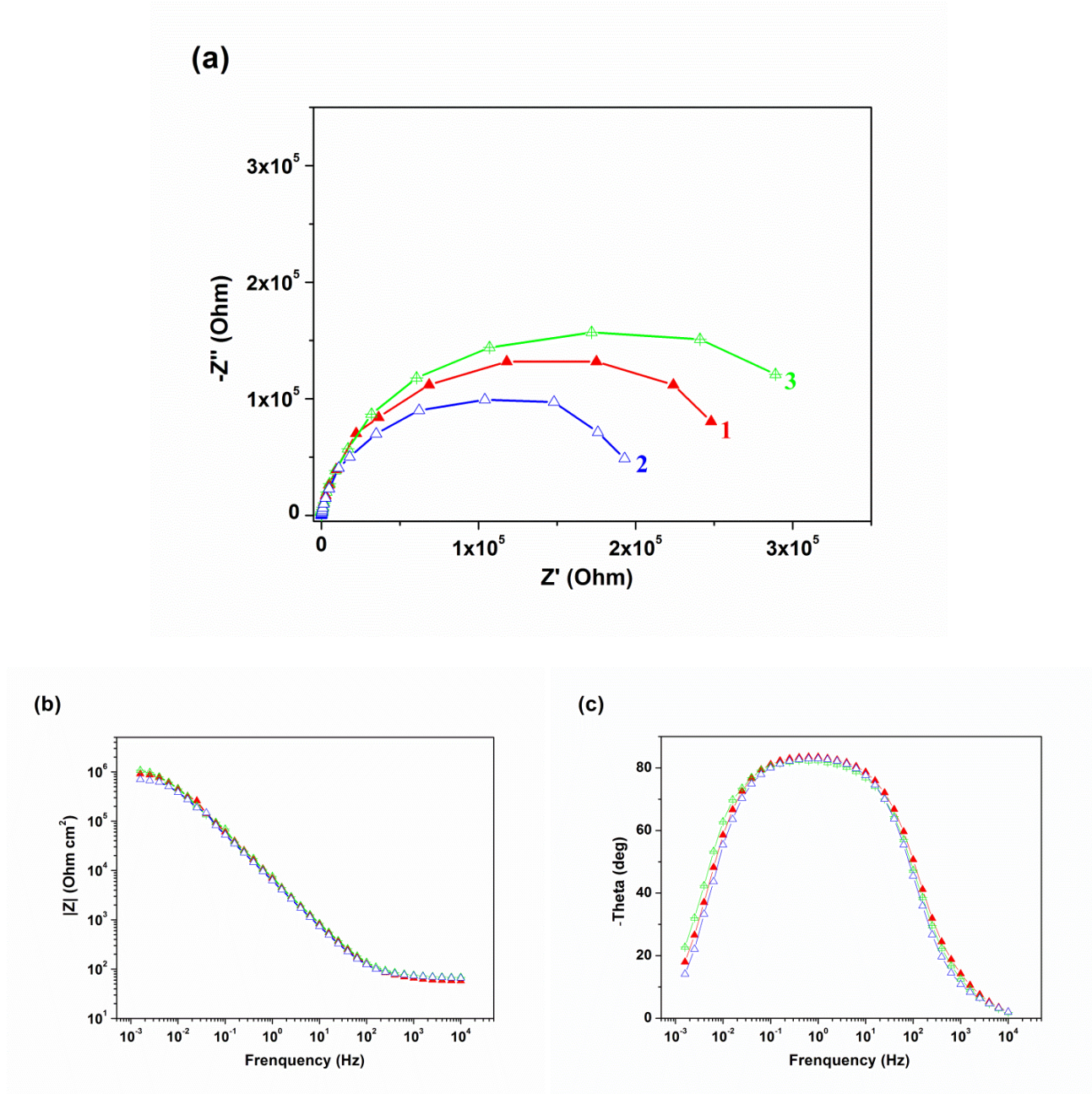
Figure 4-6 Comparison of Nyquist plots (a), Bode impedance plots (b) and Bode phase angle plots (c) for cp Ti before unidirectional sliding tests, measured with three different specimens at immersion time of 3 h before sliding in the PBS solution.
