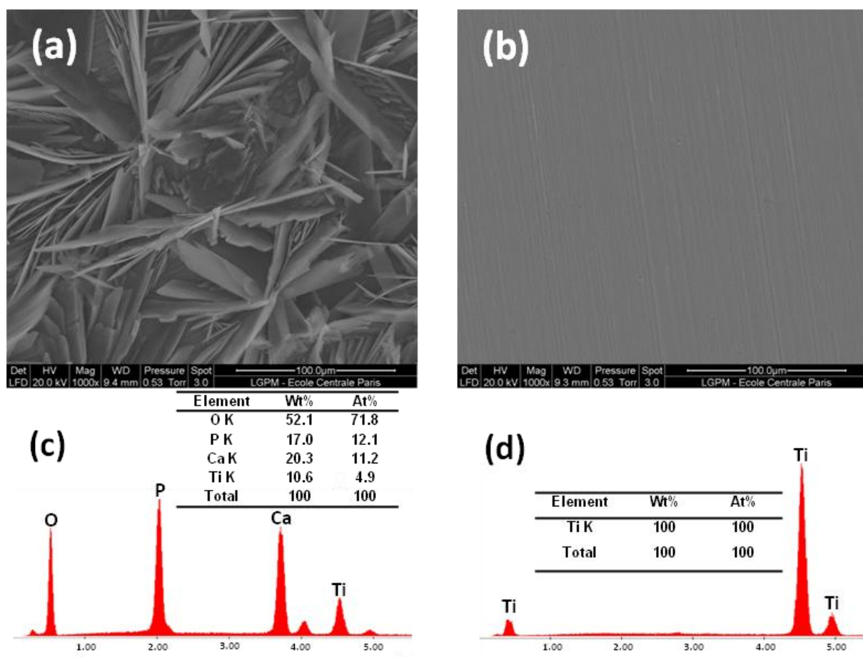
Figure 6-7 SEM images and EDS analysis of chemical composition of CaP bioactive film coated Ti (a, c) and untreated Ti (b, d).
