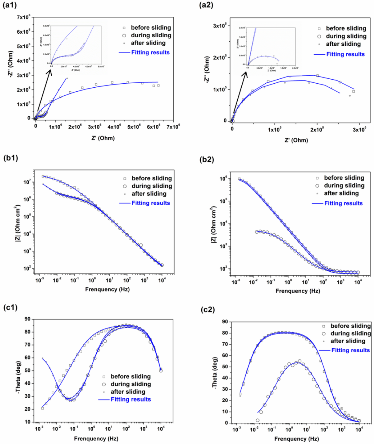
Figure 5-11 Nyquist plots (a), Bode impedance plots (b) and Bode phase angle plots (c) for TO Ti prepared at 650 °C for 48 h (1) and untreated Ti (2) measured before (square), during (ring) and after (star) continuous unidirectional sliding tests at F_n of 5 N in the PBS solution.
