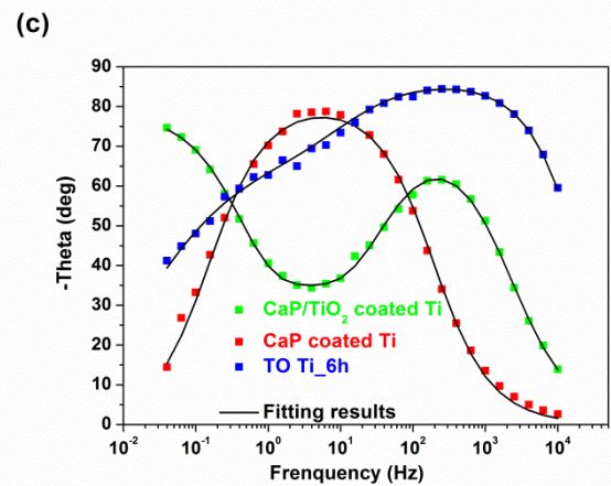
Figure 7-10 Nyquist plots (a), Bode impedance plots (b) and Bode phase angle plots (c) for CaP/TiO 2 bioceramic film coated Ti (green square), CaP bioactive film coated Ti (red square), TO Ti 6 h (blue square) during continuous unidirectional sliding tests performed at F_n of 500 mN.
