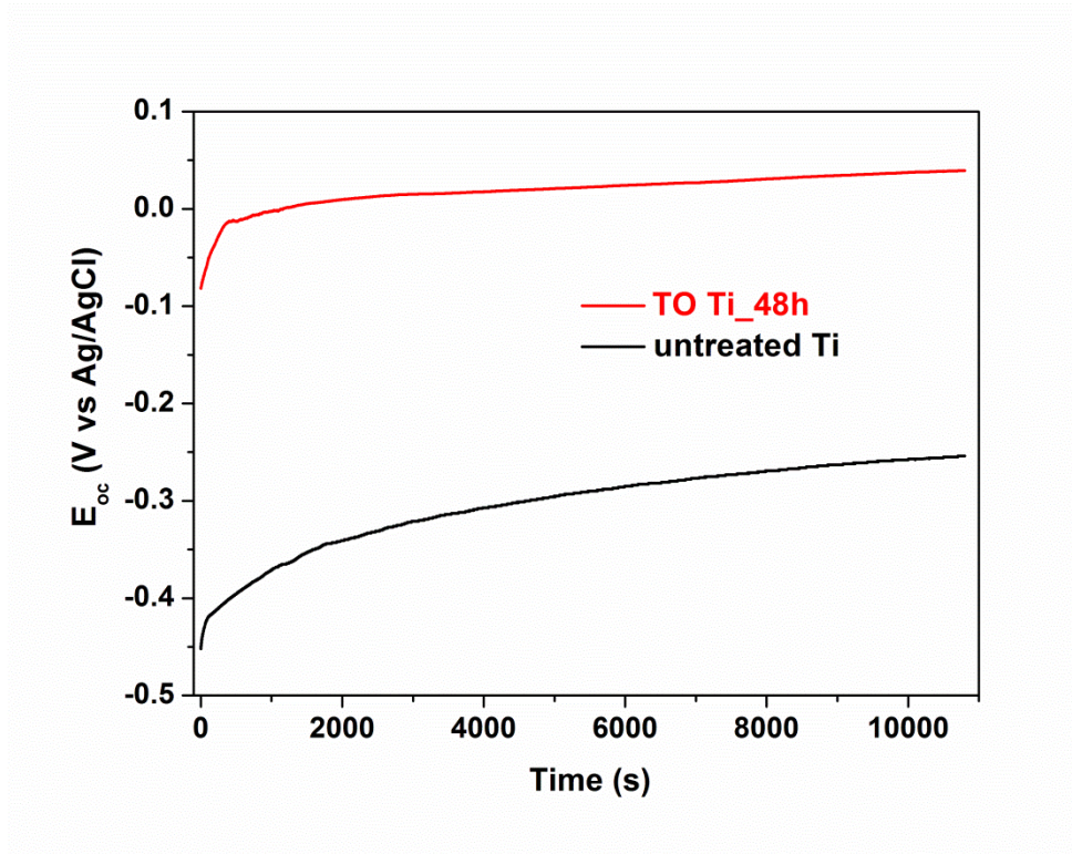
Figure 5-5 OCP evolution of TO Ti prepared at 650 °C for 48 h (red line) and untreated Ti (black line) in the PBS solution.
