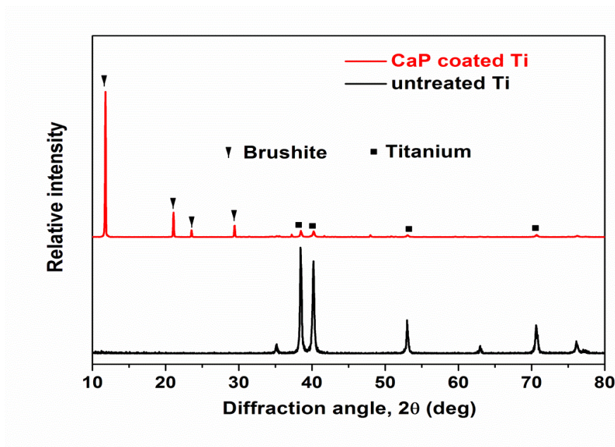
Figure 6-6 XRD patterns of CaP bioactive film coated Ti (red line) and untreated Ti (black line).
