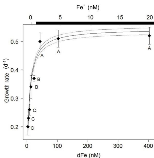
Figure 1. Growth rate of C. watsonii related to dFe and Fe' concentrations. Error bars represent standard deviation; different letters correspond to statistically different means ( p < 0.05 ) and the black bar indicates the region of expected Fe hydroxide precipitation. The Monod regression, performed with dFe concentrations, is represented by the black line and standard deviation of regression by dotted lines.
