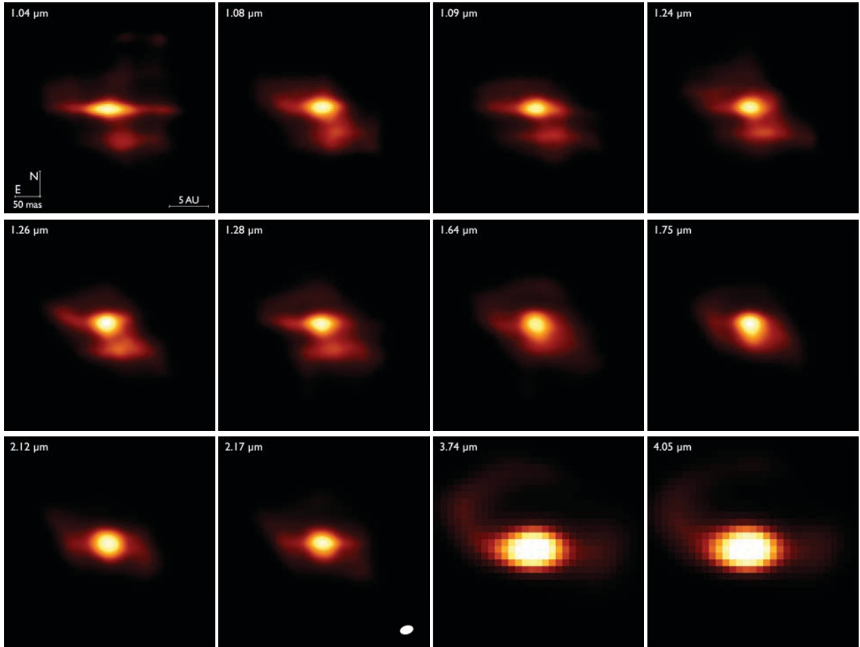
Fig. 4. Deconvolved images of L 2 Pup using a uniform, 80-step Lucy deconvolution. Orientation, field of view and color scale are the same as in Fig. 2. The white ellipse represented in the 2.17 μm panel corresponds to the star model derived from the VINCI data (Sect. 2.2.2).
