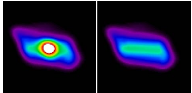
Fig. 6. Deconvolved image of L 2 Pup at 2.17 μm (left) and contribution from the disk alone (right). The field of view is 1.33''.
