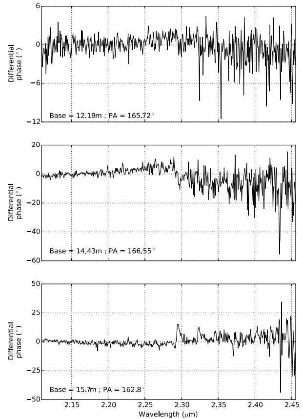
Fig. 9. Differential phases of our datasets below 55 arcsec -1 (sampling the first and second lobe of the visibility function). We selected measurements not sampling a node of the visibility function.
