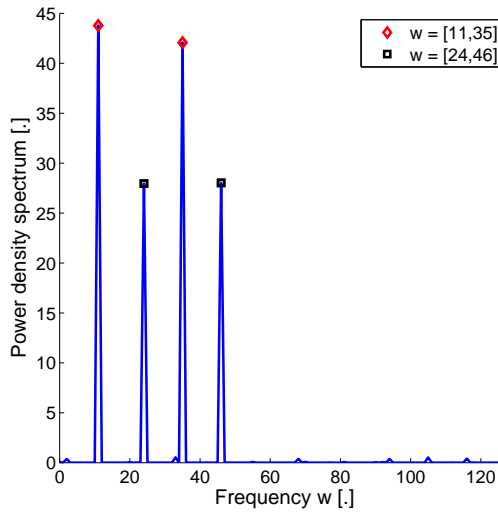
Figure B.2: Power spectrum of Y for FAST
