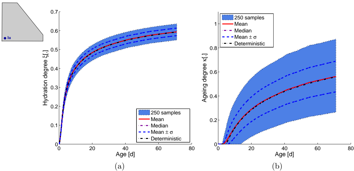
Figure 6.8: Hydration and ageing degrees evolution on “point lu”: a) Construction during winter; b) Construction during summer.
