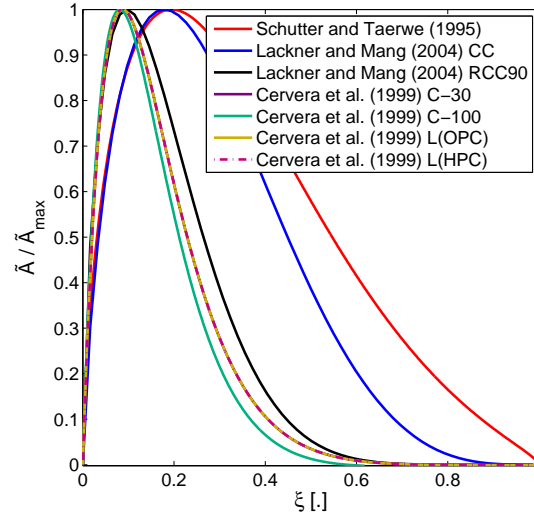
Figure 2.12: Normalized chemical affinity evolution, three different models
