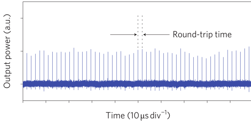
Figure 1.17: Observation of an isolated CS. The delay between subsequent pulses matches the 1.85\text{-}\mu\text{s} cavity round-trip time, and confirms the presence inside the cavity of a single persistent pulse circulating repeatedly, only sustained by the c.w. driving beam [Leo 2010].
