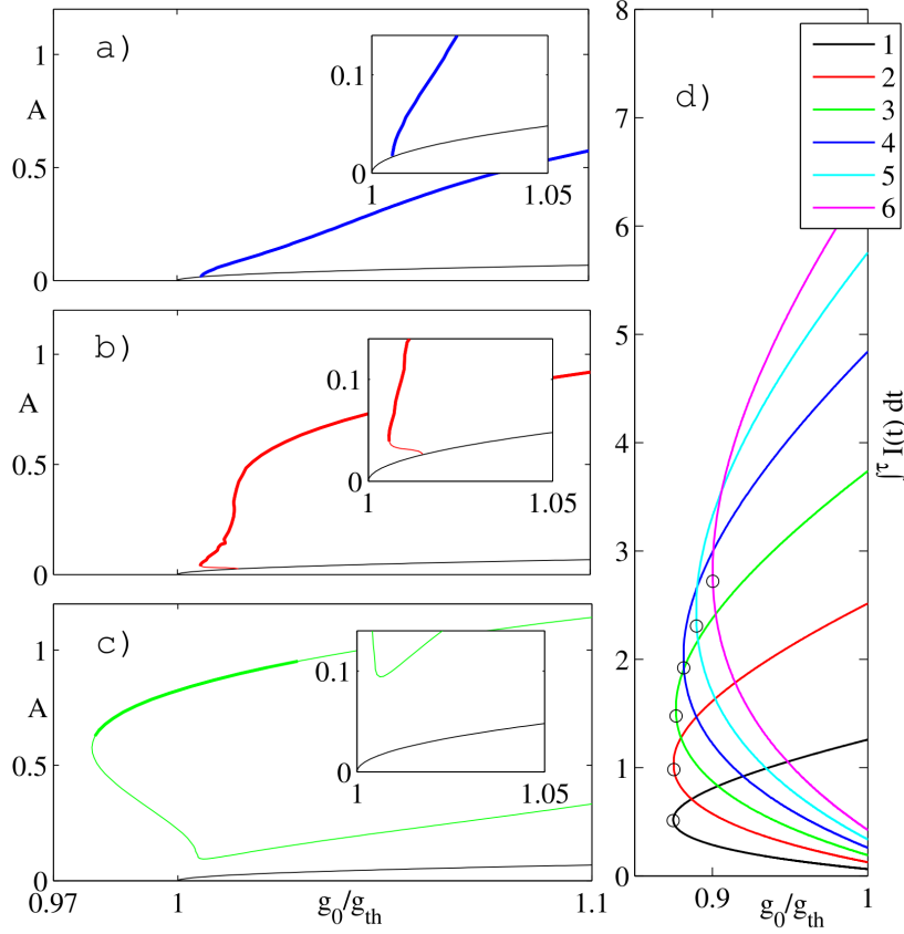
Figure 3.13: Panels (a-c) depict the bifurcation scenario as a function of the gain for different values of the delay: a) \tau=1.2\Gamma^{-1} , b) \tau=2\Gamma^{-1} and c) \tau=4\Gamma^{-1} . For short delays, the PML periodic solution (in colors) appears as a supercritical Andronov- Hopf bifurcation of the dominant c.w. mode (thin black line). The stability of the PML solution is indicated by thick lines while the stability of the c.w. mode is omitted. Panel d) shows, for \tau=16\Gamma^{-1} , the folding of the several PML solutions having a different number of equally separated pulses per round-trip while the folding point g_{sn} is represented by a circle.
