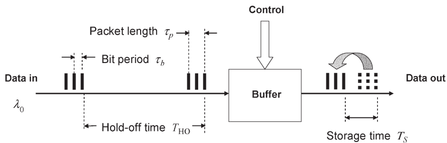
Figure 1.11: Principle of a buffer [Tucker 2005].
