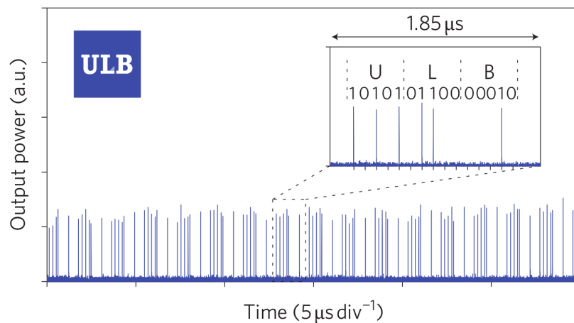
Figure 1.18: The acronym of the ULB institution stored all-optically with temporal CS. ULB (Université Libre de Bruxelles) is encoded as a 15-bit data stream in the passive fibre cavity. Each letter is represented with five bits by its ordinal position in the alphabet (U=21, L=12, B=2) [Leo 2010].
