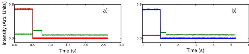
Figure 4.6: LP-X (red trace), LP-Y (blue trace) polarization intensities and PSF signal injected into the VCSEL (green trace), for clarity green trace is shifted vertically of 0.1 units. T = 30^\circ\text{C} , J = 2.9\text{mA} .
