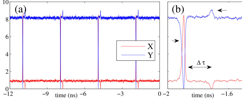
Figure 4.32: Theoretical temporal trace for a single vectorial LS (a) created by perturbing the phase of PSF and zoom on the pulse detail (b): the antiphase dip is followed by a small inverted kink after a time delay \Delta\tau corresponding to the re-injection of Y into X after a longer time \tau_r . Other exponentially decreasing replica of this secondary kink (not visible) follow at time intervals n\Delta\tau .
