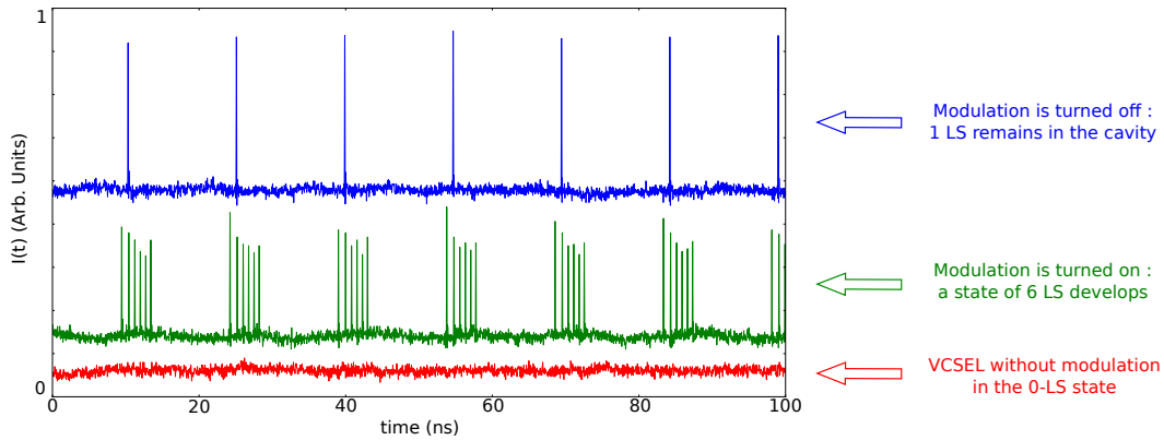
Figure 3.9: Time traces showing the experimental process for LS generation via current modulation. First the laser is in the 0-LS state without modulation (red), J = 215 mA. Second, modulation is applied with -30 dBm amplitude, 6 LS suddenly arise on top of the modulation (green). When we switch-off current modulation, only 1 LS remains in the cavity.
