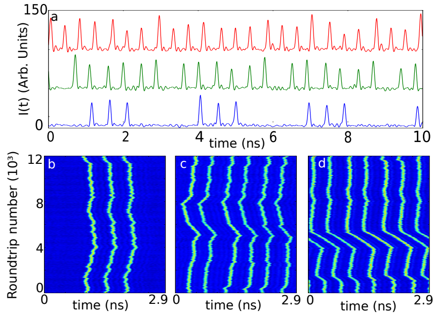
Figure 4.26: Panel a): (blue) LP-X time trace showing a three-peaks molecule, (green) a six-peaks molecule, (red) a seven-peaks molecule. The two last traces have been shifted vertically for clarity. Panel b): Space-time like diagram for the 3-peaks molecule, panel c) for the 6-peaks molecules, panel d) for the 7-peaks molecule.
