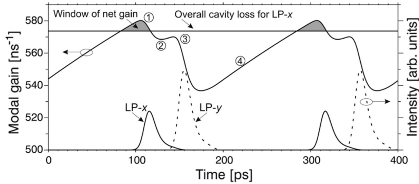
Figure 1.31: Temporal evolution of the gain and overall-cavity loss for X. The loss for Y is out of scale. The labels (1) and (3) depict the positions of the gain depletions, while (2) and (4) stand for gain recovery stages.
