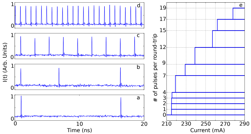
Figure 3.2: Panels a), b), c) and d): coexisting time output traces ( J = 290 mA). Panel e): experimentally obtained bifurcation diagram for the number of pulses per round-trip. The stability of each solution is indicated by the solid horizontal lines.
