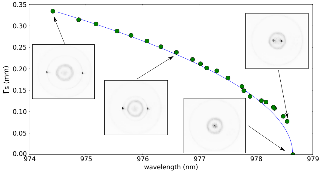
Figure 2.7: Off-axis position of a single spot in the far-field profile as a function of the spectral emission peak of the VCSEL. Far-field profiles are shown for a few points in the graph. VCSEL emission is in the mode-locking regime for all points of the graph while the one at the highest wavelength, where a single on-axis spot appears in the far-field profile, corresponds to very irregular dynamics. VCSEL is biased at 700 mA. The transverse wave vector is selected by laterally shifting the RSAM along the back focal plane of its collimating lens. The large size of the RSAM section ( 4 \times 4 \text{ mm}^2 ) with respect to the far-field size (0.7 mm at most) renders this operation feasible. The blue line has been obtained plotting r_s = \frac{\lambda_0 f}{2\pi} \sqrt{\lambda^{-2} - \lambda_0^{-2}} , with \lambda_0 = 978.65 \text{ nm} and f = 8 \text{ mm} .
