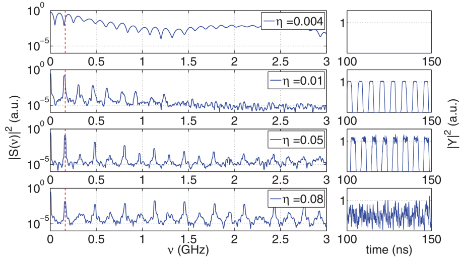
Figure 4.16: Power spectra (left) and temporal traces (right) of the intensity of the LP-Y component of the VCSEL for increasing values of the PSF rate \eta with \mu = 2 and \beta = 0.3 . For too small values of \eta , the system operates on the stable LP-X polarization, and there is an optimal feedback value \eta \approx 0.01 above which the regularity of the square-waves deteriorates. The vertical red line in the spectra marks the frequency spacing of the external cavity modes.
