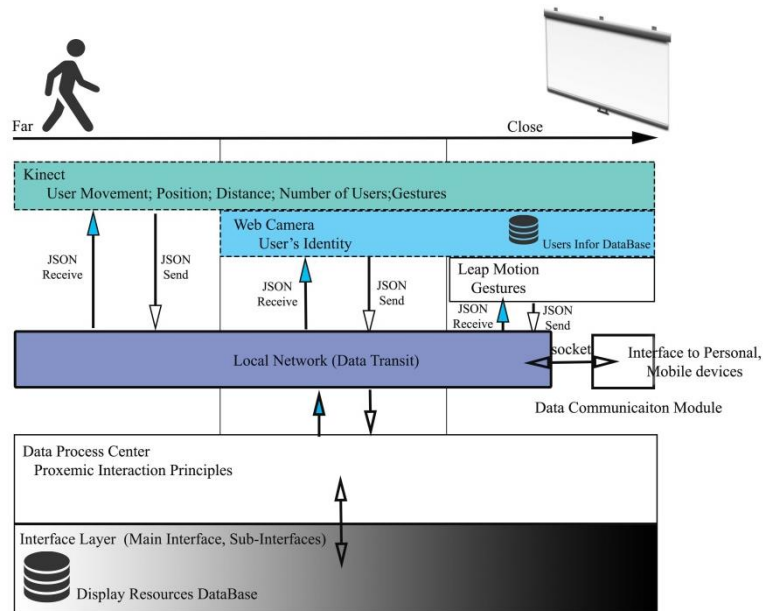
Figure 4.7 Modularized System Architectures
