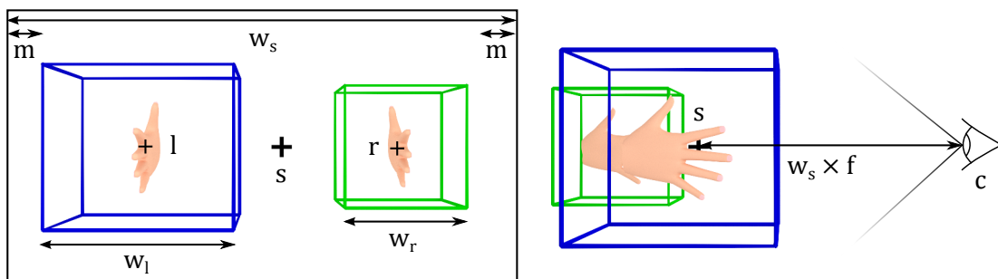
Figure 3.4 – Computation of the camera position for viewport adaptation. (left) View of the two bubbles from the computed camera position. The points l , r , s are the centers of the left bubble, right bubble and scene, and w_l , w_r , w_s their respective widths. (right) Side view showing the camera position \mathbf{c} with respect to the center of the scene.
