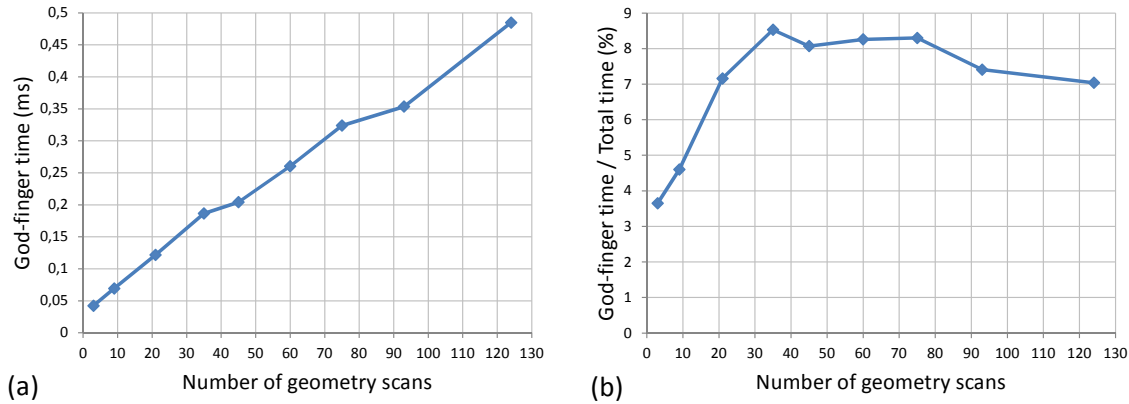
Figure 4.14 – Scaling of the computation time of the god-finger algorithm with the number of geometry scans. (a) Absolute time. (b) Relative time to the total simulation step.
