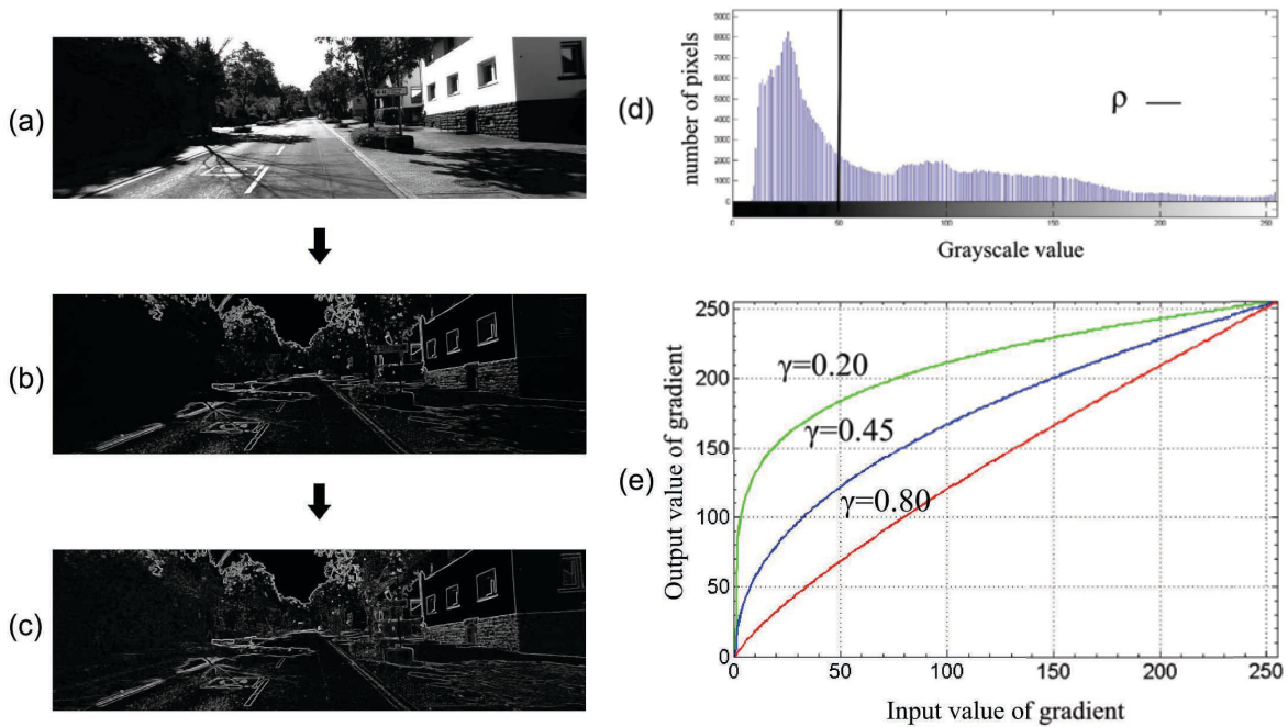
Figure 3.3 - Enhancing the contrast of higher frequency in shadow areas. (a) Original image, (b) gradient image, (c) the gradient image with shadow area enhanced, (d) the division of the two groups based on the image histogram and (e) presents different output results ranging the parameter \gamma .
