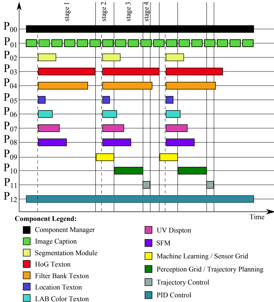
Figure 5.13 - Execution example of the designed multiprocessed pipeline.
