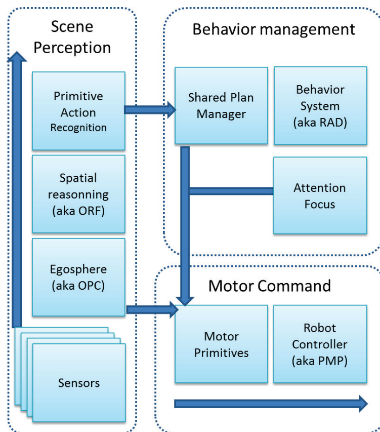
Figure 39: Status of the EFAA architecture at the time of writing.
