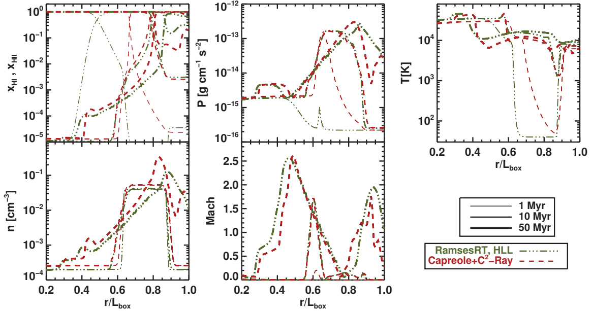
Figure 4.25: IIO9 test 7. Profiles along the x-axis of symmetry through the center of the box, at 1, 10 and 50 Myr for the RamsesRT and Capreole+C 2 -Ray results. Clockwise from top left: Ionization fractions, pressure, temperature, Mach number, atom number density.
