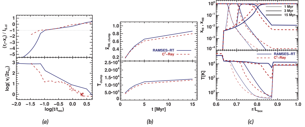
Figure 4.14: IIO6 test 3: RamsesRT+HLL versus C 2 -Ray comparison. (a) Evolution of the position and speed of the I-front along the x-axis through the center of the box. The position plot (top) shows the x-position where x_{HII} = 0.5 , with respect to the center of the cloud, x_c = 5 kpc, in units of the Strömgren length inside the cloud, \ell_{S,cl} = 0.78 kpc. The dotted horizontal lines mark the edges of the cloud. The speed (bottom) is plotted in units of twice the isothermal sound speed in the cloud at T = 10^4 K, 2c_{s,l}(10^4 \text{ K}) = 2.35 \cdot 10^6 cm/s. (b) Evolution of the average ionized fraction (top) and temperature (bottom) inside the dense cloud. (c) Profiles along the x-axis through the box center of the ionization state (top) and temperature (bottom), at 1, 3 and 15 Myr.
