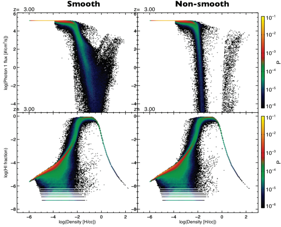
Figure 5.14: Smooth RT: Comparison of photon fluxes ( top ) and H I fractions ( bottom ) at redshift 3 in low resolution equivalents of the H I simulation that are identical save that the left one uses smooth RT and the right one does not.
