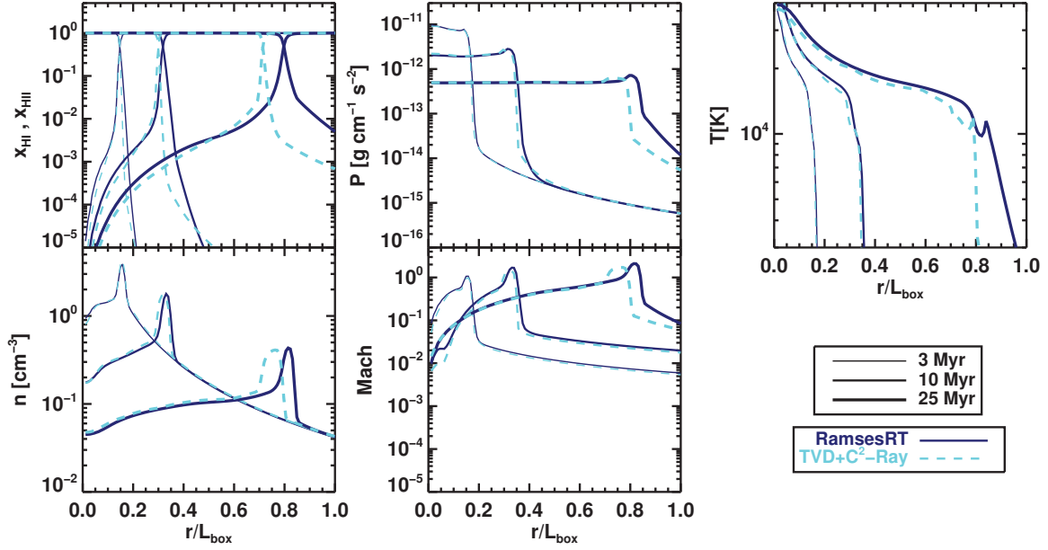
Figure 4.22: I109 test 6. Radial profiles at 3, 10 and 25 Myrs, compared to the TVD+C 2 -Ray results. Clockwise from top left: ionization fractions, pressure, temperature, Mach number, atom number density.
