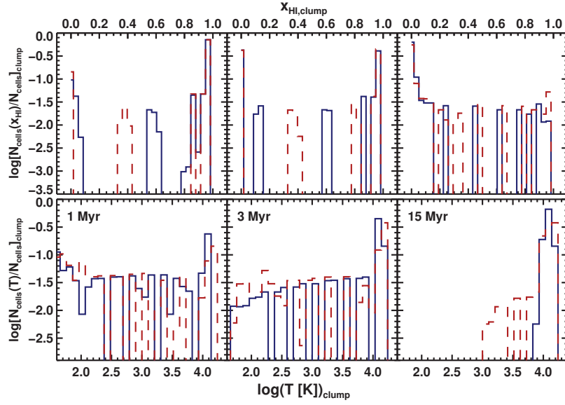
Figure 4.15: II06 test 3: RamsesRT+HLL versus C^2 -Ray comparison. Histograms of neutral fraction (top row) and temperature (bottom) inside the dense cloud at 1, 3 and 15 Myr (from left to right).
