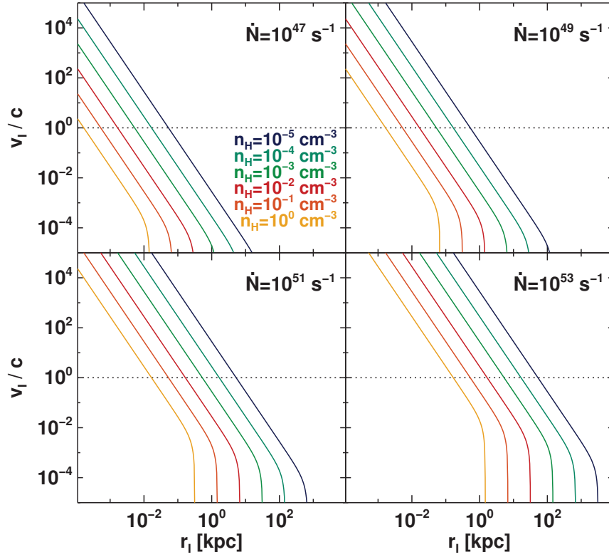
Figure B.1: Idealized I-front speeds, in units of the light speed, for a range of densities and luminosities. The speed of the I-front, v_I , is calculated from the Strömgren sphere model. Each of the four plots represents a source luminosity. Each of the solid colored lines represents a gas density. Horizontal dotted lines represent the light speed.
