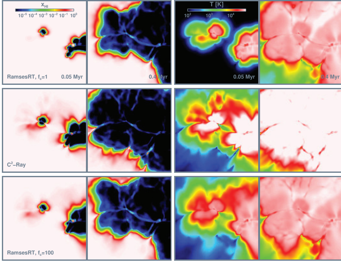
Figure 4.16: IIO6 test 4. Maps showing slices at i_z=64/128 of the neutral fraction and temperature at times 0.05 Myr and 0.4 Myr. Top row shows RamsesRT results with physical light speed. The middle row shows the C^2 -Ray results (infinite light speed). The bottom row shows the RamsesRT results with one hundred times the physical light speed.
