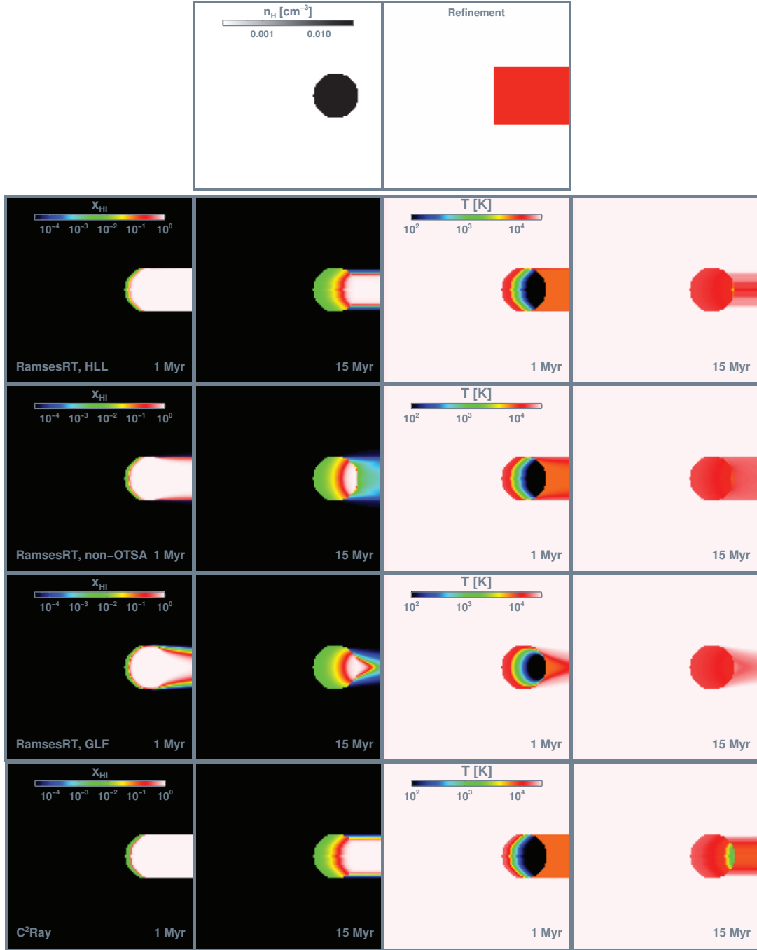
Figure 4.13: IIO6 test 3. Maps showing slices at i_z=64/128 . The top row maps show the (constant) density field (left) and the static refinement (right) applied in the RamsesRT run, where white/red marks effective resolution of 64^3/128^3 cells. The second row shows the RamsesRT+HLL results in terms of neutral fraction (left) and temperature (right) at 1 and 15 Myr. The third row Shows the RamsesRT+HLL results without the on-the-spot approximation. The fourth row shows the RamsesRT+GLF results. The bottom row shows the C 2 -Ray results for comparison.
