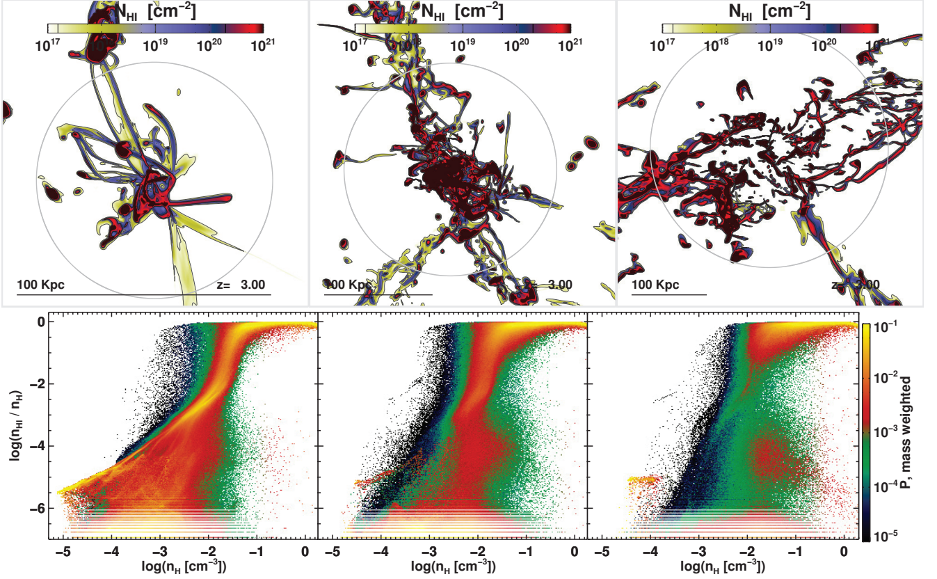
Figure 4. Neutral hydrogen at redshift 3 (H1, H2, H3 halos from left to right). Top row: Maps of projected H I column density. Contours correspond to the lower limits for DLAs ( N_{\text{H}} = 2 \times 10^{20} \text{ cm}^{-2} ), SLLSs ( 10^{19} \text{ cm}^{-2} ) and LLSs ( 1.6 \times 10^{17} \text{ cm}^{-2} ). Bottom row: Phase diagrams of neutral hydrogen fraction, x_{\text{HI}} \equiv n_{\text{HI}}/n_{\text{H}} , versus density. The color scale represents mass-weighted probability per x_{\text{HI}} - n_{\text{H}} bin over the plotted x_{\text{HI}} range. The quantization-like horizontal lines at the bottom of all diagrams are due to numerical precision of the cell variable x_{\text{HI}} in RamsesRT , which is roughly seven digits.
