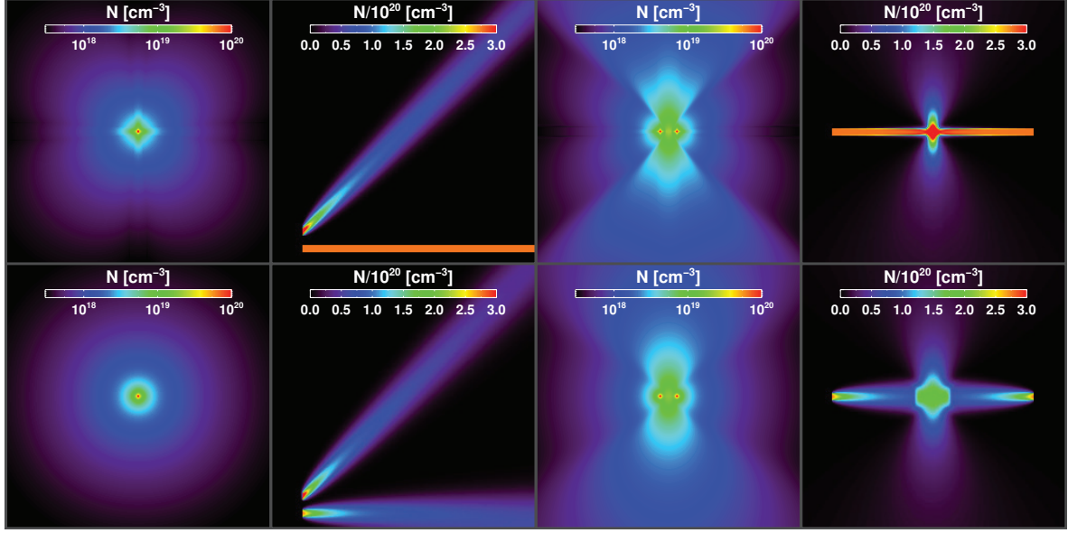
Figure 3.1: Comparison of radiative transport in 2D RamsesRT runs (no gas interaction) with the HLL ( top ) and GLF ( bottom ) flux functions. The box width is 1 kpc and 10^{50} photons \text{s}^{-1} are injected continuously for each source. The snapshots are taken after a few light crossing times. Far left frames show single isotropic point sources. Middle left frames show attempts at creating horizontal and diagonal beams. Photons are injected into a vertical buffer of 7 cells with a unity reduced flux (i.e. no isotropic component). Middle right frames show two isotropic point sources and how the photons act between them. Far right frames show two beams of opposing directions and how a perpendicular radiation source forms where they meet.
