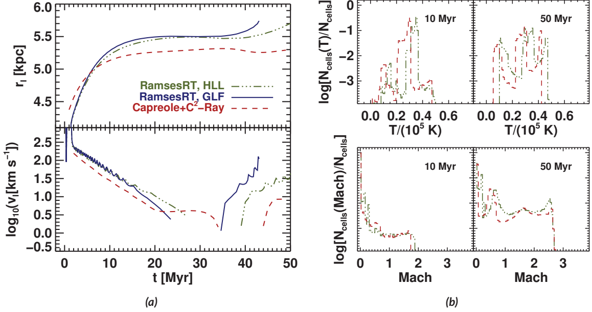
Figure 4.24: IIO9 test 7. (a) Time evolution of the position (top) and speed (bottom) of the ionization front along the x-axis of symmetry through the center of the box. (b) Histograms of the gas temperature (upper panel) and flow Mach number (lower panel) at 10 and 50 Myr for RamsesRT and Capreole+C 2 -Ray.
