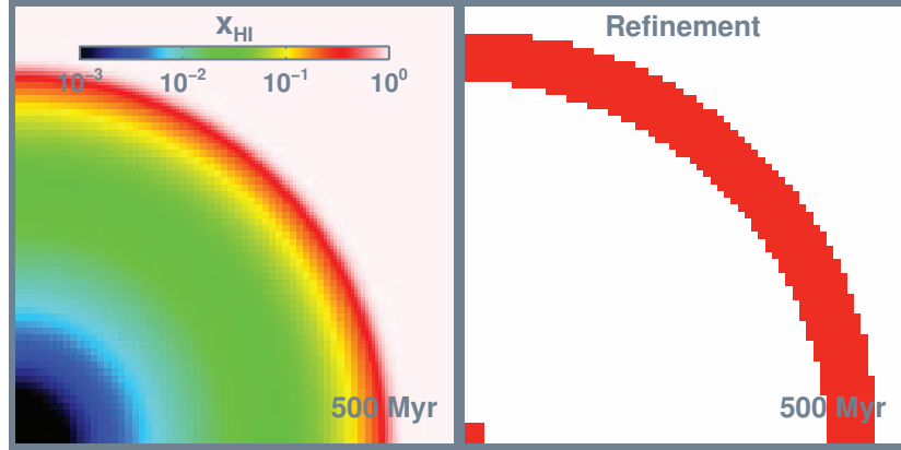
Figure 4.7: II06 test 1. Maps showing the neutral fraction ( left ) and grid refinement ( right ) in a box slice at i_z = 1/128 (first cell-slice out of 128), at 500 Myr. In the refinement map, white corresponds to the minimum effective resolution of 64^3 cells and red to the maximum effective resolution of 128^3 cells. As the map shows, the radiative source and the outer side of the I-front are refined on-the-fly during the experiment.
