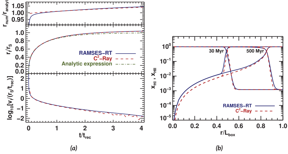
Figure 4.8: I/O6 test 1. (a) Evolution of the I-front position and velocity. Blue solid lines show our result, red dashed lines show the C 2 -Ray result and green dot-dashed lines show the analytic expression. (b) Spherically averaged profiles for neutral fractions x_{\text{HI}} and ionized fractions x_{\text{HII}} at 30 and 500 Myr versus radius (in units of the box width L_{\text{box}} ).
