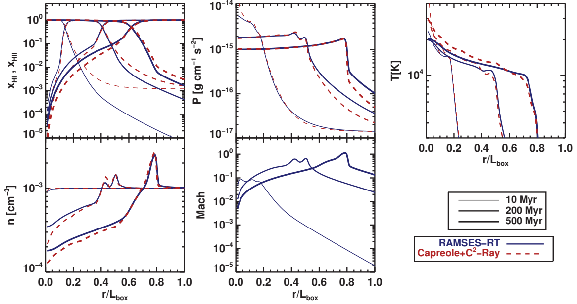
Figure 4.19: IIO9 test 5. Radial profiles at 10, 200 and 500 Myrs, compared to the Capreole+C 2 -Ray results. Clockwise from top left: Ionization fractions, pressure, temperature, Mach number, atom number density.
