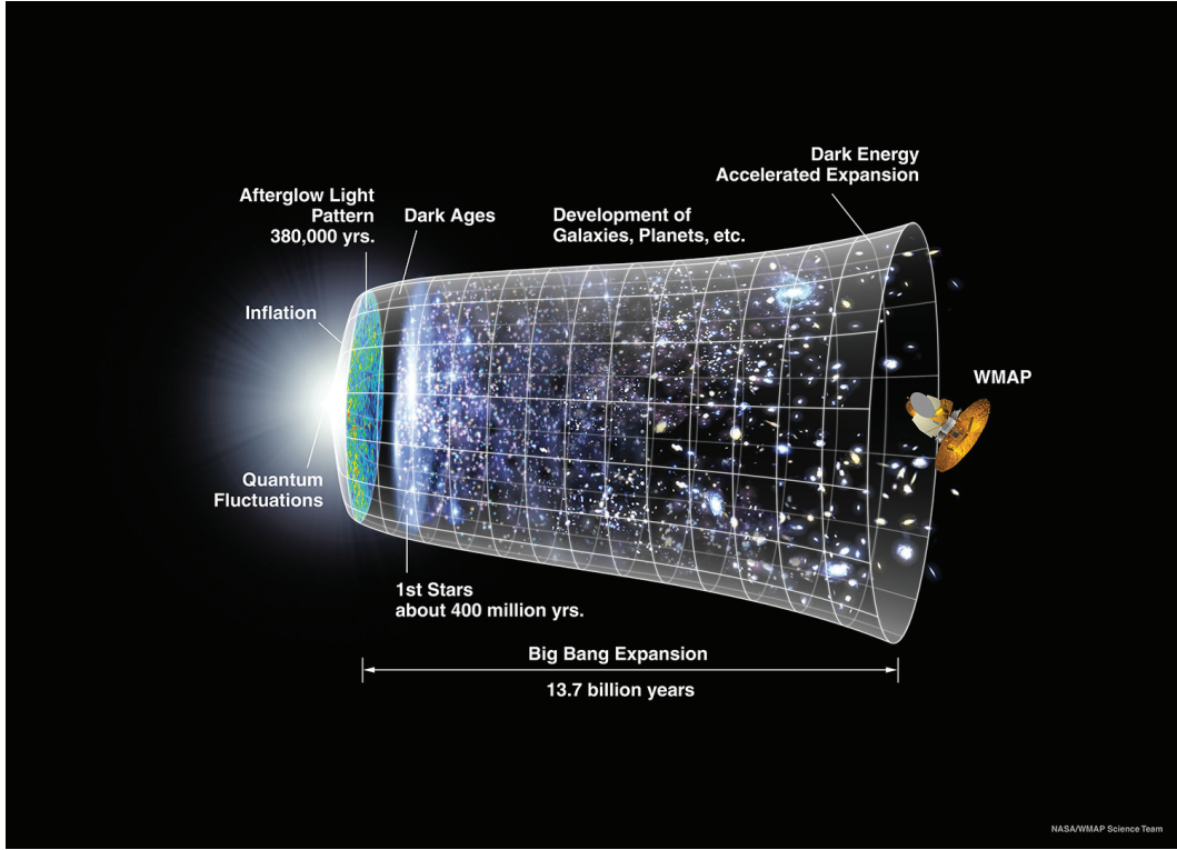
Figure 1.2: Timeline of the Universe, with the WMAP satellite looking through almost the whole history so far at the CMB. Credit: NASA / WMAP Science Team.
