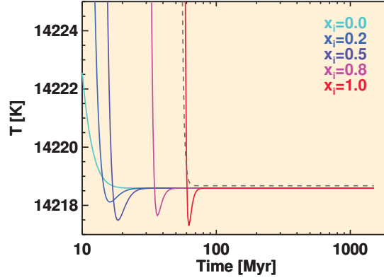
Figure 4.5: Close-up of temperature convergence, for the UV inclusive test with initial temperature T \approx 10^5 K and n_H = 10^{-2} \text{ cm}^{-3}
