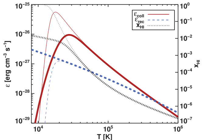
Figure 6. Ly \alpha emissivity of gas at number density n_{\text{H}} = 3 \times 10^{-2} \text{ cm}^{-3} , which is close to the lower limit for accretion streams in our simulations. Thick curves show gas exposed to a UV field with \Gamma = 6.1 \times 10^{-13} \text{ s}^{-1} , corresponding to redshift 3. Thin curves show UV shielded gas ( \Gamma = 0 \text{ s}^{-1} ). Blue dashed curves show recombinative Ly \alpha emissivity, red solid curves show collisional Ly \alpha emissivity and black dotted curves show the approximate neutral hydrogen fraction in the gas, assuming equilibrium between photoionization, collisional ionization and recombinations.
