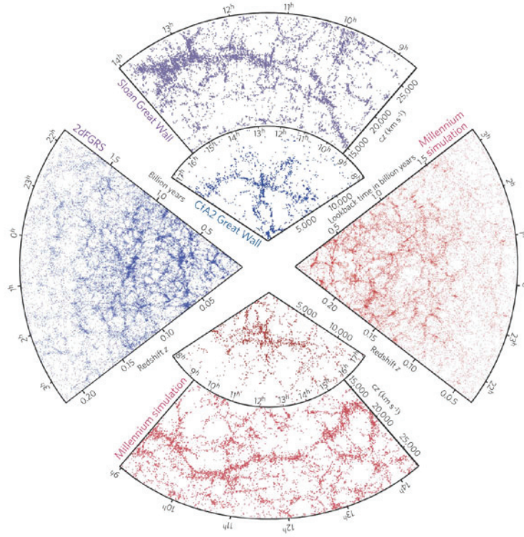
Figure 1.3: Simulations versus observations of the large scale structure of the universe. The left and top wedges show results from sky-surveys of our neighbourhood, with each dot representing a galaxy. The bottom and right wedges show mock observations of the Millennium cosmological simulation at z = 0 with the same depths and fields of view as the real observations. Note how galaxies grow more diffuse as we reach further out in redshift in the left wedge due to the extinction of light at large distances. Yet this is only at a fraction of the redshift of the reionization epoch; there is very little to see out there with current instruments. Credit: Springel et al. (2006).
