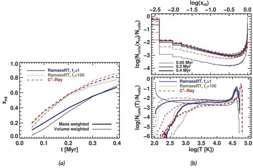
Figure 4.17: IIO6 test 4. (a) Time evolution of the mass weighted and volume weighted average ionized fractions. (b) Histograms of neutral fraction (top) and temperature (bottom).
