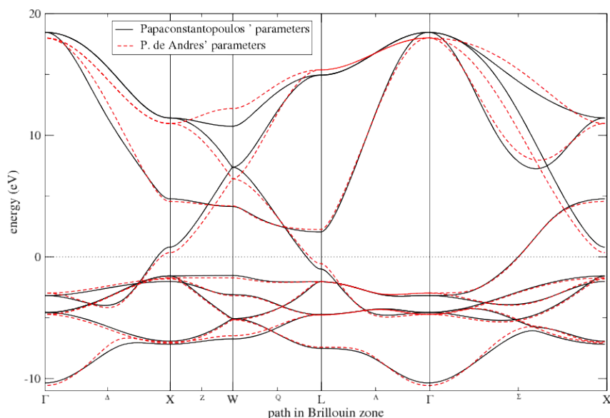
Figure V.1: Band structure of gold considering only nearest-neighbor hopping from BEEEM v2.1 input files (in dashed red lines) vs second nearest-neighbor hopping from [48] (in black lines). The two band structures are in quite good agreement, in particular around the Fermi level (RMS error < 70 meV for the sixth band).
