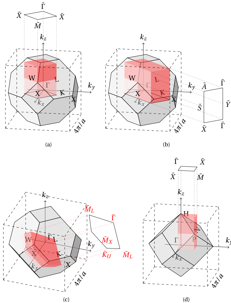
Figure V.5: 2-dimensional reduced projections of the 3D Brillouin zone of the FCC and BCC lattices. The current is calculated for each k -points within the red parallelepipeds, then summed in the direction of epitaxy. V.5(a), V.5(b) and V.5(c) are the projection of the reduced FCC Brillouin-zone respectively in the (001), (110) and (111) directions. V.5(d) is the projection of the reduced BCC Brillouin-zone (one quarter of the full Brillouin zone) in the (001) direction.
