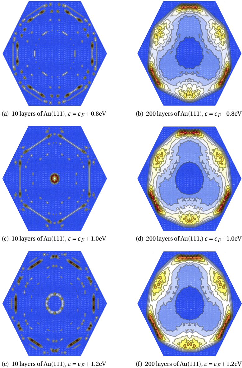
Figure V.19: Distribution of the elastic current with respect to the energy for 10 and 200 layers of Au(111). The current does not vary too much for thick slabs, so it is possible to project the available DOS from the Schottky barrier to the bias, that is not the case for thin structures.
