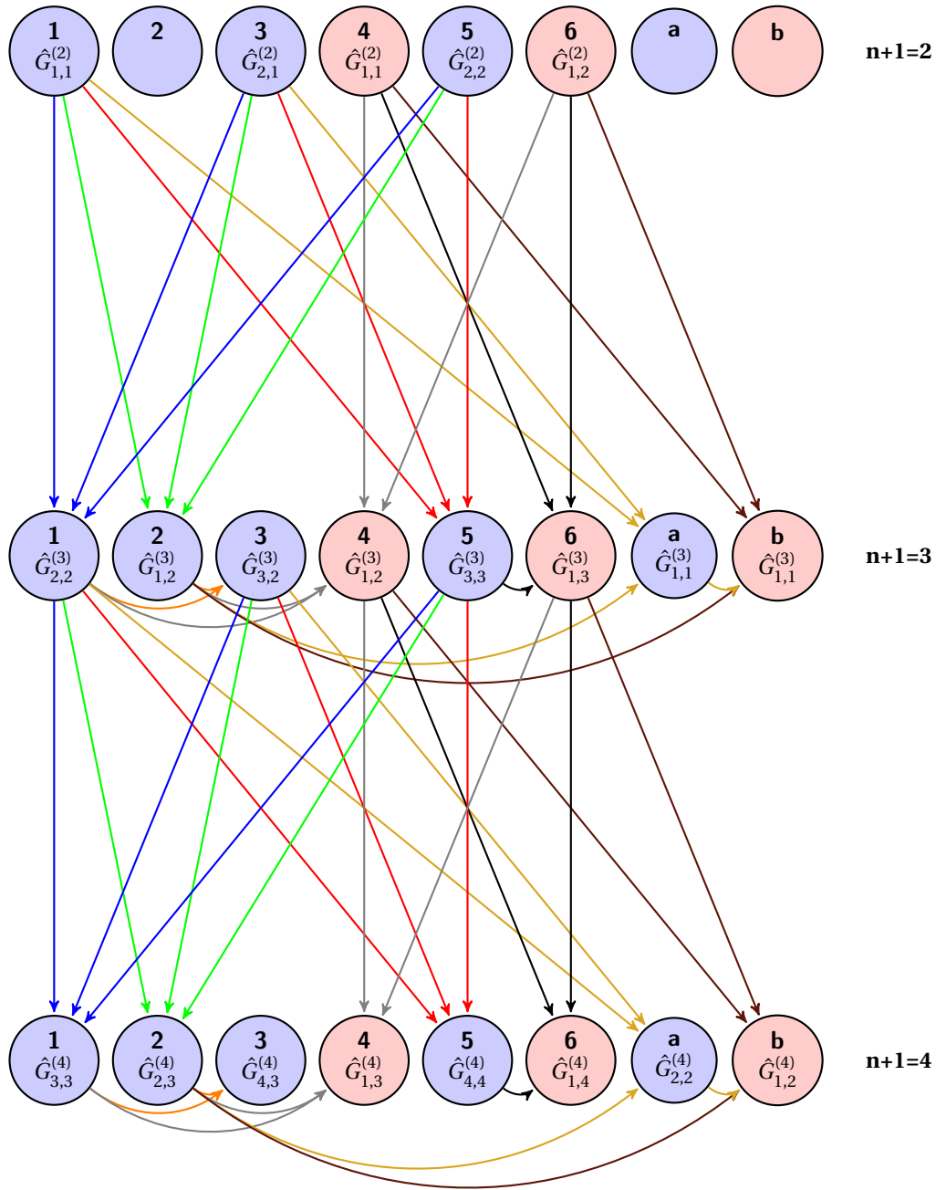
Figure III.7: Flow chart of the algorithm used to calculate the Green functions \hat{G}_{1,3}^{R,(4)} , \hat{G}_{1,2}^{R,(4)} and \hat{G}_{4,1}^{A,(4)} (pink circles). The label 1, 2, 3, 4, 5 and 6 are the same as those used in sec III.3.2.ii.h. This is also the same order used in the code to calculate the various Green functions. At the first iteration ( n=1 , we are looking for n+1=2 ), there is no next-nearest layers: \hat{G}_{i,j}^{(2)} is only expressed in term of \hat{G}_{i,j}^{(1)} . At the second iteration there are next-nearest-layer interactions, but still one degenerate case: step step 4 = step step 2 . At the third iteration, each Green function is different (at least all indexes are). Equations (III.152), (III.154) and (III.158) give the retarded Green function and the advanced Green function of the current formula (eq. (III.62)).
