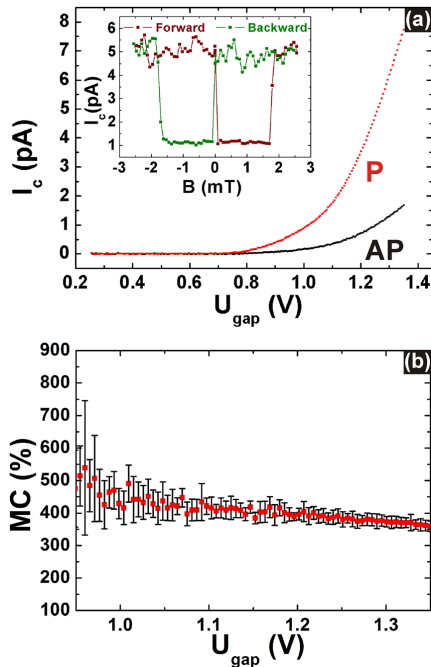
FIG. 1. (a) Ballistic electron spectroscopy curves I_c(U_{gap}) recorded on a Au(2.2 nm)/Fe(1 nm)/Au(2.6 nm)/Fe(1.2 nm)/GaAs(001) spin-valve in the parallel (red curve) and anti-parallel (black curve) magnetic configuration. Tunneling current was set to 20 nA. The inset displays a typical hysteresis loop I_c(B) recorded at 1.25 eV of electron energy. The in-plane magnetic field was applied along the [110] direction. (b) Calculated magnetocurrent versus electron energy deduced from Figure 1(a).
