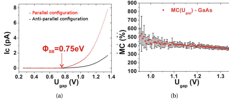
Figure II.9: (a) Room temperature Ballistic Electron Magnetic Spectroscopy performance on the Fe/Au/Fe/GaAs spinvalve, by M. Hervé et al. [25] and (b) resulting magneto-current. The MC seems to increase near the Schottky barrier.
