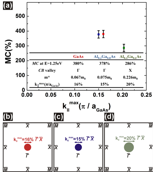
FIG. 3. (a) Evolution of the magnetocurrent amplitude at 1.25 eV versus maximum aperture in the semiconductor collimator for three Au(2.2 nm)/Fe(0.7–1.7 nm)/Au(2.6 nm)/Fe(1.2 nm)/Al x Ga 1-x As(25 nm)/GaAs(001) spin-valves with various aluminium contents x = 0, 0.2, 0.4 . The inset table gives for the three samples the CB minimum probed close to the Schottky barrier, the corresponding effective mass m^* , and collimator aperture k_{||}^{\max} calculated at 1.25 eV. Sketch of the collimator aperture at 1.25 eV in the projected semiconductor 2D Brillouin zone of Al x Ga 1-x As for x = 0 (b), x = 0.2 (c), and x = 0.4 (d).
