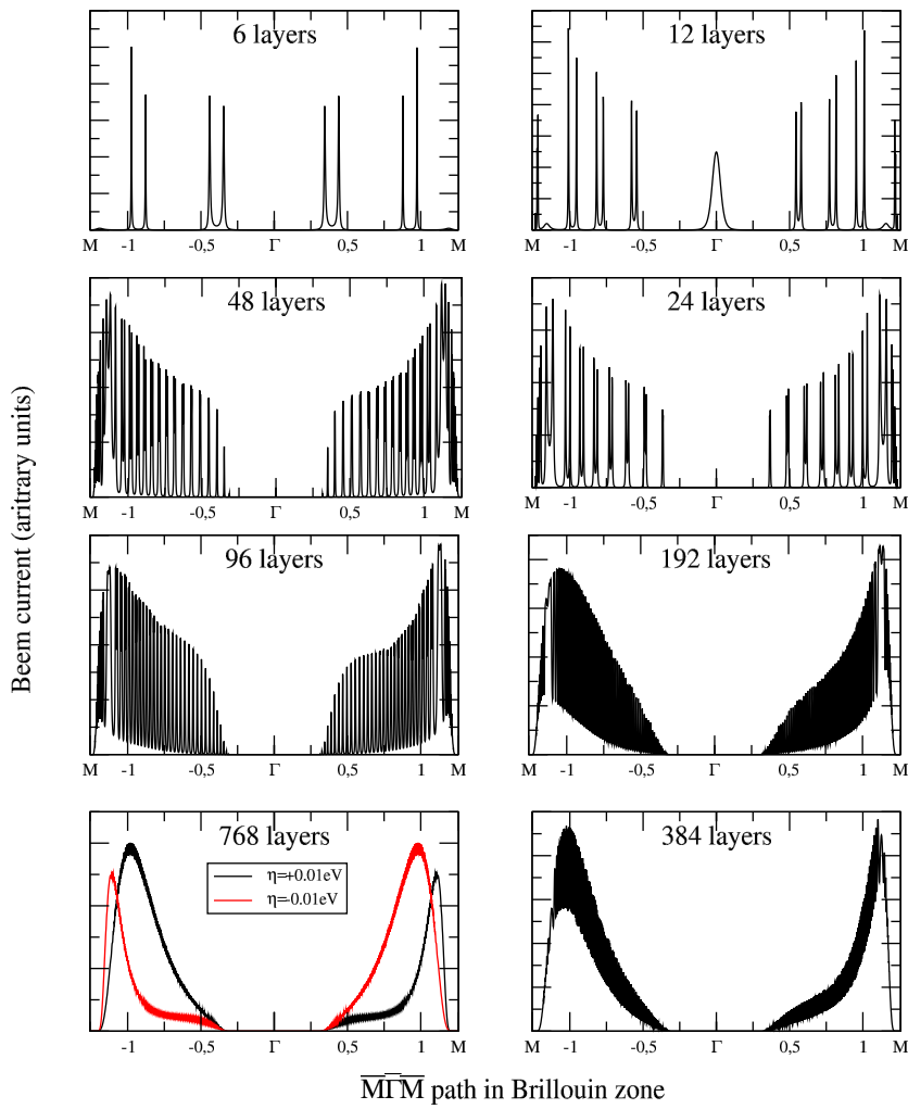
Figure V.13: Effect of the number of layers on the current profile, for \eta = 0.01\text{eV} . Above 384 layers, the 6-fold symmetry is lost, and the results converged to the equilibrium approach as found in Ref. [51] by P. de Andres and F. Flores group. The red curve obtained by taking a negative \eta is a check that by exchanging the retarded by the advanced GF, one finds the symmetric result.
