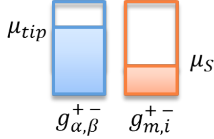
Figure III.3: The Keldysh Green functions for the uncoupled system ( i.e. for the tip alone and for the sample alone) are linked to the chemical potentials as shown in Eq. (III.42).
