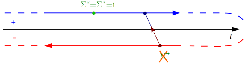
Figure III.2: The perturbation induced by the STM tip is instantaneous.
