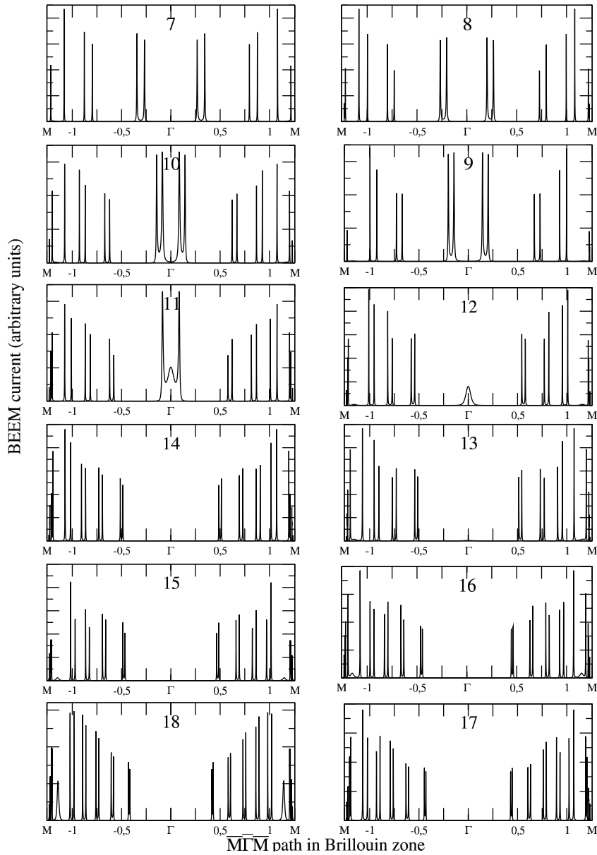
Figure V.14: Evolution of the BEEM current along \bar{M}\bar{\Gamma}\bar{M} with respect to the number of layers (from 7 to 18 layers) with \eta = 5\text{meV} . A peak at \vec{k}_{\parallel} = 0 appears for 10 layers, reaches its maximum for 11 layers and disappears after 12 layers.
