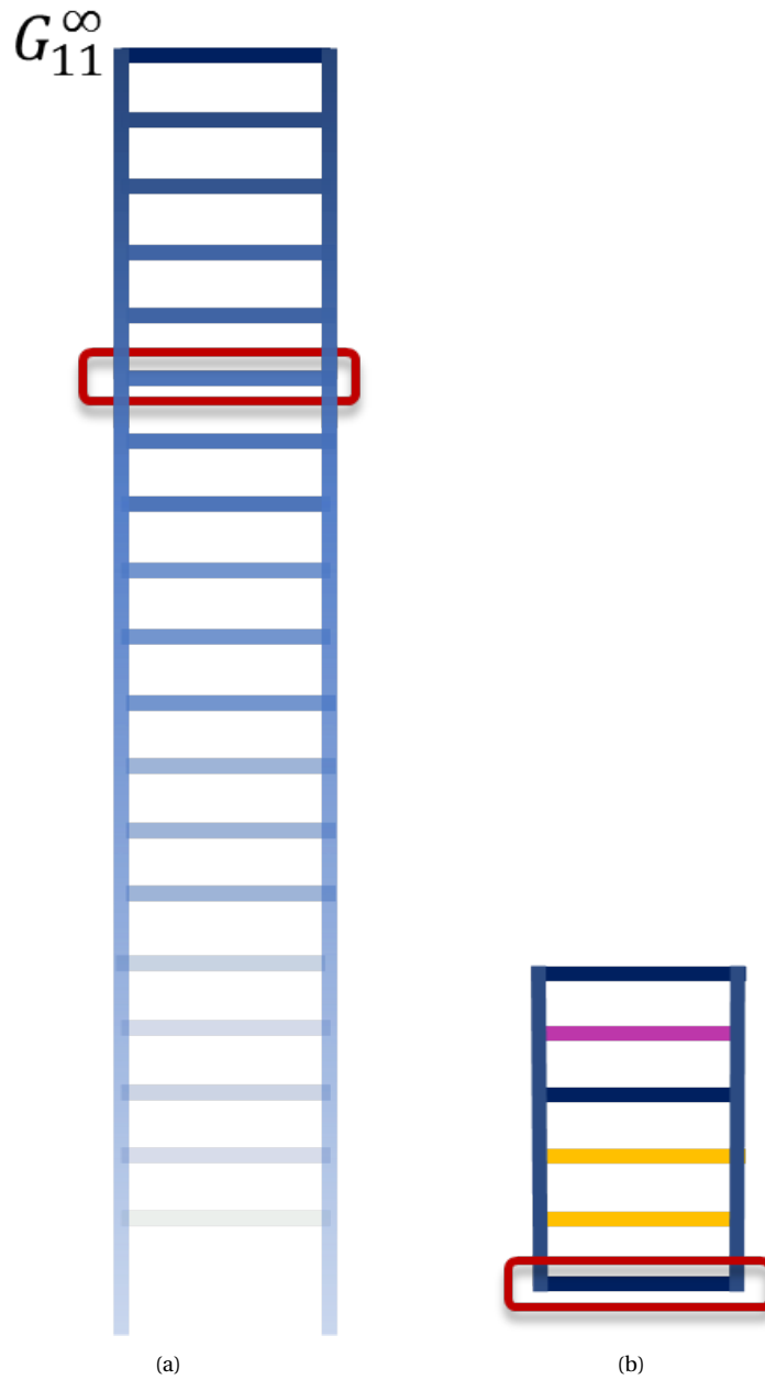
Figure III.4: Semi-infinite vs finite procedures. (a) BEEM v2.1 [52] uses the decimation procedure combined with a transfer-matrix approach in order to calculate the elastic current inside a semi-infinite slab that is, by construction, layer periodic. (b) Calculate Green functions through a layer-by-layer procedure allows to describe thin heterostructures.
