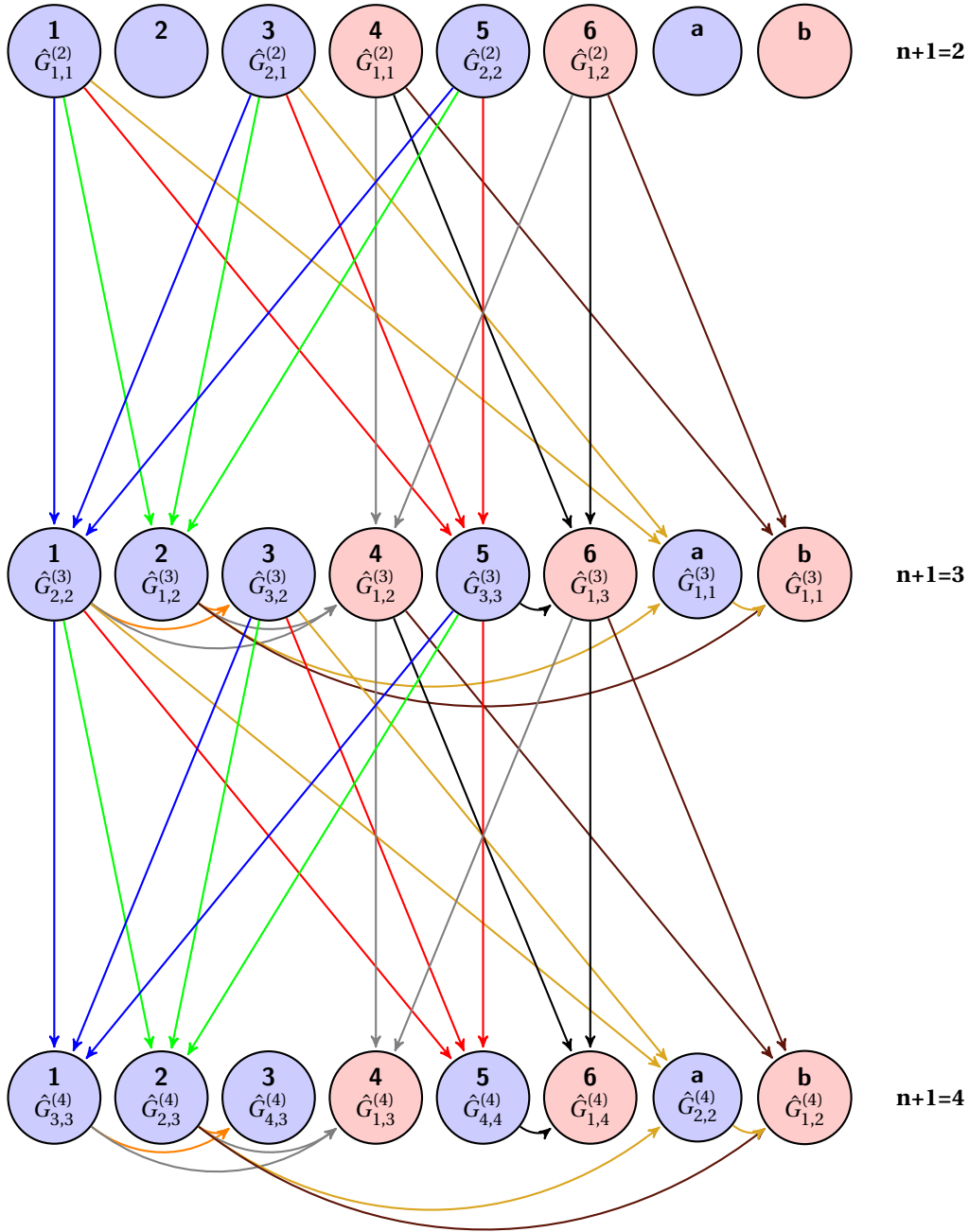
Figure IV.3: Flow chart of the algorithm used to calculate the Green functions \hat{G}_{1,3}^{R,(4)} , \hat{G}_{1,2}^{R,(4)} and \hat{G}_{4,1}^{A,(4)} (pink circles). The label 1, 2, 3, 4, 5 and 6 are the same as those used in sec III.3.2.ii.h. This is also the same order used in the code to calculate the various Green functions. At the first iteration ( n=1 , we are looking for n+1=2 ), there is no next-nearest layers: \hat{G}_{i,j}^{(2)} is only expressed in term of \hat{G}_{i,j}^{(1)} . At the second iteration there are next-nearest-layer interactions, but still one degenerate case: step step 4 = step step 2 . At the third iteration, each Green function is different (at least all indexes are). Equations (III.152), (III.154) and (III.158) give the retarded Green function and the advanced Green function of the current formula (eq. (III.62)).
