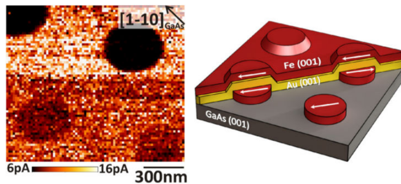
Figure II.2: Image of a buried structure (Fe(1nm)/Au(6nm)/Fe(1nm)/GaAs(001)) made using the BEEM imaging mode ( U_{\text{gap}} = 1.5 V), from Ref. [24]. The dark regions are low current areas, while bright regions are high current area.
