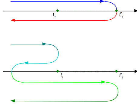
Figure I.3: The above contour C has to be deformed in order to perform the integration. The new contour is formed of two contours, C_1 and C_1' . The first runs from -\infty to t_1 and go back to -\infty . The second goes from -\infty to t_1' and go back to -\infty .
