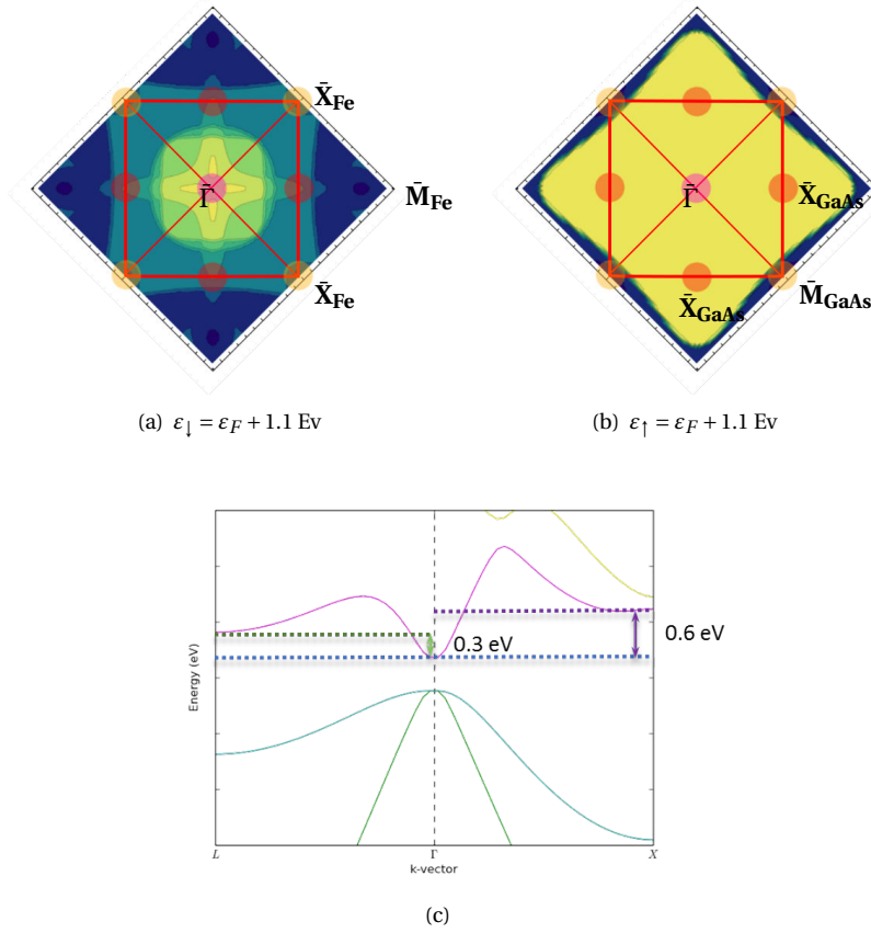
Figure V.8: The current-density vector is projected on the Fe(001) 2D Brillouin-zone for (a) spin-down and (b) spin-up electrons ( \varepsilon = E_F + 1.1\text{eV} ). Yellow color is high current area and blue color is low current area. The available density of states in 2D Brillouin zone for GaAs(001) is represented by red disks. They correspond to the three valleys that are accessible at \Gamma ( \phi_{\Gamma} = \varepsilon_F + 0.75 \text{ eV} ), L ( \phi_L = \phi_{\Gamma} + 0.33 \text{ eV} ) and X ( \phi_X = \phi_{\Gamma} + 0.48 \text{ eV} ) points in (c) the band structure of GaAs (obtained through DFT/LDA calculations using ABINIT [17] code). For the spin-down electrons, no electron can be injected in the L valley of GaAs (that projects in 2D to the point \tilde{X}_{GaAs} ), unlike the spin-up electrons.
