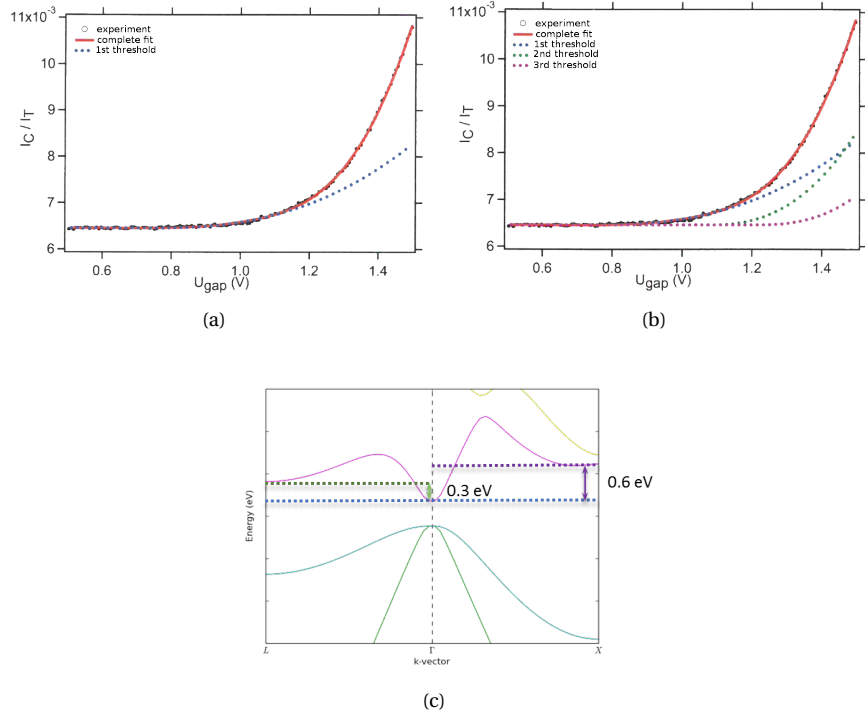
Figure II.5: (a) and (b): Fit of experimental spectroscopy curve [19], using respectively 1 and 3 thresholds (Eq.(II.12)): \phi_\Gamma = \varepsilon_F + 0.75 eV, \phi_L = \phi_\Gamma + 0.33 eV and \phi_X = \phi_\Gamma + 0.48 eV. (c): band structure of GaAs obtained through DFT/LDA calculations. The 3 thresholds of the fit correspond to the 3 minima, \Gamma , L and X of the conduction band of GaAs.
