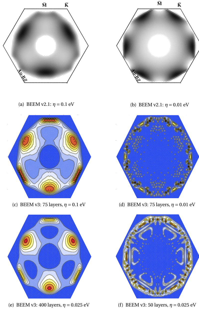
Figure V.18: Distribution of the elastic current, 1 eV above the Fermi level, in Au(111) obtained through BEEM v2.1 and BEEM v3. Increasing \eta or the number of layers leads to the loss of the 6-fold symmetry, that is to say the loss of the time-reversal symmetry, that is similar to equilibrium calculations.
