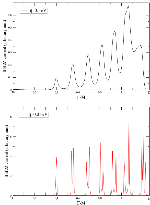
Figure V.12: BEEM current along the \bar{\Gamma}\bar{M} path in the Brillouin zone for 20 layers and two values of \eta : \eta = 0.1 eV and \eta = 0.01 eV. Increasing \eta spreads the peaks.
