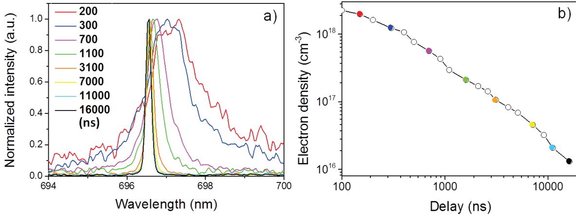
Figure 3.20 Evolution of the profile of the Ar I 696.5 nm line at different delays (a) and that of the electron density (b) in a plasma induced by a 20-mJ laser pulse at 1064 nm in Ar gas at the atmospheric pressure. The same color code as in (a) is used in (b).
