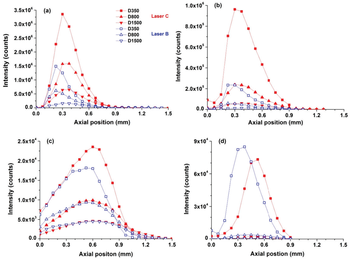
Figure 4.3 Axial emission intensity profiles of the plasmas induced by the two types of pulses: laser B of pulse duration of 4 ns and laser C with pulse duration of 45 ns. A same fluence of 65 mJ/cm 2 is used for the two lasers. Different species in the plasma are (a) neutral aluminum evaporated from the target, (b) corresponding ions of aluminum, (c) neutral argon contributed by the ambient gas, and (d) corresponding ions of argon.
