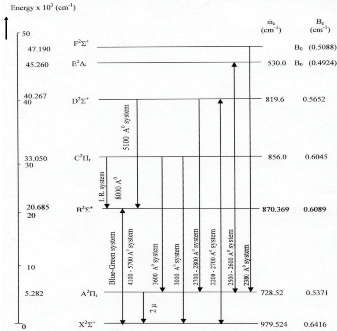
Figure 2.2 Energy level diagram of AlO molecule [76]
