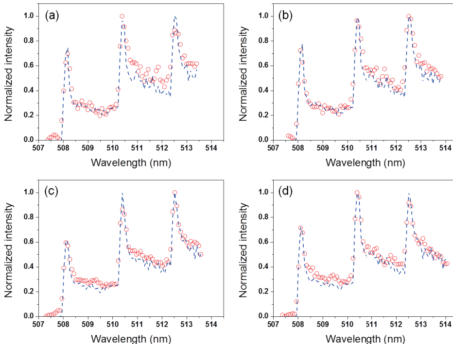
Figure 6.10 Experimental molecular emission intensities (red open circles) measured at 4 delays of 10 \mu s (a), 15 \mu s (b), 20 \mu s (c) and 30 \mu s (d) for a plasma induced by a 20 mJ pulse. Experimental data are fitted with synthetic spectrum (dashed blue curve).
