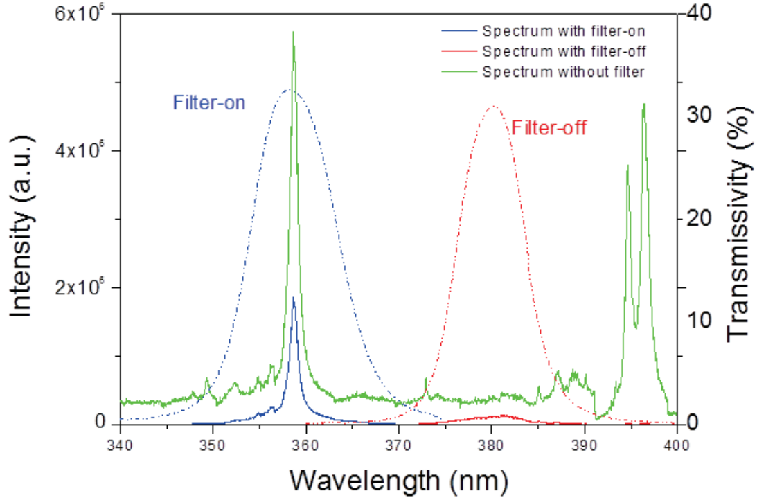
Figure 3.5 Spectra around 370 nm including the Al II 358.6 nm line, without filter, with a filter-on and with a filter-off.
