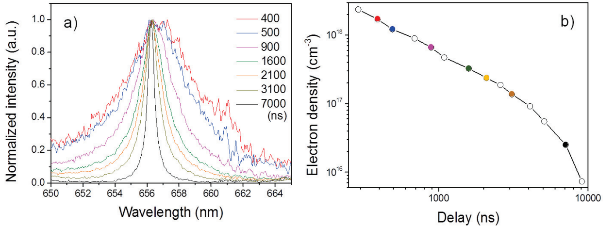
Figure 3.19 (a) Evolution of the H_\alpha 656.3 nm line at different delay and (b) that of the electron density in the plasma induced by a 50-mJ laser pulse at 1064 nm in the atmospheric air. The same color code as in (a) is used for (b).
