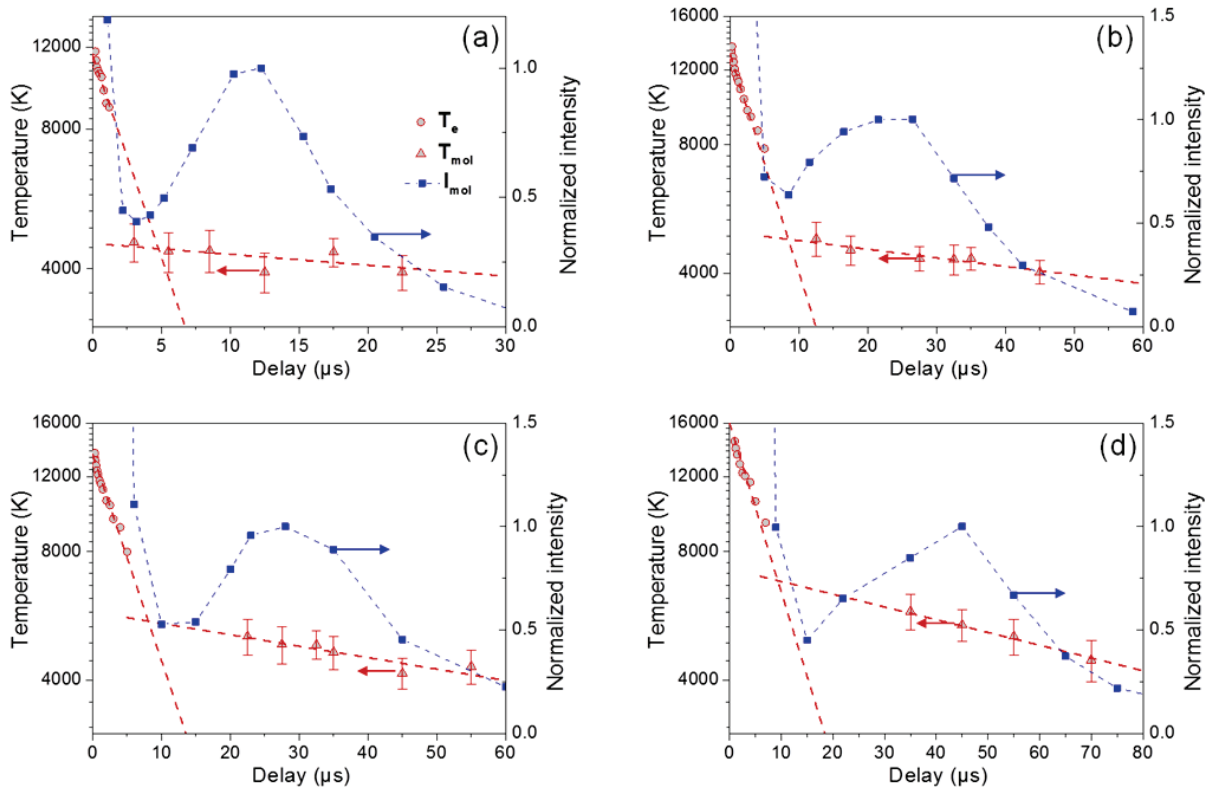
Figure 6.14 Temperatures of the plume (in red) and molecular emission intensity (in blue) as a function of delay with the ablation laser pulse energy of 5 mJ (a), 20 mJ (b), 30 mJ (c) and 50 mJ (d).
