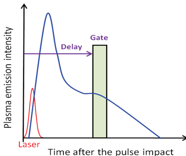
Figure 1.10 Schematic presentation of the time evolution of the plasma emission. The red curve corresponds to the profile of laser pulse. The blue curve represents the plasma emission intensity after the ablation as a function of time.
