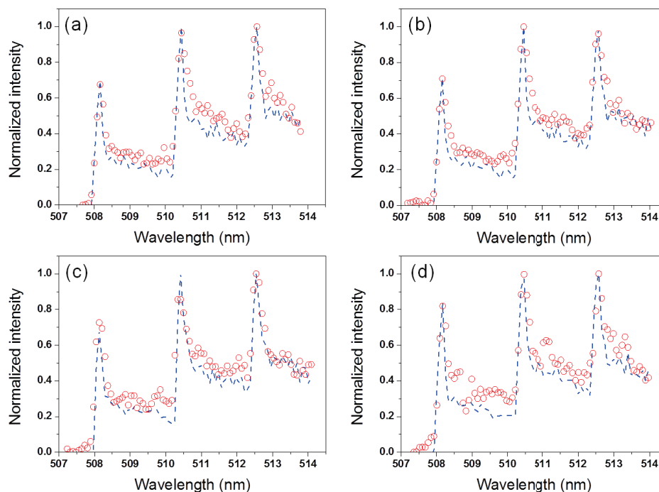
Figure 6.12 Experimental molecular emission intensities (red open circles) measured at 4 delays of 30 \mu s (a), 40 \mu s (b), 50 \mu s (c) and 60 \mu s (d) for a plasma induced by a 50 mJ pulse. Experimental data are fitted with synthetic spectrum (dashed blue curve).
