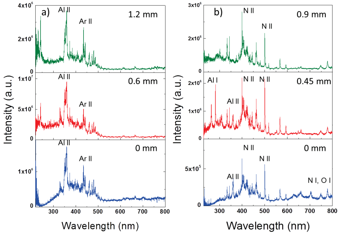
Figure 5.4 Emission spectra of the plasma at different axial positions in the ambient gas of (a) argon and (b) air recorded at a delay of 50 ns.
