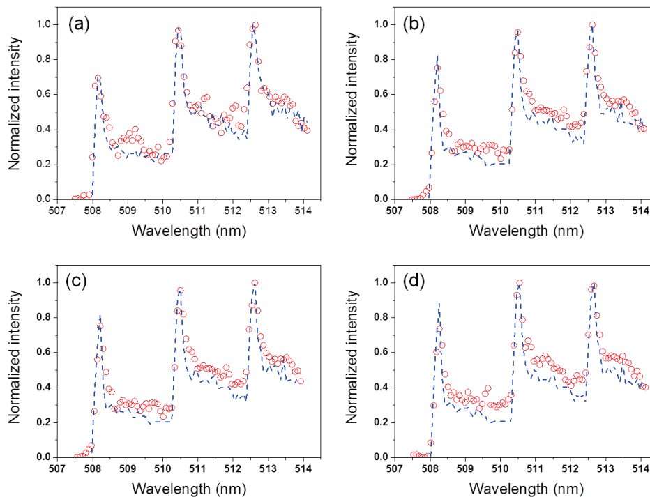
Figure 6.9 Experimental molecular emission intensities (red open circles) measured at 4 delays of 2 \mu s (a), 4 \mu s (b), 7 \mu s (c) and 10 \mu s (d) for a plasma induced by a 5 mJ pulse. Experimental data are fitted with synthetic spectrum (dashed blue curve).
