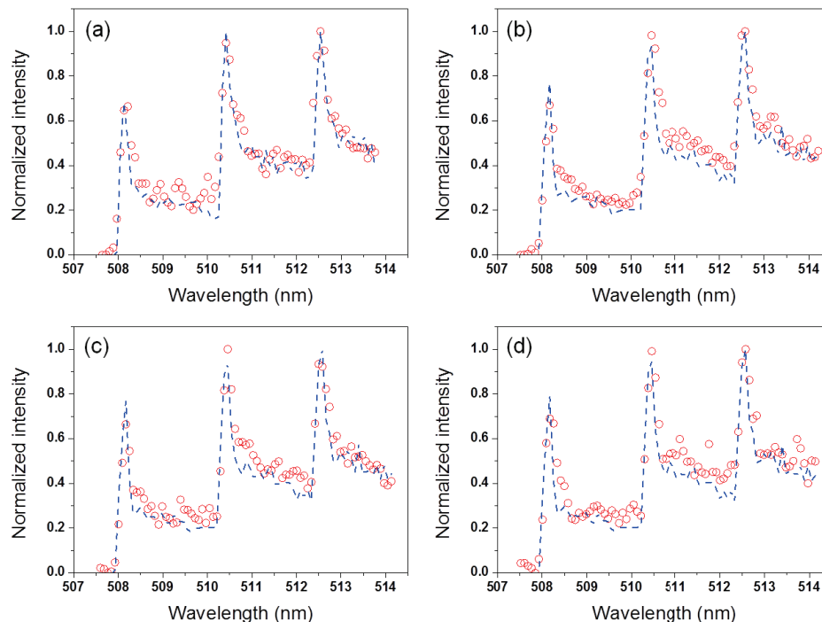
Figure 6.11 Experimental molecular emission intensities (red open circles) measured at 4 delays of 20 \mu s (a), 25 \mu s (b), 30 \mu s (c) and 35 \mu s (d) for a plasma induced by a 30 mJ pulse. Experimental data are fitted with synthetic spectrum (dashed blue curve).
