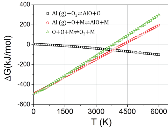
Figure 6.1 The variation of the Gibbs function for the 3 reactions of Eqs (6-1), (6-2) and (6-3). Black points correspond to the reaction Eq. (6-1), red ones to the reaction Eq. (6-2) and green ones to the reaction Eq. (6-3)
