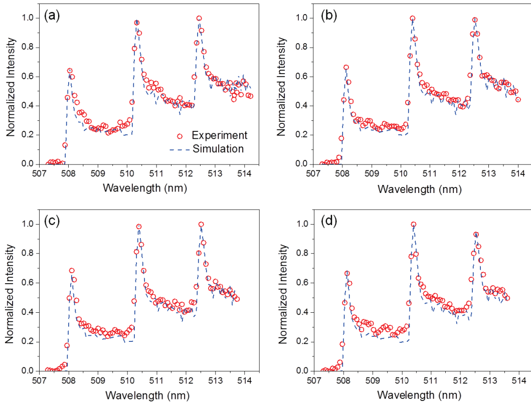
Figure 6.4 Emission band B^2\Sigma^+ - X^2\Sigma^+ of \text{AlO} molecules. Experimental intensities represented by red open circles, are measured at 4 delays of 5 \mu\text{s} (a), 10 \mu\text{s} (b), 15
