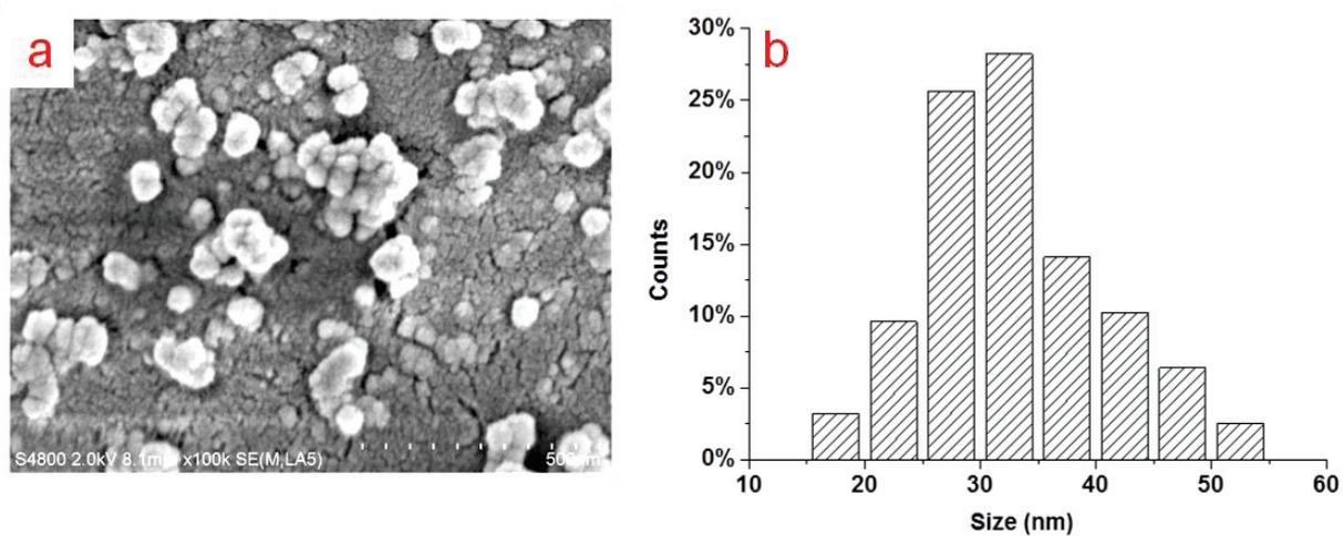
Figure 6.19 (a) SEM image of the collected nanoparticles obtained with 5-mJ ablation and (b) their size distribution (b).
