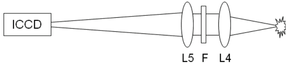
Figure 3.4 Experimental setup for “image” type measurement. L4, L5: lenses, F: filter.
