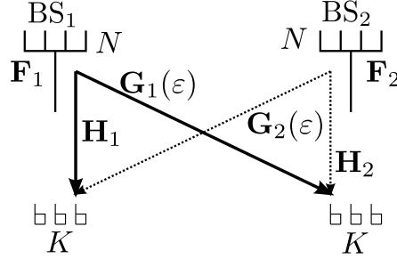
Figure 4.1: Simple 2 BS Downlink System.
