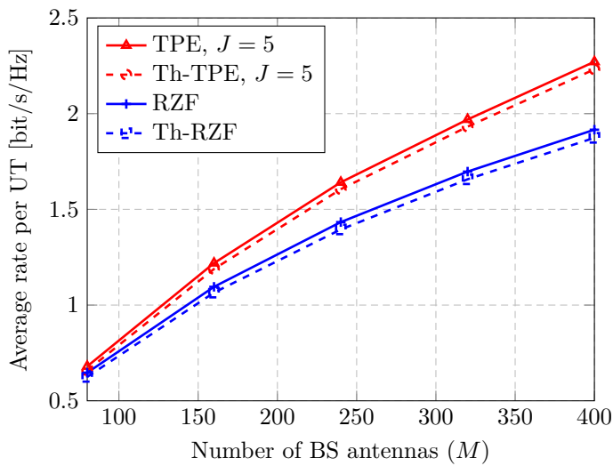
Figure 3.12: Comparison between the empirical and theoretical user rates. This figure illustrates the asymptotic accuracy of the deterministic approximations.
