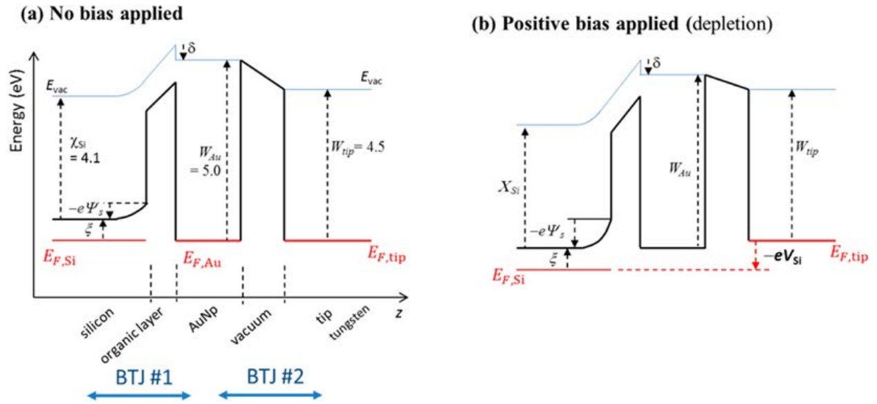
Figure 5.8: Energy Diagram of the DBTJ. The first barrier tunnel junction is between the silicon and the selected AuNP, and the second BTJ is between this AuNP and the STM tip. From Caillard et al. Langmuir (2013).
