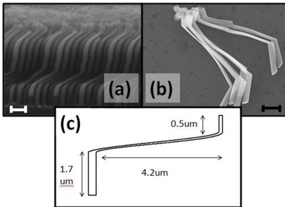
Figure 8.11: SEM images of bended silicon nanowires. Double bended silicon nanowires are the result of repeating the process twice (a). When broken down with Sonication, pillars can be drop casted on a flat surface (b) where we can estimate more accurately the dimensions (c) the thickness of the thin part is estimated to be 80nm. Note: picture (a) have been taken using a low resolution JEOL tabletop SEM. Scale bars: 1\mu\text{m} .
