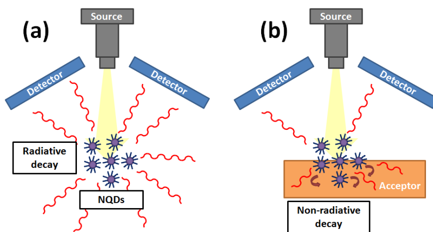
Figure 3.5: Visual representation of NQDs decay without (a) and with an acceptor (b). Without an acceptor the decay is mostly radiative. With an acceptor, the decay is a combination of radiative decay, RET and NRET.
