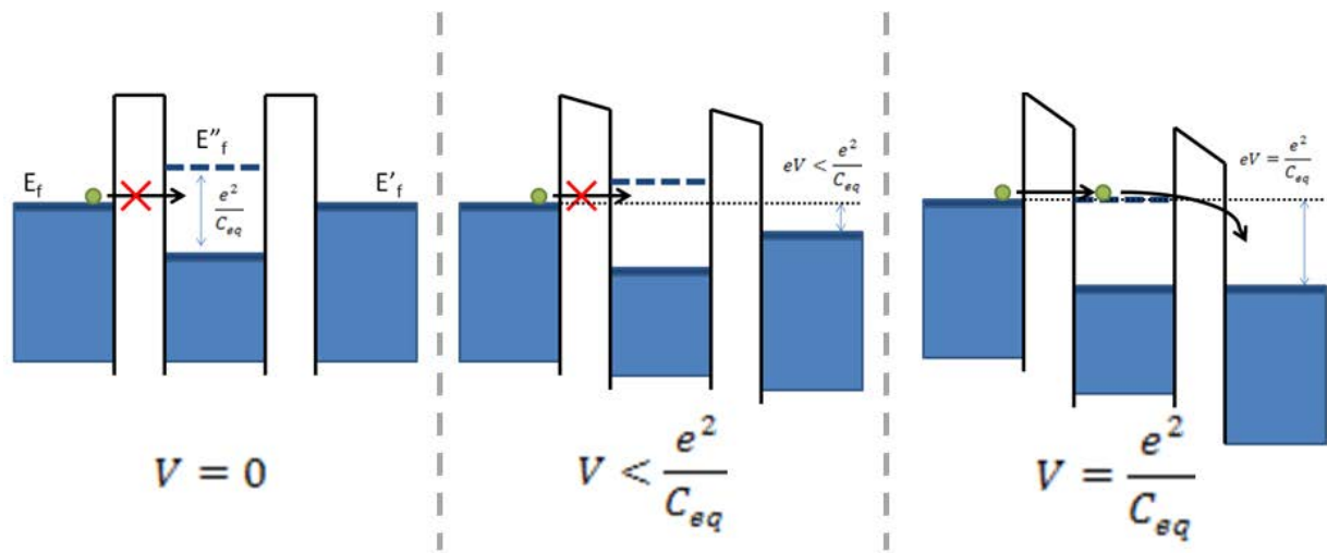
Figure 2.4: Band diagram of a symmetrical DBTJ with different applied voltage
