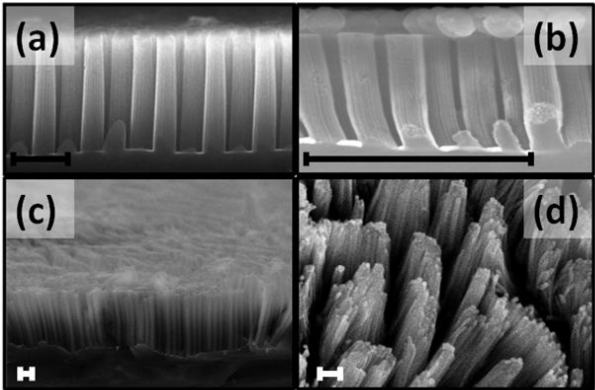
Figure 8.9: SEM images of silicon nanowires. Side-view of Straight pillars obtained with 500nm beads (a) and 200nm beads (b). Pillars can be etched for a longer time which gives them a more slender aspect (side-view, c) but it makes them collapse when it is overdone (top view, d). Note: images (c) and (d) have been taken using a low resolution JEOL tabletop SEM. Scale bars: 1 \mu m.
