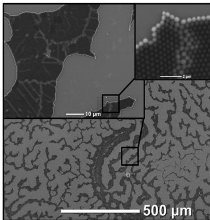
Figure 8.2: SEM images of a silicon substrate with a layer of polystyrenes nanoparticles with a diameter of 500nm deposited with spin coating. Insets show several zoom-in that gives indication of a good localized assembly of the beads despite a low coverage (~15%). Note: the image has been taken with a low resolution JEOL tabletop SEM.
