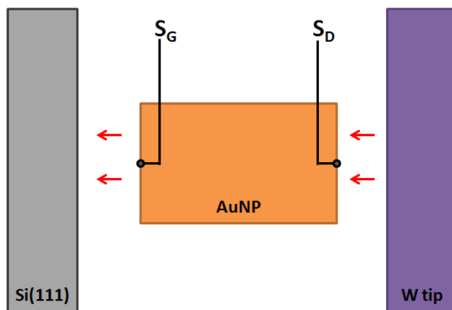
Figure 7.4: Geometry for calculating the current flow through the nanoparticle. The spherical shapes are replaced with planar surfaces. S_D and S_G are taken as 1/10 of the particle cross section ( 4\pi R^2 ).
