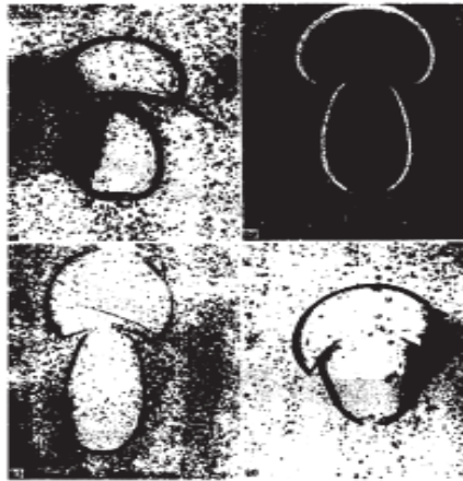
Figure 4.23: Coalescence of two bubbles in 3D: results obtained in [NGK74].
