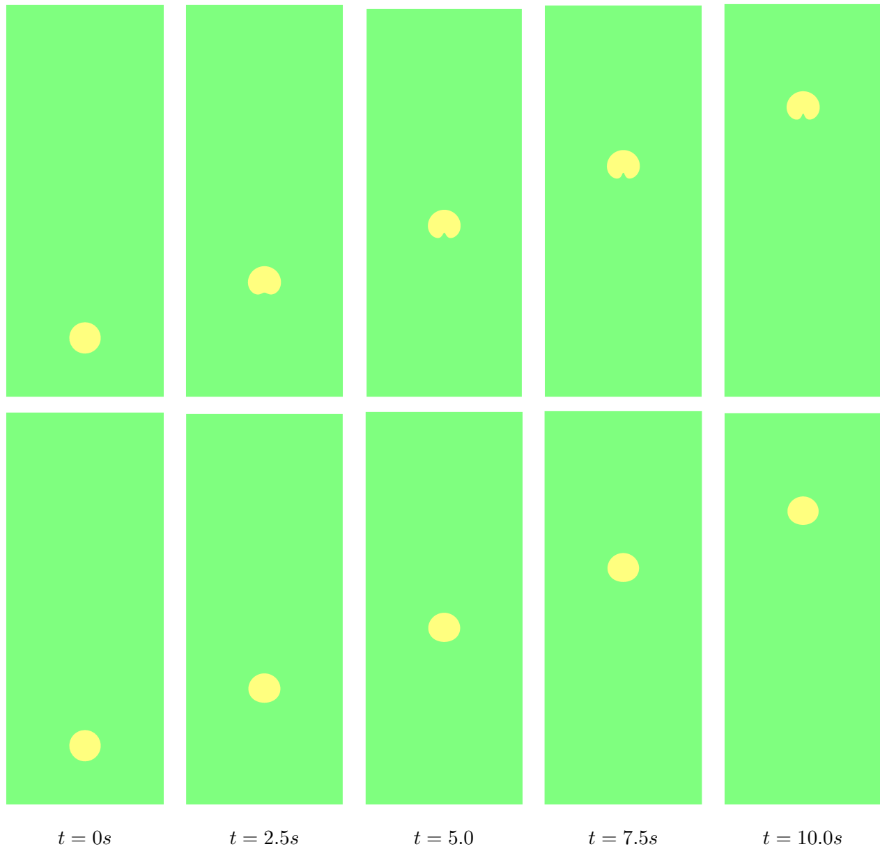
Figure 2.4: Rising bubble in 2D: evolution of the interface in time: (top) without surface tension; (bottom) with surface tension.
