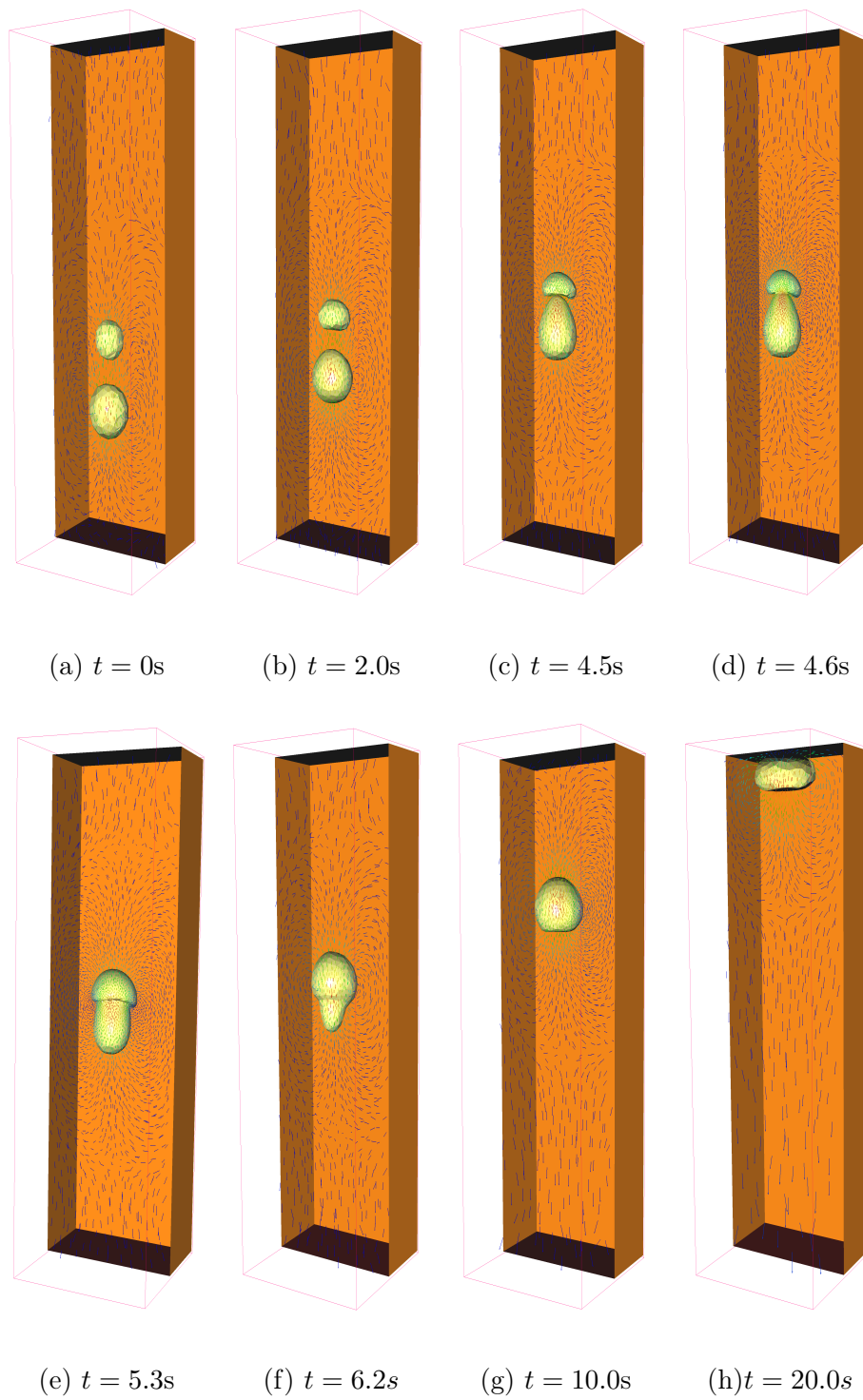
Figure 4.26: Coalescence of two bubbles in 3D: Velocity fields, cutting in the plan y = 0.5 .
