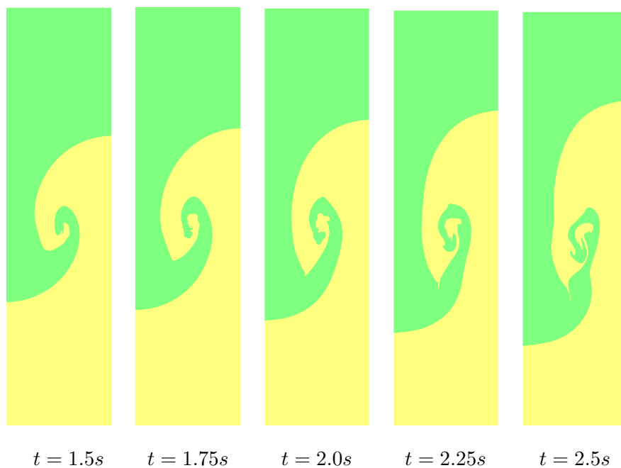
Figure 4.15: Rayleigh-Taylor instability in 2D: evolution of the interface with At = 0.5 , Re = 1000 .
