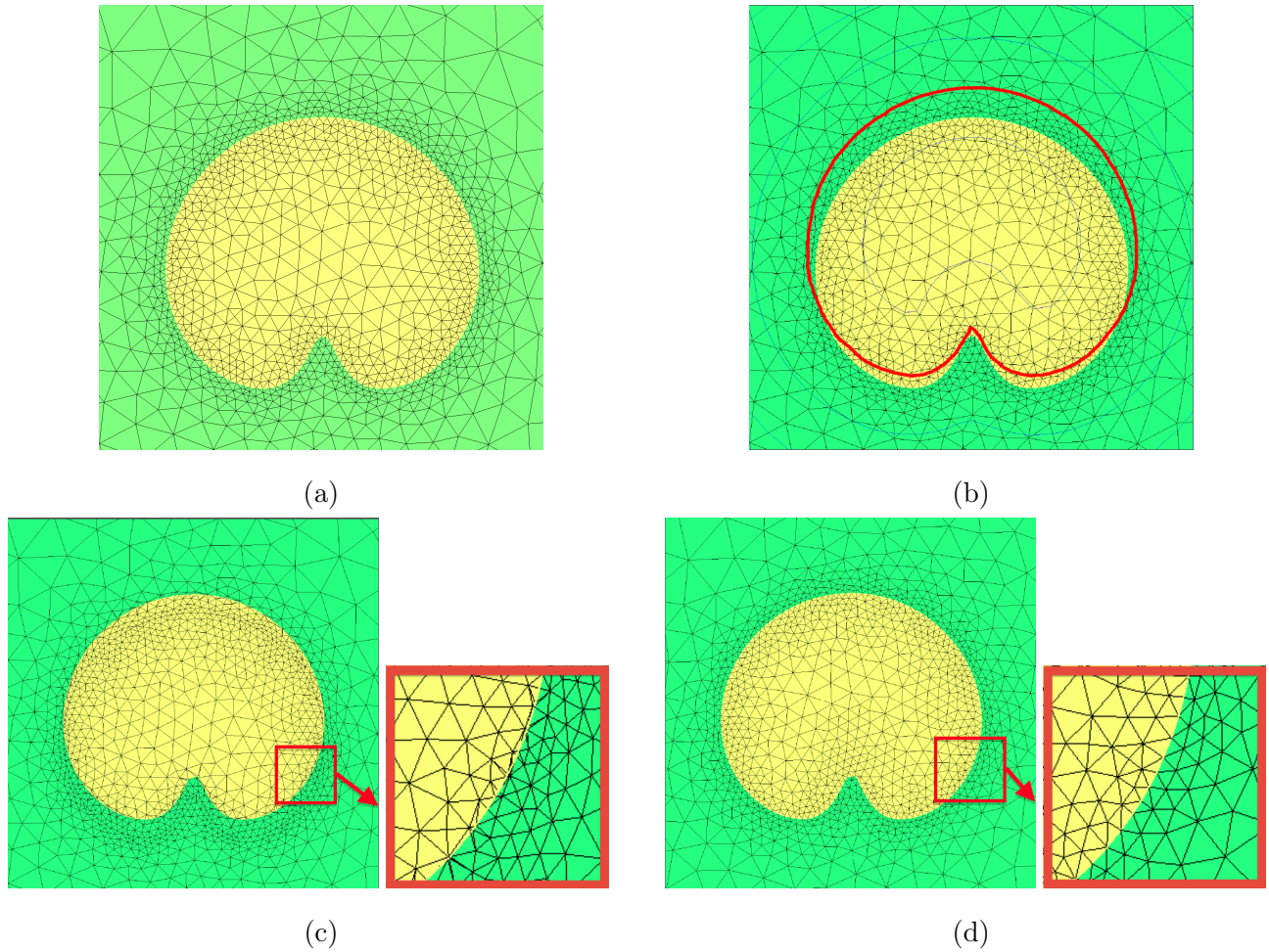
Figure 3.6: Illustration for mesh adaptation in n^{\text{th}} iteration for two fluids flow. (a): Initial mesh T^n (used to obtain \mathbf{u}^n ), (b): The new level set function \phi^n with the red line is the zero-level set, (c): Explicit discretization of zero-level set of \phi^n , the obtained mesh is not well-shaped, (d): High-quality adapted mesh in which the zero-level set of \phi^n is explicitly discretized.
