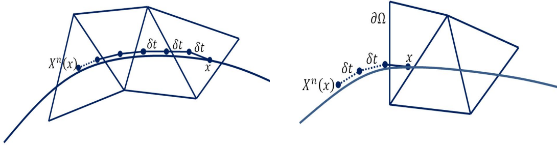
Figure 1.1: (left) travel characteristic point with time \delta t and (right) characteristic point is go out to domain.
