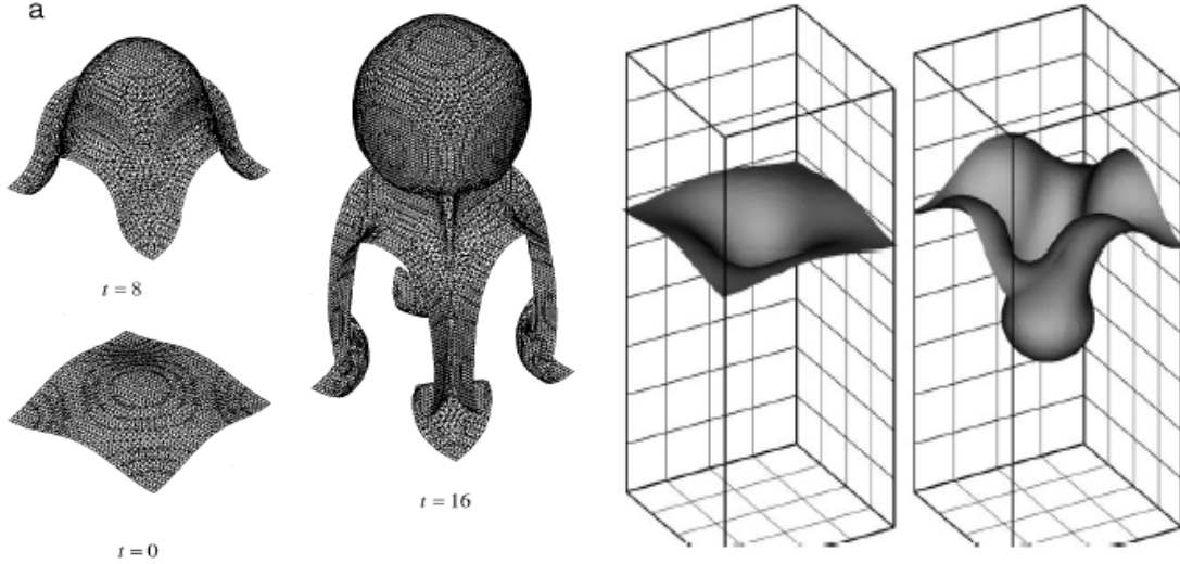
Figure 4.19: Rayleigh-Taylor instability in 3D: results obtained in [LJG96] (left) and [LFX05] (right).
