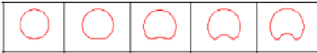
Figure 4.8: Rising bubble in 2D: interaction of surface tension in case of Re = 5 and from left to right: Bo = 10 ; Bo = 20 ; Bo = 50 ; Bo = 100 ; Bo = 200 in [HSL07].
