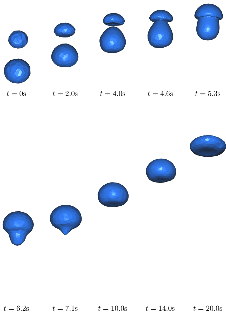
Figure 4.22: Coalescence of two bubbles in 3D: evolution of the interfaces in time. The coalescence occurs at t = 4.6s .
