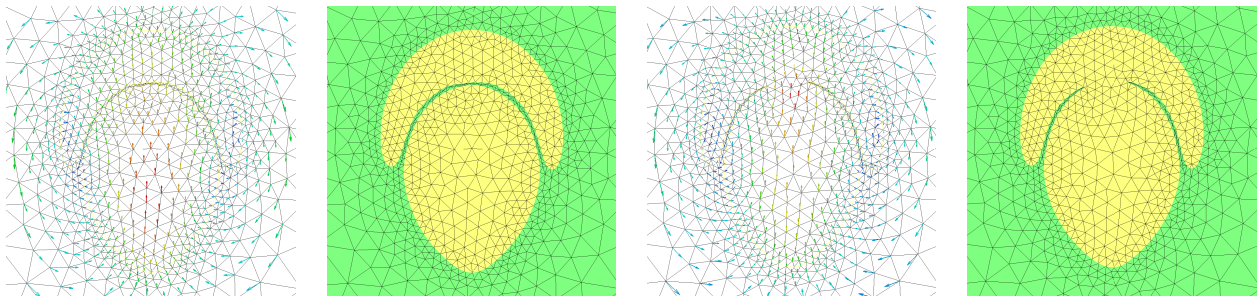
Figure 4.21: Zoom of mesh and velocity of 2 bubbles at t = 12.6s and t = 12.7s .
