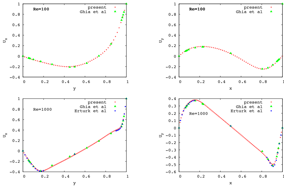
Figure 4.2: Cavity in 2D: velocity profile for u_x and u_y in cases of Re=100 and Re = 1000 .
