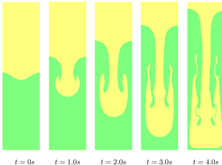
Figure 4.12: Rayleigh-Taylor instability in 2D: evolution of the interface in time with At = 0.3 .
