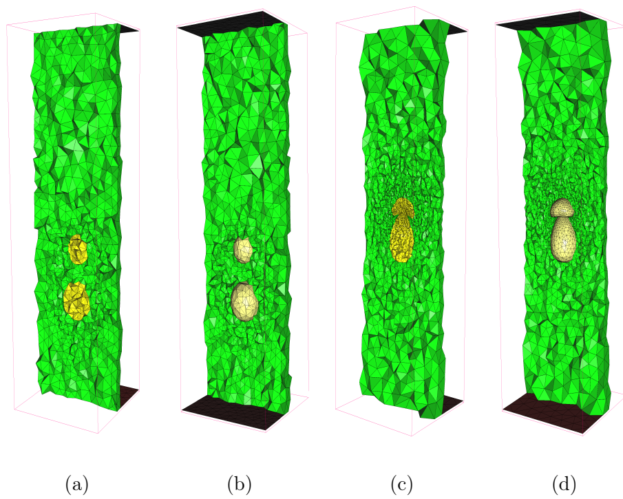
Figure 4.27: Coalescence of two bubbles in 3D: Initial mesh with 11113 vertices (two first ones) and adapted mesh with 30101 vertices at the coalescence (two last ones).
