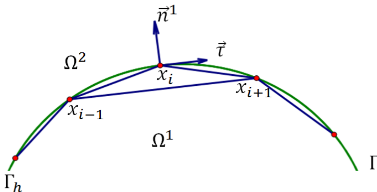
Figure 2.5: Illustration of geometric discretization of interface in 2D.
