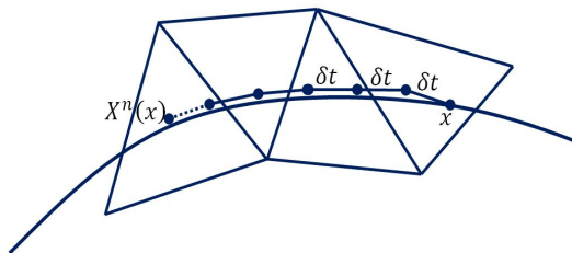
Figure 2.6: Illustration of characteristic curve approximation.
