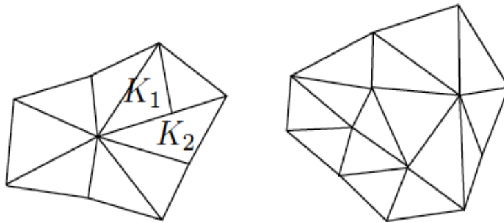
Figure 3.1: Examples of non conforming mesh (left) and conforming mesh (right).
