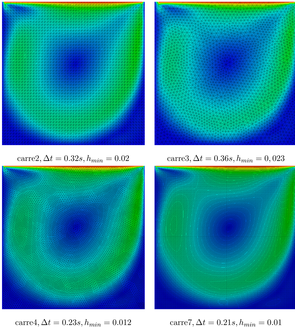
Figure 1.4: Cavity in 2D: steady-state solution in case of Re = 1000 for different meshes with the different time steps.
