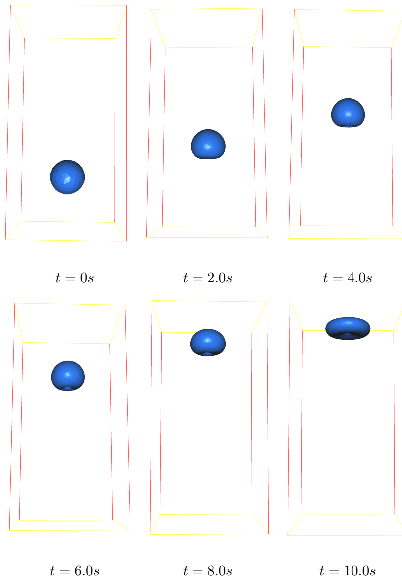
Figure 4.10: Rising bubble in 3D: evolution of the interface in time.
