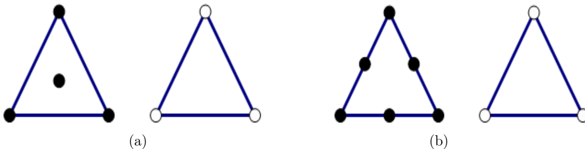
Figure 1.2: Degree of freedom: (a) mini element ( \mathbb{P}_1 bubble/ \mathbb{P}_1 ); (b) Taylor-Hood element ( \mathbb{P}_2/\mathbb{P}_1 )
