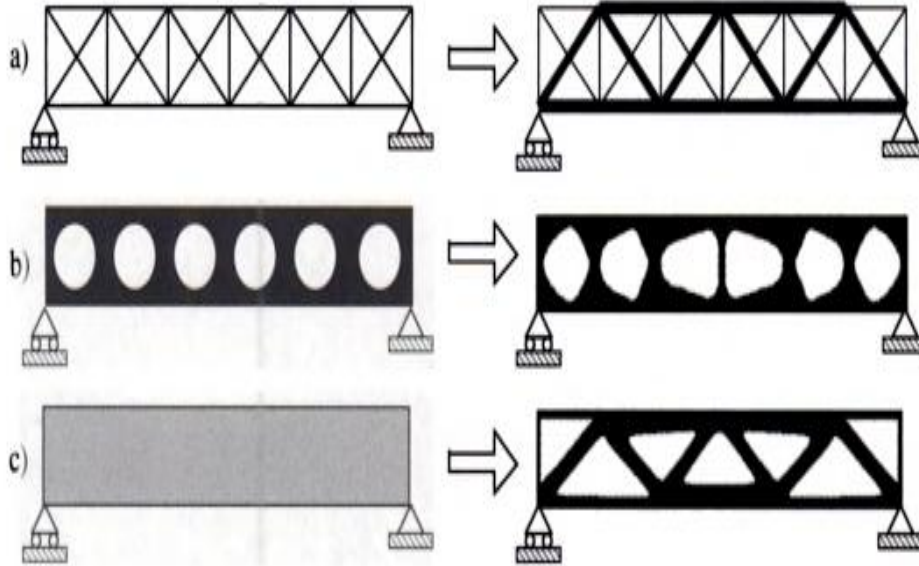
Figure 4.28: Three categories of structural optimization. (a) Size optimization of a truss structure, (b) shape optimization and (c) topology optimization. The initial problems are shown at the left hand side and the optimal solutions are shown at the right. (from [BS03])
