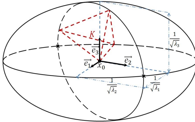
Figure 3.4: Geometrical illustration of a unit ellipsoid \mathcal{B}_M(x_0) with an inscribed element K associated to a metric tensor in 3D.
