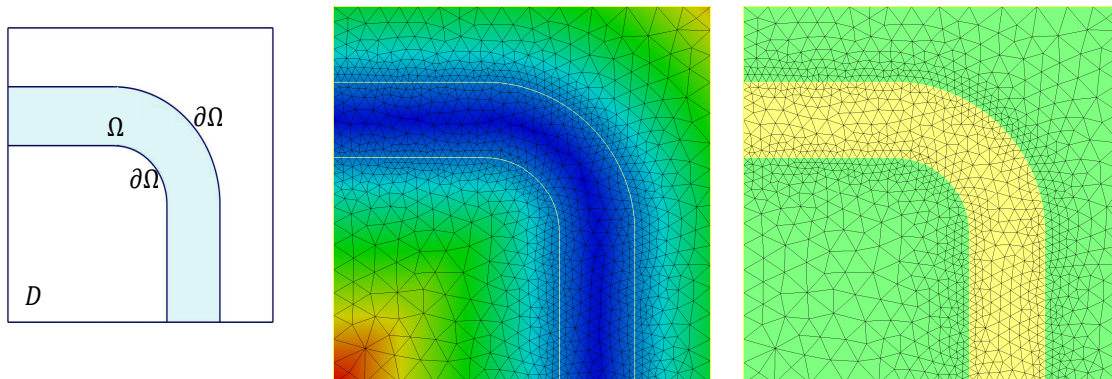
Figure 4: (Left) A shape \Omega \subset D , (Center) representation of shape \Omega by associated level set function and (Right) triangular mesh of D enclosing a mesh of \Omega (yellow elements).
