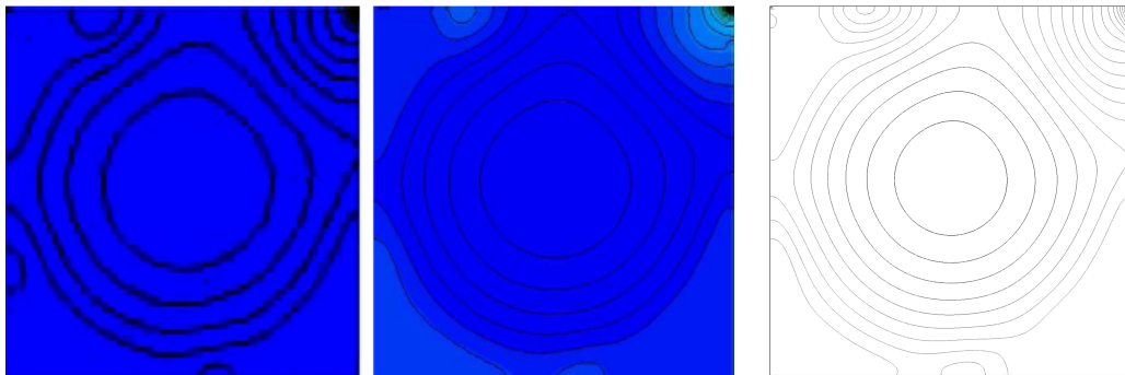
Figure 4.3: Cavity in 2D: Isolines of pressure with Re = 10000 . Left: result in [VG04]. Center: result in [HRK + 10]. Right: present result.
