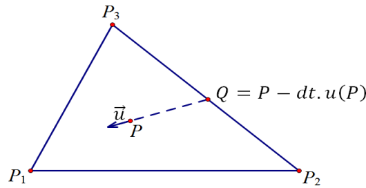
Figure 2.8: Illustrations of time dt to go out an element.
