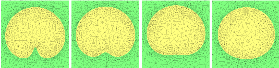
Figure 4.7: Rising bubble in 2D: interaction of surface tension on the final bubble (at time t=10s ) with different tension coefficients, from left to right: \gamma = 6e - 5 ; \gamma = 6e - 3 ; \gamma = 2.5e - 2 ; \gamma = 9e - 2 .
