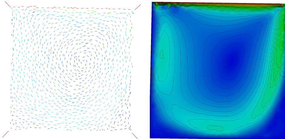
Figure 1.6: Cavity in 3D: (left) velocity of the flow and (right) streamlines in the plane ( z = 0.5 ) for Re = 1000 .
