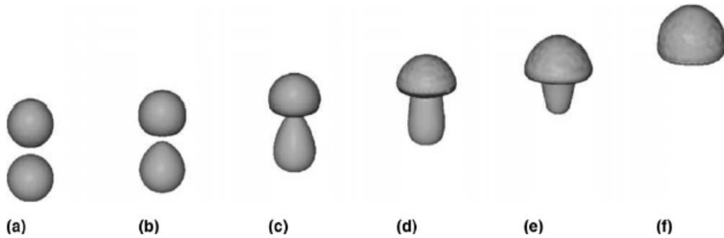
Figure 4.25: Coalescence of two bubbles in 3D: results obtained in [dSMN + 04]: (a) 0.0 s; (b) 0.03 s; (c) 0.06 s; (d) 0.09 s; (e) 0.12 s; (f) 0.15 s.
