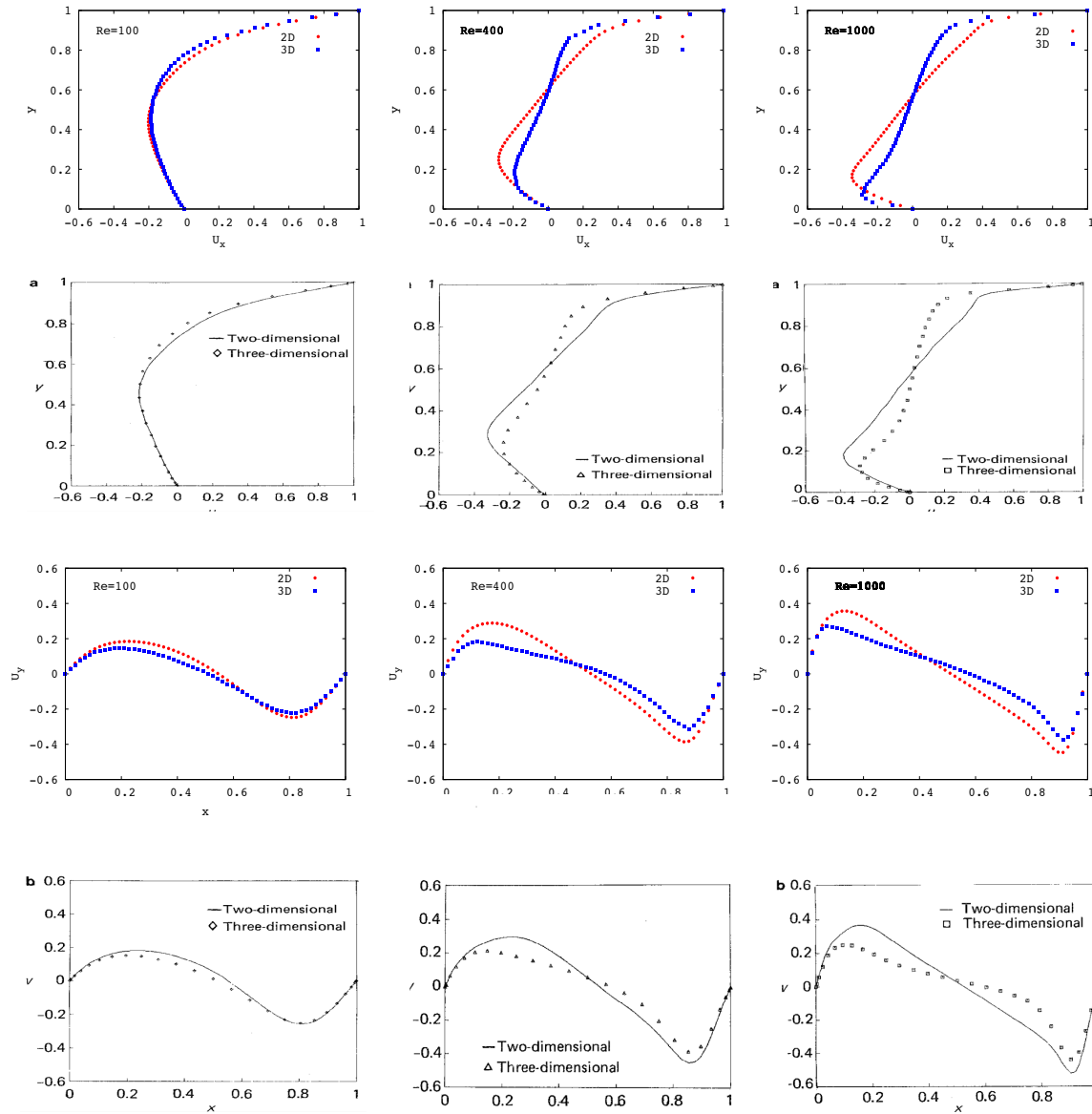
Figure 4.5: Cavity in 3D: velocity profiles on vertical centerline. The first and third rows: present results. The second and fourth rows: results obtained in [KHT87].
