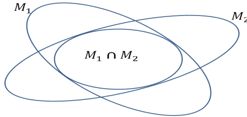
Figure 3.5: Intersection of two metric tensors.
