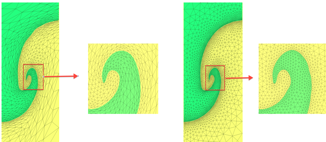
Figure 4.17: Rayleigh-Taylor instability in 2D: zoom of adapted mesh in the vicinity of the interface, left: anisotropic mesh, right: isotropic mesh.
