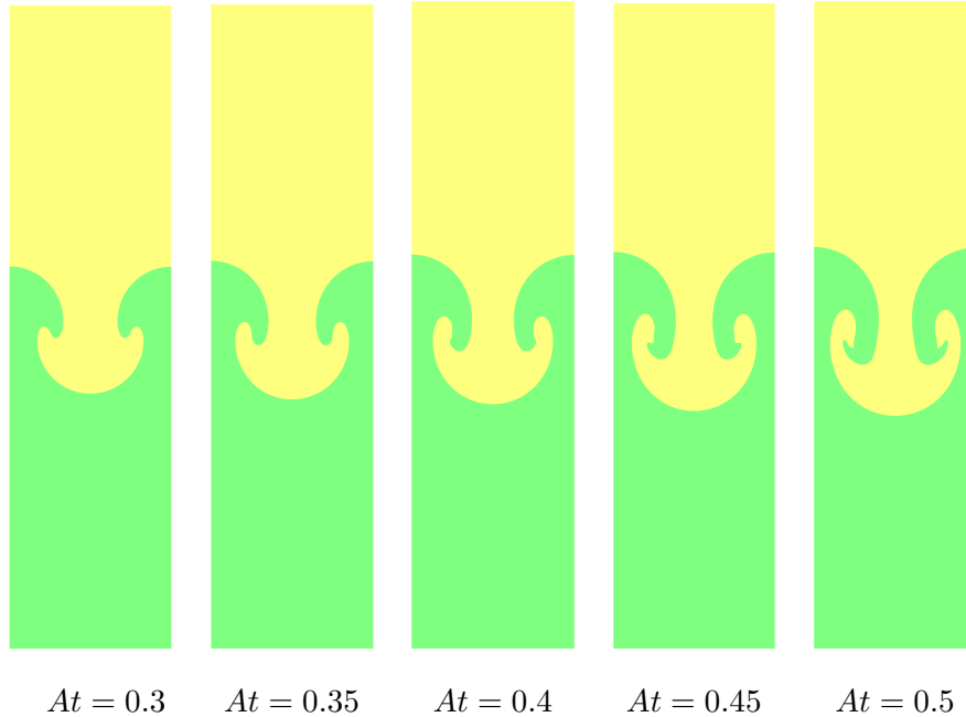
Figure 4.13: Rayleigh-Taylor instability in 2D: evolution of the interface with different Atwood numbers.
