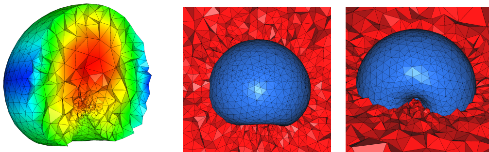
Figure 4.11: Rising bubble in 3D: zoom of and adapted mesh at time t = 6.0s .
