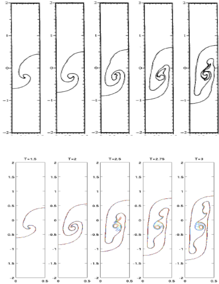
Figure 4.16: Rayleigh-Taylor instability in 2D: extracted results of evolution of the interface with At = 0.5 , Re = 1000 in [FGQ01] (top) and [CCG08] (bottom).
