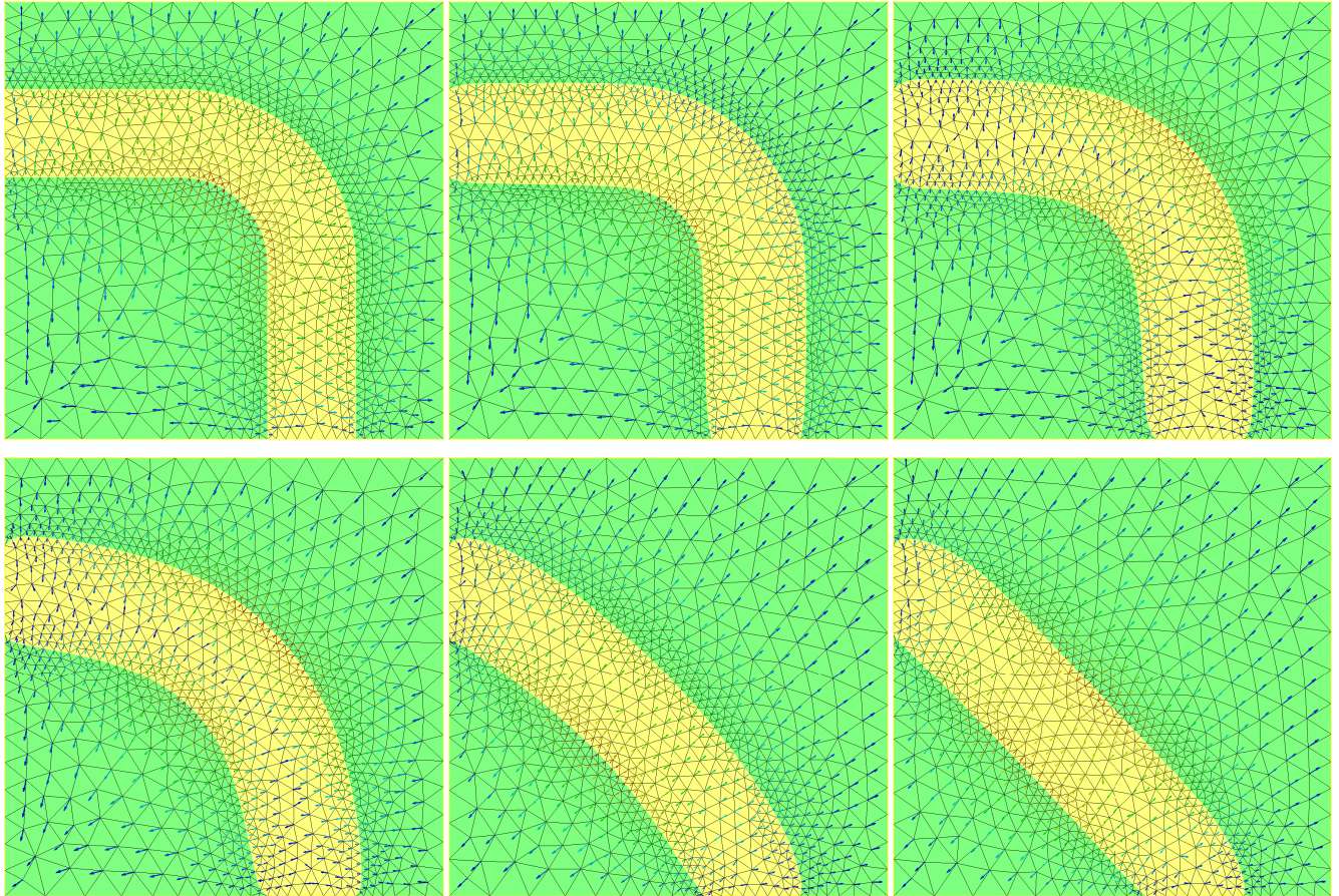
Figure 5.5: Deformation process of domain in the case test of elbow. From top to bottom, left to right: 1 th , 50 th , 70 th , 85 th , 100 th and 150 th iterations of the case test.
