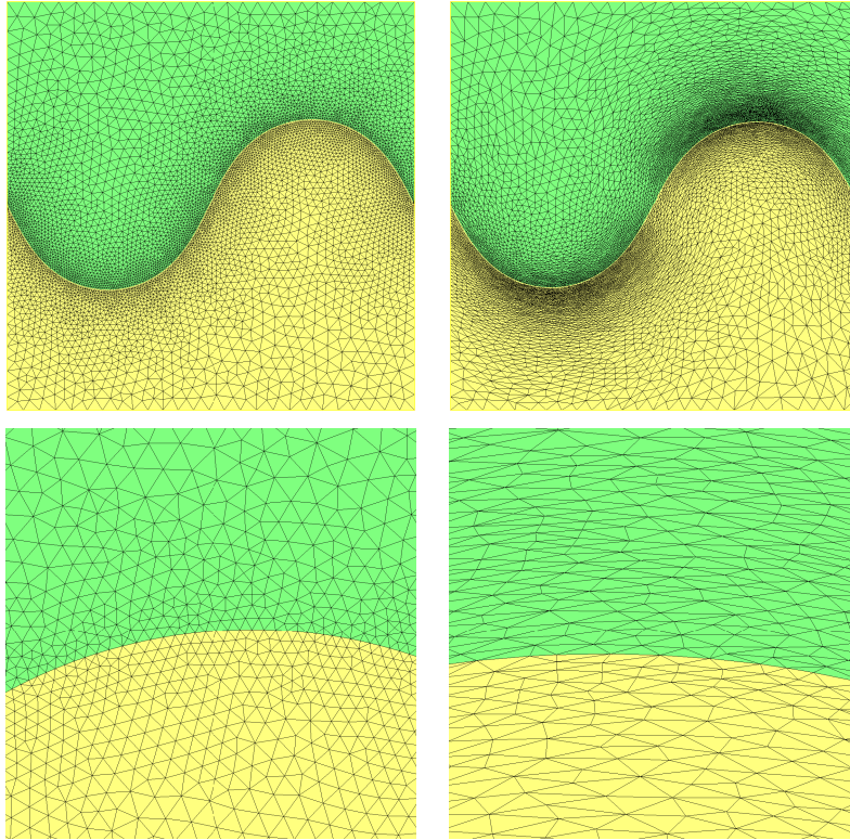
Figure 3.3: Example of mesh adaptation about 7000 vertices: isotropic mesh (top, left) and anisotropic mesh (top, right); zoom in the vicinity of the interface triangulations (bottom).
