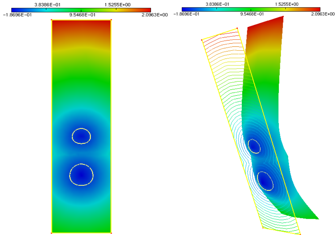
Figure 2.2: Examples of computational domains with level-set function in 2D.
