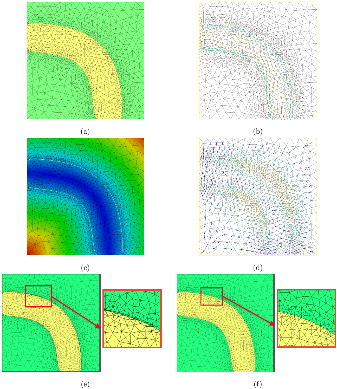
Figure 5.4: Implements in n^{\text{th}} -iteration. (a): Explicit discretization of shape \Omega^n in mesh \mathcal{D}_{\Omega^n} , (b): Velocity field of Stokes problem on sub-mesh T_{\Omega^n} of shape \Omega^n , (c): Shape-domain \Omega^n in mesh \mathcal{D}_{\Omega^n} corresponding level set function \phi^n , (d): Velocity field V^n on \mathcal{D}_{\Omega^n} for advection of \phi^n , (e): Explicit discretization of zero-level set of \phi^{n+1} , the obtained mesh \tilde{\mathcal{D}}_{\Omega^{n+1}} is very ill-shaped, (f): High-quality mesh \mathcal{D}_{\Omega^{n+1}} in which the new shape \Omega^{n+1} is explicitly discretized.
