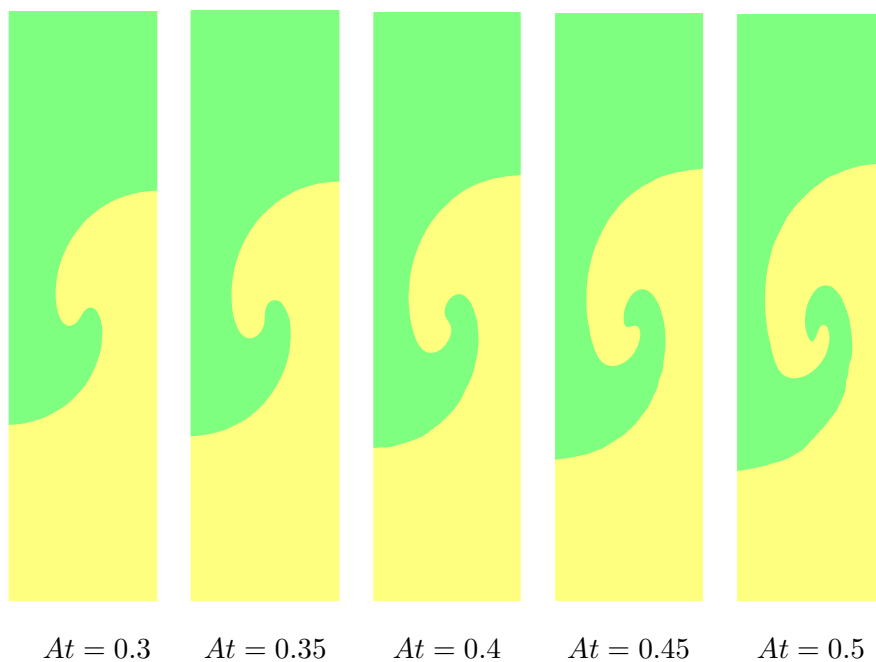
Figure 4.14: Rayleigh-Taylor instability in 2D: evolution of the interface with different Atwood numbers and reduced domain.
