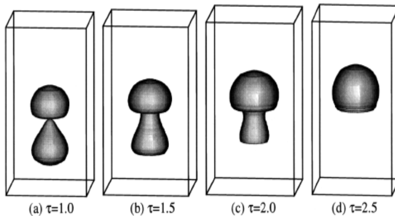
Figure 4.24: Coalescence of two bubbles in 3D: results obtained in [CL98].
