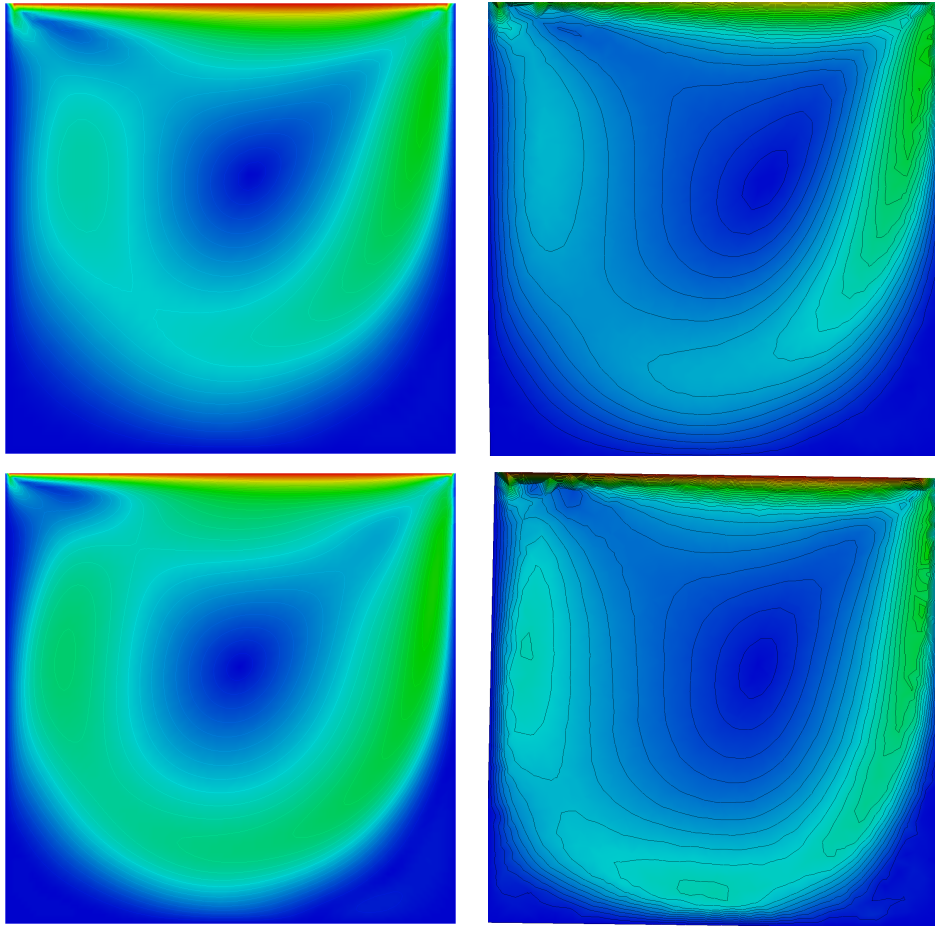
Figure 4.4: Cavity in 3D: from left to right, streamlines in 2D and in the plane ( z = 0.5 ) of 3D for Re = 400 (top), Re = 1000 (below).
