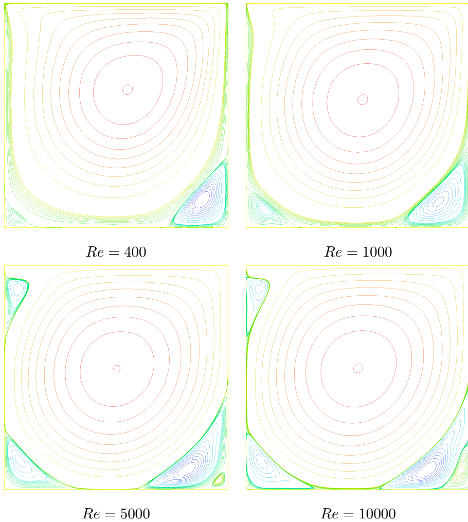
Figure 4.1: Cavity in 2D: Streamlines for different Reynolds number.
