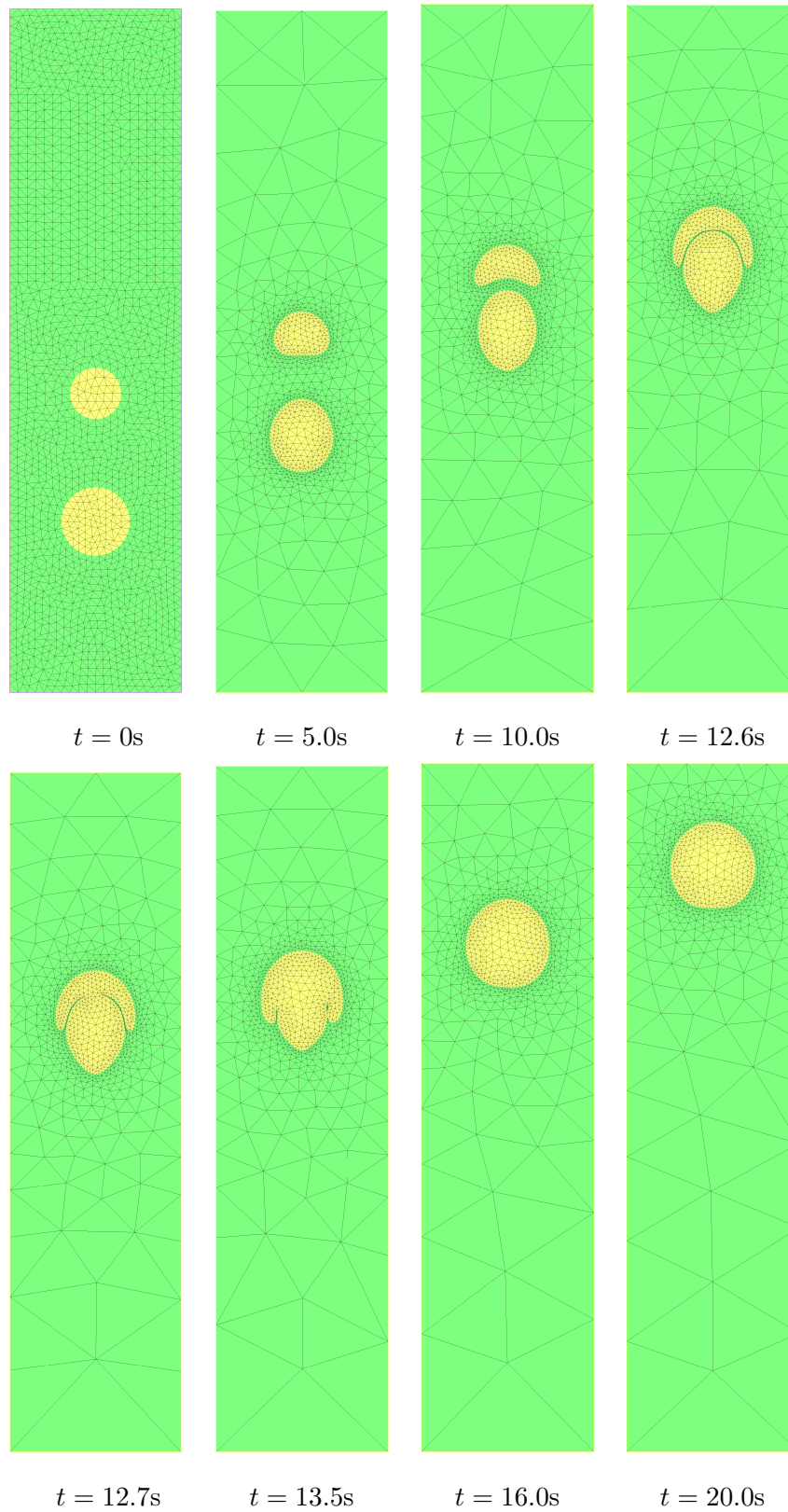
Figure 4.20: Coalescence of two bubbles: evolution of the interface in time. The coalescence occurs at t = 12.7s .
