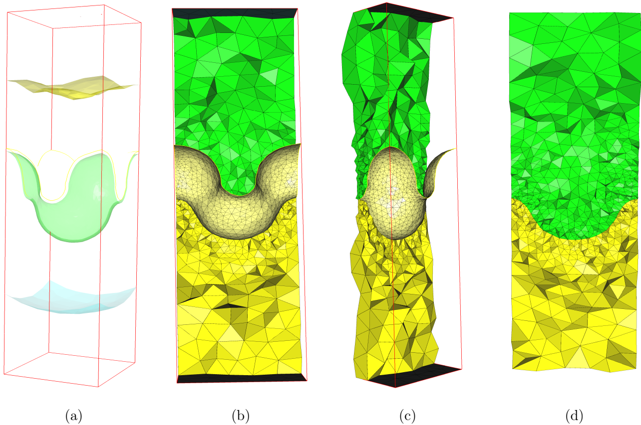
Figure 3.7: Illustration for mesh adaptation in 3D ( h_{min} = 1.e - 2, h_{max} = 0.2, h_{grad} = 1.3, h_{hausd} = 5e - 3 ). (a): isosurfaces of level set function, (b) and (c): Final adapted mesh where zero-surfaces is explicitly discretized , (d): a cut of final mesh.
