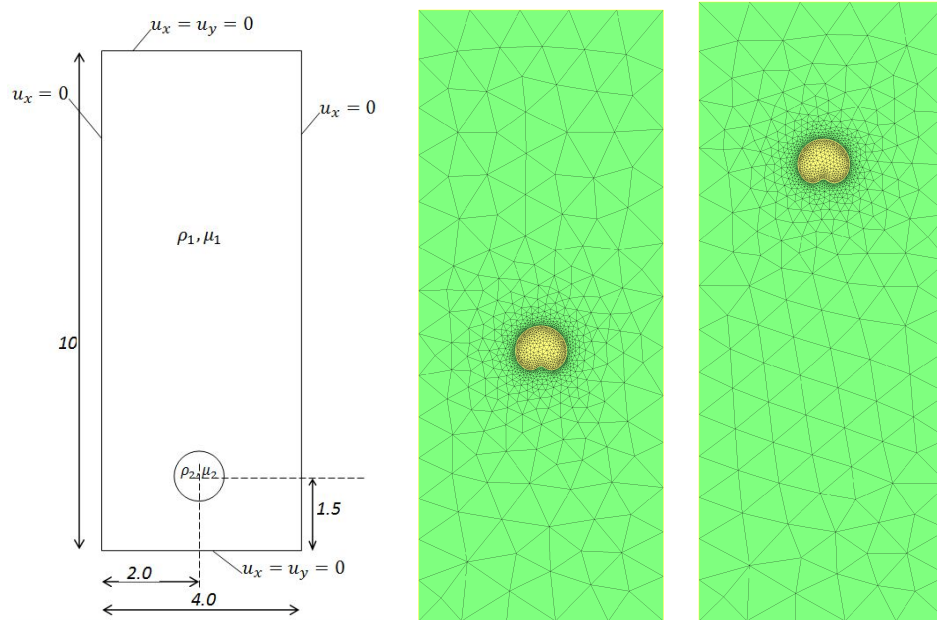
Figure 4.6: Rising bubble in 2D: initialisation (left) and evolution in time: t = 5.0s (center), t = 10.0s (right).
