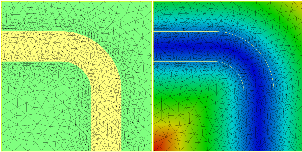
Figure 5.2: Left: explicit discretisation of shape \Omega (yellow zone) in mesh of computational domain D . Right: representation of shape \Omega as negative subdomain of a level set function defined on D
