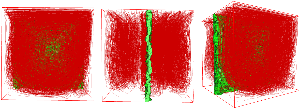
Figure 1.5: Cavity in 3D: the streamtraces for the test case Re = 1000 .
