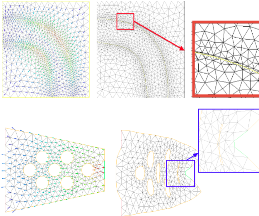
Figure 3: Illustration for the cases of ill-shaped mesh (top) and invalid mesh (bottom): (left) A velocity field V , defined at the vertices of a mesh; (right) deformed mesh.
