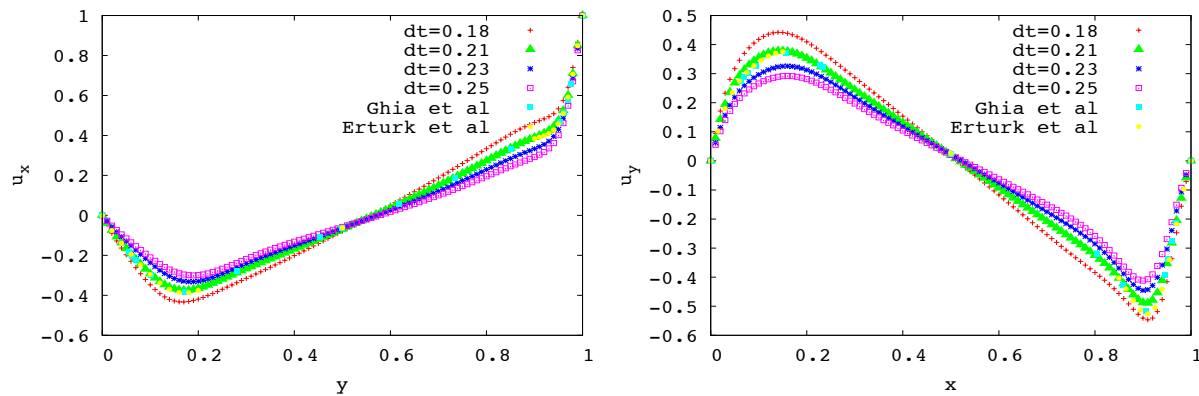
Figure 1.3: Cavity in 2D: velocity profile for u_x and u_y in case of Re = 1000 with the different time steps.
