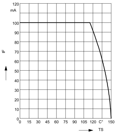
Forward current I_F = f(T_S) BAR50-03W
