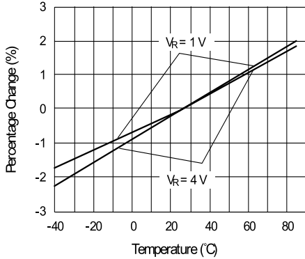
Relative Capacitance Change vs. Temperature
