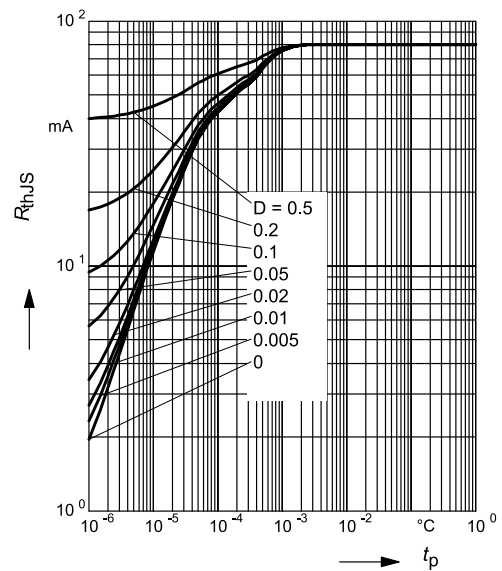
Permissible Pulse Load R_{thJS} = f(t_p) BAR50-02L
