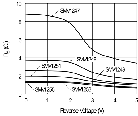
Series Resistance vs. Reverse Voltage @500 MHz
