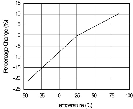
Relative Series Resistance Change vs. Temperature @500 MHz
