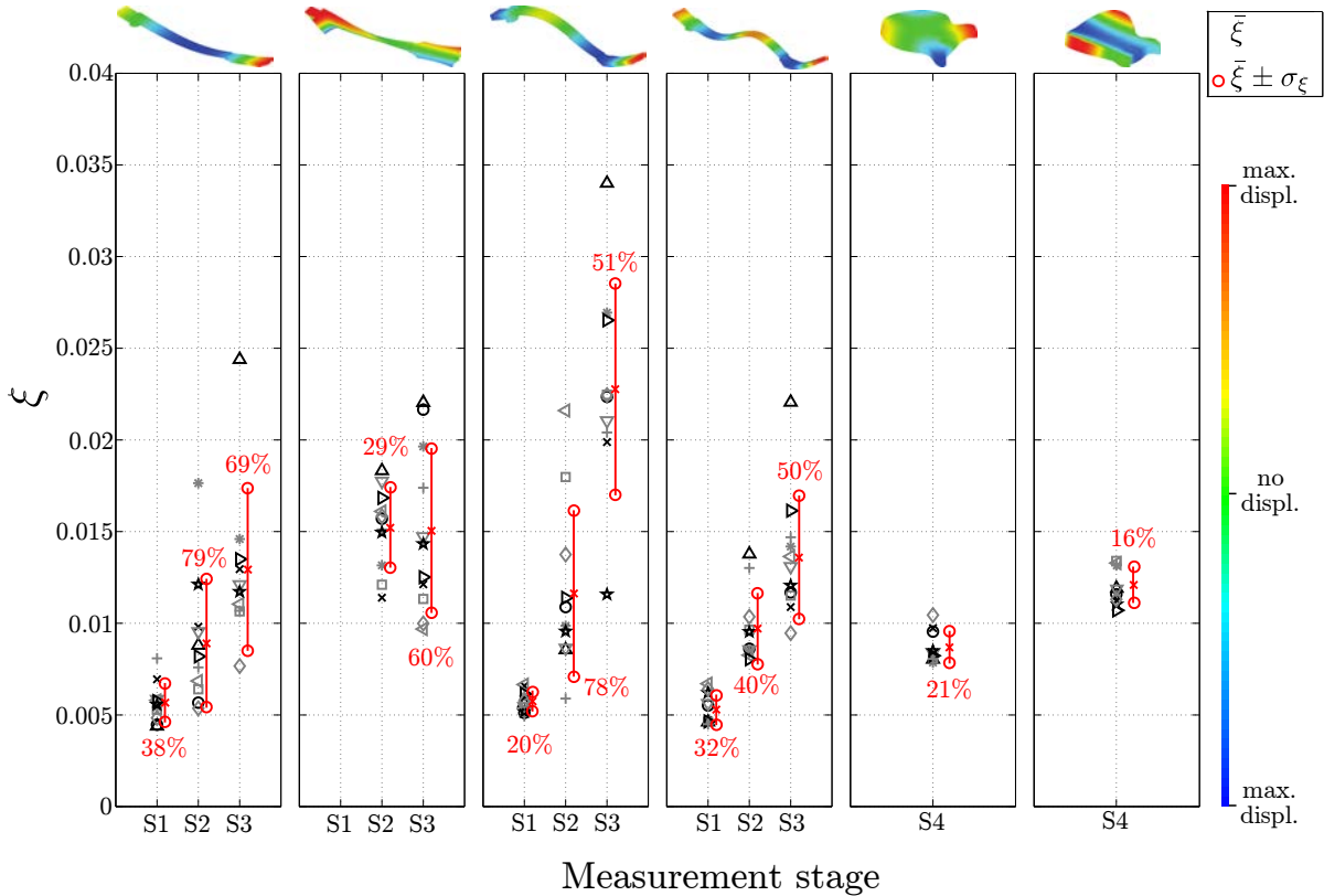
Figure 9.6: Modal damping tracking for the separated necks and bodies. Various black and gray markers are used for the individual objects. Red crosses indicate the mean value \bar{\xi} , red circles indicate the 2 standard deviation-large region centered on the mean values. For each mode, the normalised variability 2\sigma_\xi/\bar{\xi} is indicated as a percentage of \bar{\xi} . The mode shapes are shown above the corresponding modes.
