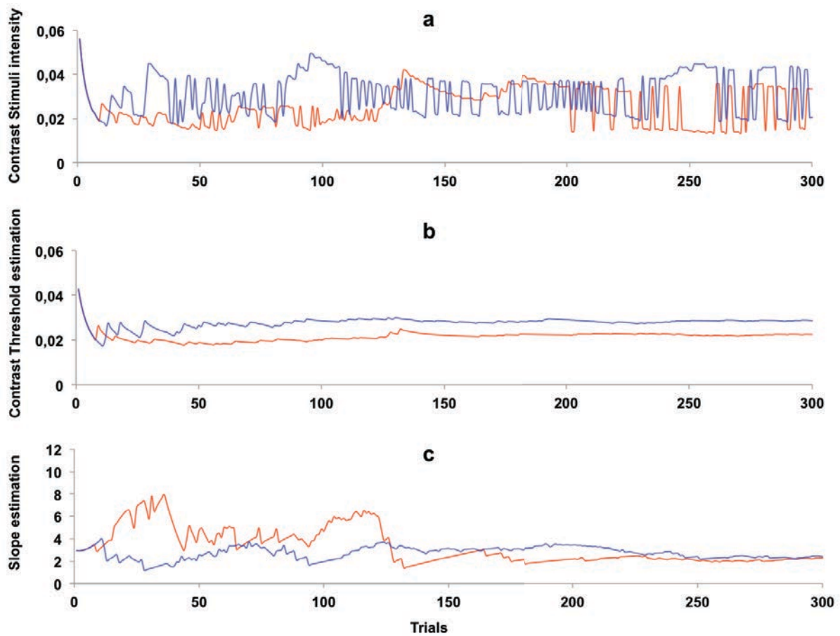
FIGURE 2. ALGORITHMIC PROCEDURE EMPLOYED TO ESTIMATE THE CONTRAST SENSITIVITY FUNCTIONS FOR THE DIFFERENT TMS MODALITIES AND FEF PATTERN CONDITIONS OF THE STUDY.
