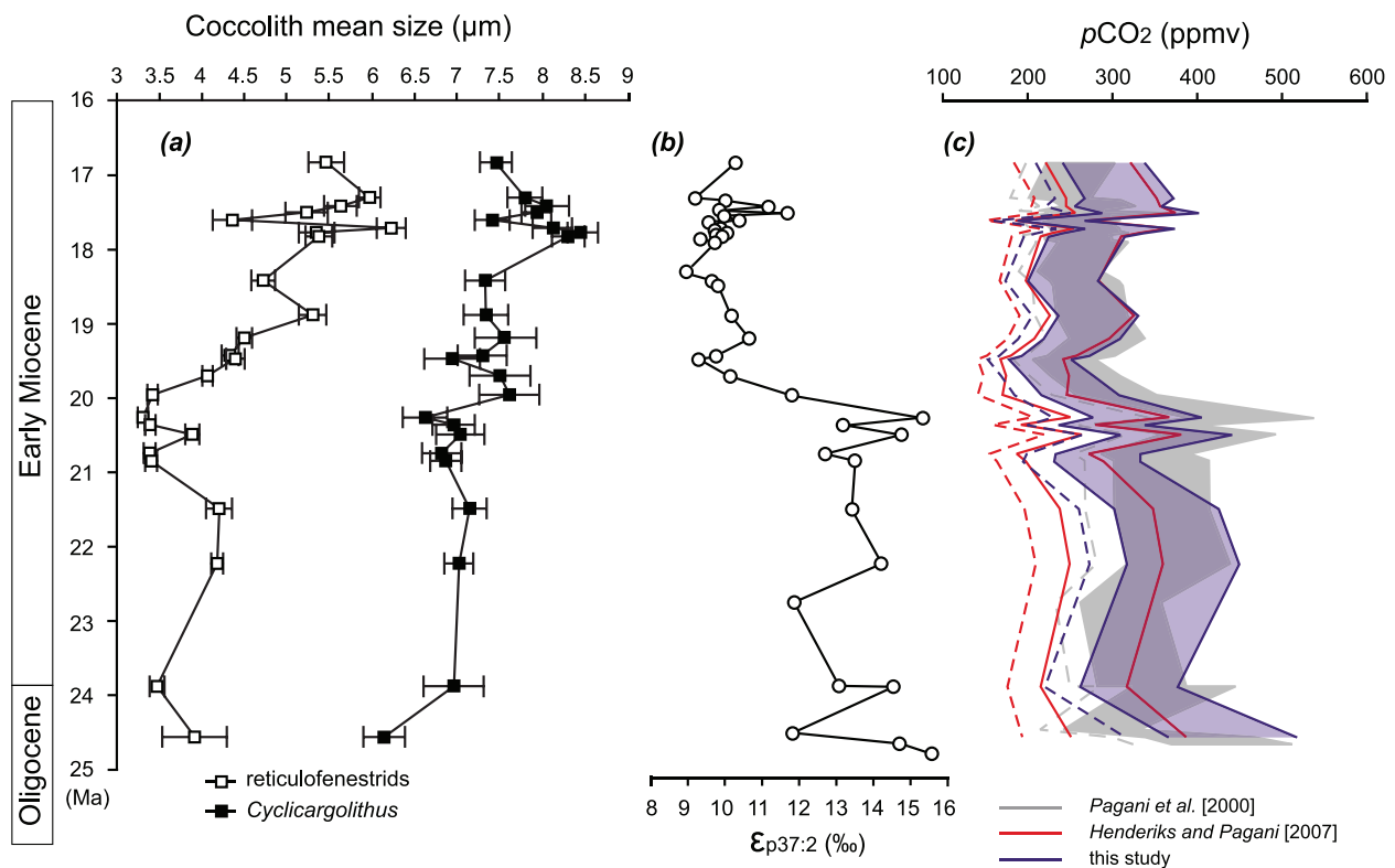
Figure 6. (a) Mean size variability at Site 516 of reticulofenestrads ( Reticulofenestra plus Dictyococcites ) and Cyclicargolithus , as determined in the 24 samples studied by Henderiks and Pagani [2007] (error bars indicate 95% confidence intervals); (b) alkenone-derived \epsilon_{p37:2} record [from Pagani et al. , 2000b]; (c) revised p\text{CO}_2 estimates after cell size corrections (see detailed methods in work by Henderiks and Pagani [2007]) including Cyclicargolithus (blue) compared to p\text{CO}_2 estimates of Pagani et al. [2000b] (grey) and Henderiks and Pagani [2007] (red). Shaded bands and lines depict minimum and maximum estimates with propagated 95% confidence levels of input factors. Dashed lines represent minimum estimates assuming no diagenetic alteration of biogenic carbonates used to determine paleo-SST [see Pagani et al. , 2005].
