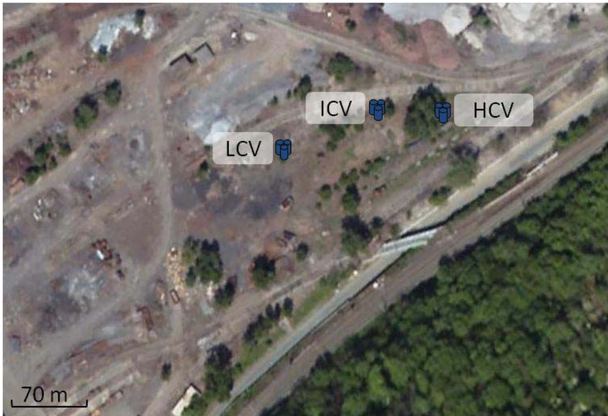
Figure 26: Localization of the microcosms on the plots of the SHSE site. LCV: low level of cover vegetation, ICV: intermediate level of cover vegetation, HCV: high level of cover vegetation. A blue cylinder represents a microcosm.
