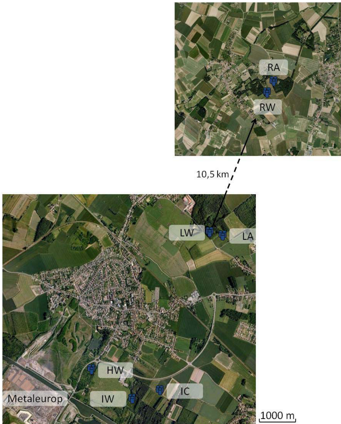
Figure 28: Localization of the microcosms on the plots of the Metaleurop site. R: reference, L: low metal contamination, I: intermediate metal contamination, H: high metal contamination, W: woodland, A: arable. A blue cylinder represents a microcosm.
