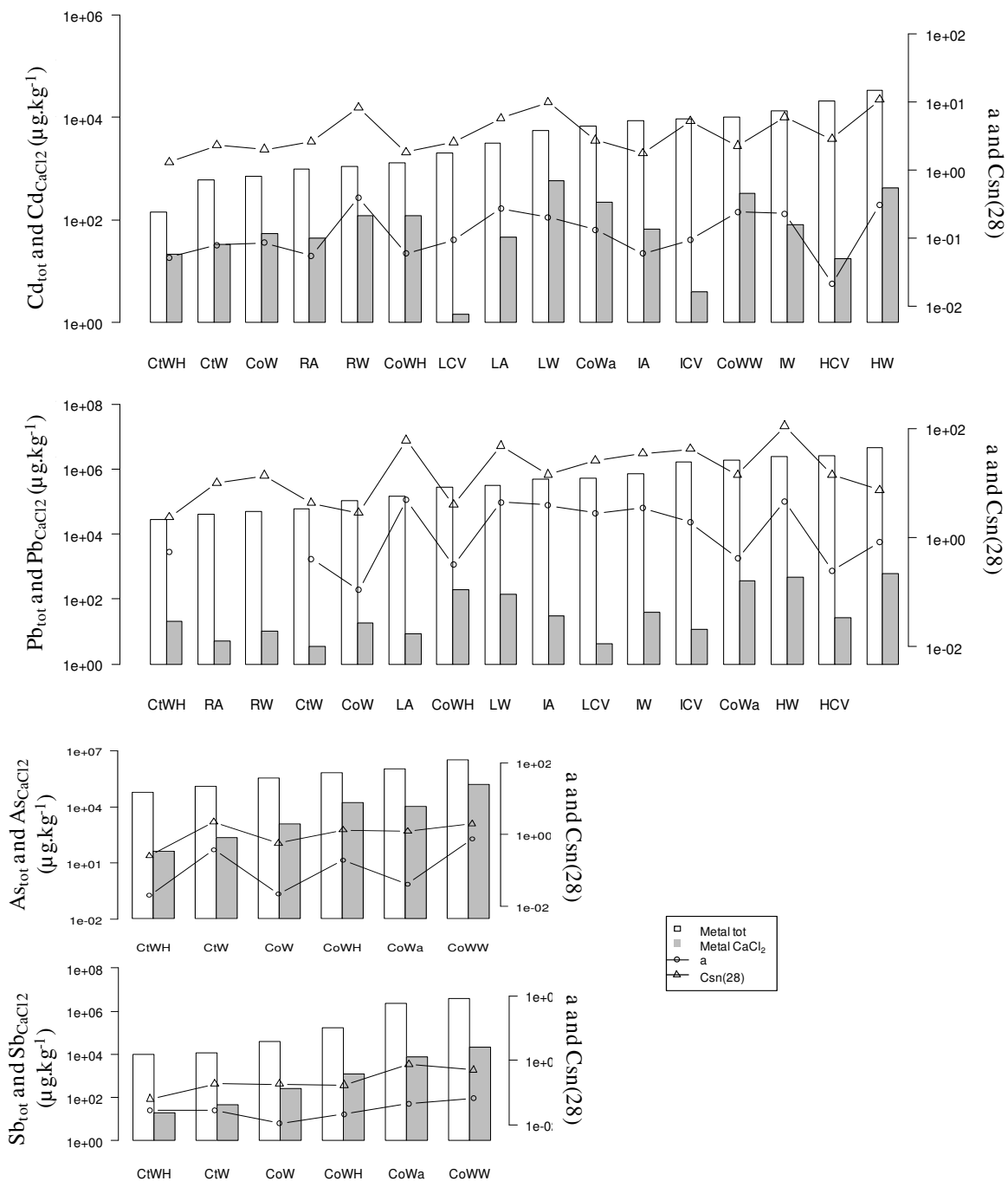
Figure 35: Comparison of accumulation in snail viscera after 28 days of exposure ( C_{\text{sn}}(28) ) and assimilation flux (a) with total soil metal concentration and \text{CaCl}_2 -extracted metal concentration of Cd and Pb and of accumulation in snail viscera after 28 days of exposure ( C_{\text{sn}}(28) ) and assimilation flux (a) to total soil metal concentrations of As and Sb.
