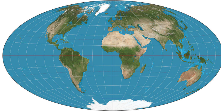
Figure 1.8 – Hammer projection.
