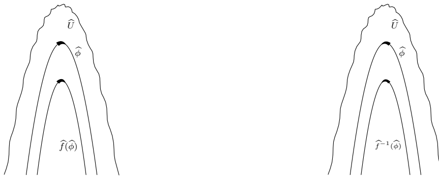
Figure 3.1: Each component \widehat{U} of \widehat{M} \setminus \widehat{K} is invariant by \widehat{f}
