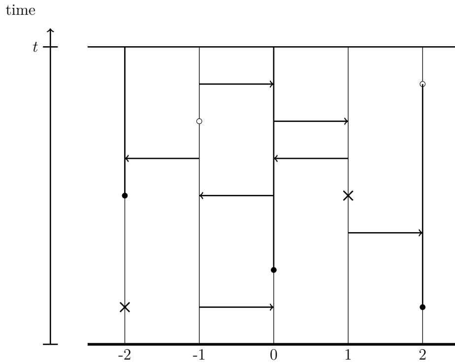
FIGURE 2.1: Graphical representation in the space-time picture \mathbb{Z} \times \mathbb{R}_+ . Starting from \eta_0 = \mathbf{1}_{\{0\}} , following the arrows, if U_1^0 < \frac{\lambda_2}{\lambda_1} and U_2^0 < \frac{\lambda_2}{\lambda_1} , the wild population occupies at time t the set H_t = \{-1, 0, 1\} in the asymmetric case and the set H_t = \{-2, -1, 0, 1\} in the symmetric case.
