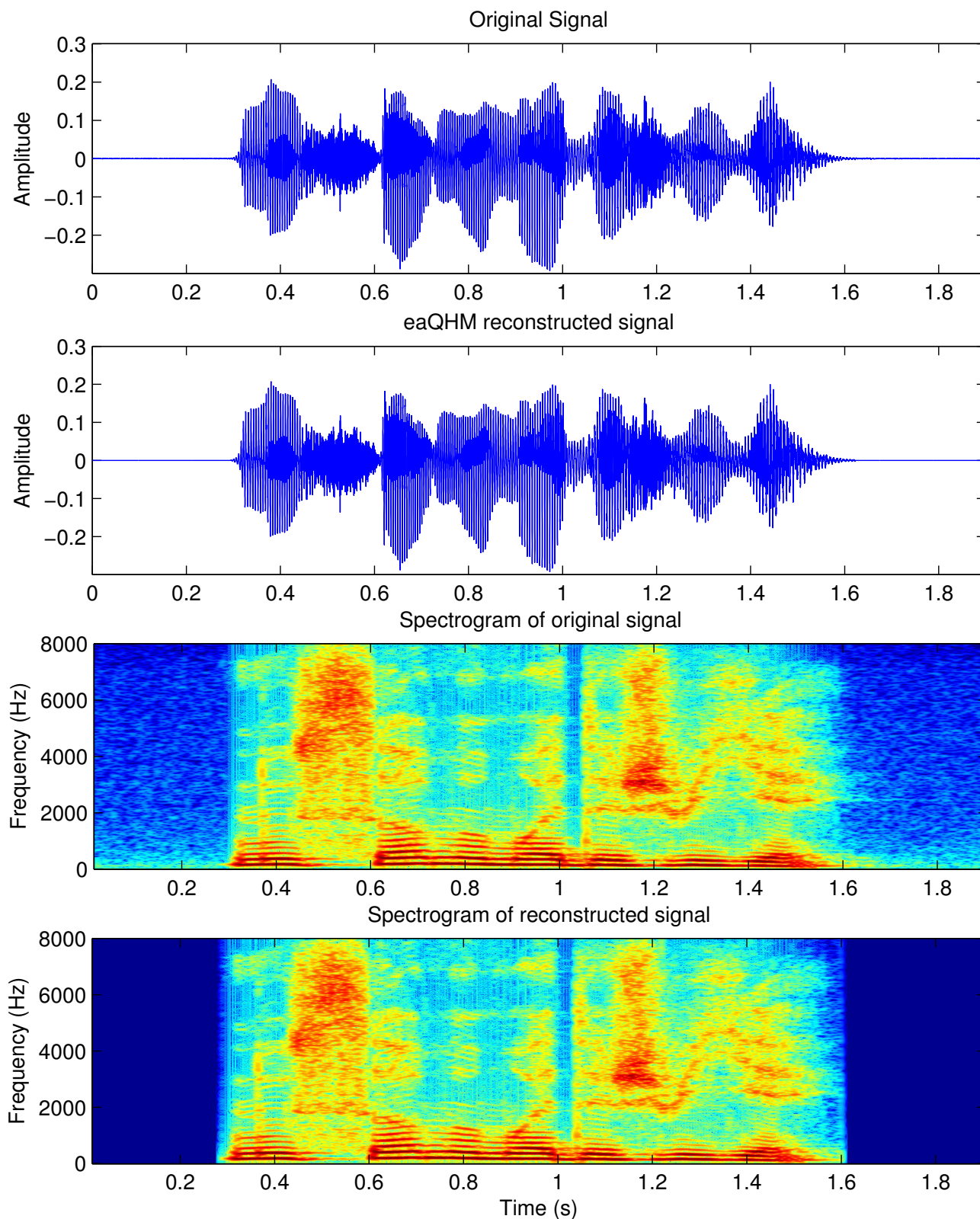
Figure 4.15: extended adaptive Quasi-Harmonic Model : Original signal (first panel) and reconstructed signal (second panel) along with their corresponding spectrograms (third and fourth panel) for a female speaker.
