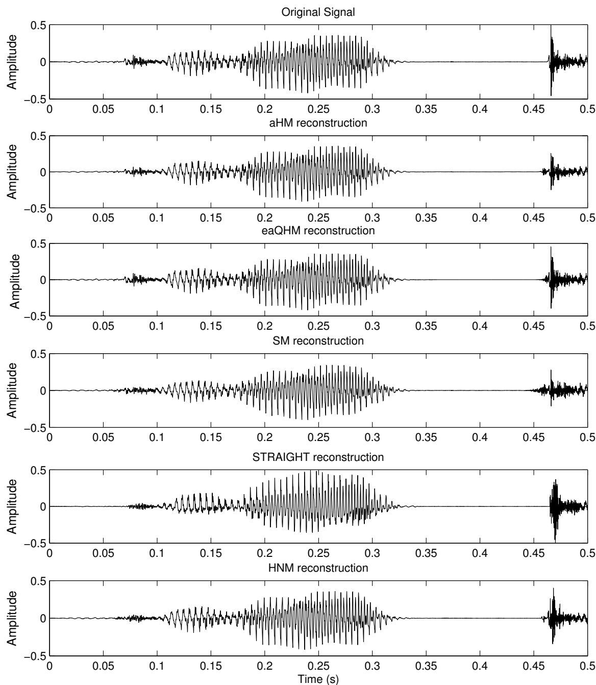
Figure 4.19: Speech utterance ( /k\tau k^h \epsilon/ ) in Korean language by a female subject. First panel: Original signal, Second panel: aHM reconstruction, Third panel: eaQHM reconstruction, Fourth panel: SM reconstruction, Fifth panel: STRAIGHT reconstruction, Sixth panel: HNM reconstruction.
