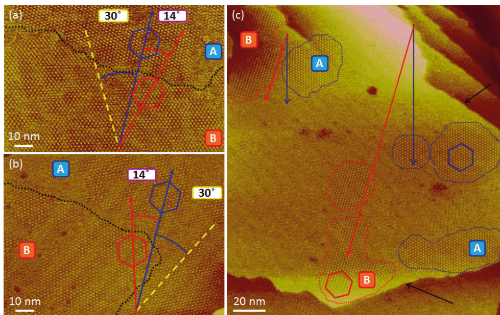
Figure 3.5 STM images of twofold orientation of H5T molecules self-assembled at the n -tetradecane/Au(111) interface. (7 × 7) domains (A) and (\sqrt{52} \times \sqrt{52})R13.9^\circ domains (B) are depicted by blue and red graphics, respectively. Yellow dashed-lines at (a) and (b) highlight the main direction of Au(111) reconstruction, black dotted-lines at (a) and (b) highlight the domain boundaries. (a) and (b) STM pictures are taken on the same Au(111) monocrystal and evidence the two possible orientations of (B) domains, rotated by \pm 13.9^\circ from the (A) ones. Black arrows at (c) show the steppedges of Au(111) substrate; I_t = 10 pA, V_t = 100 mV.
