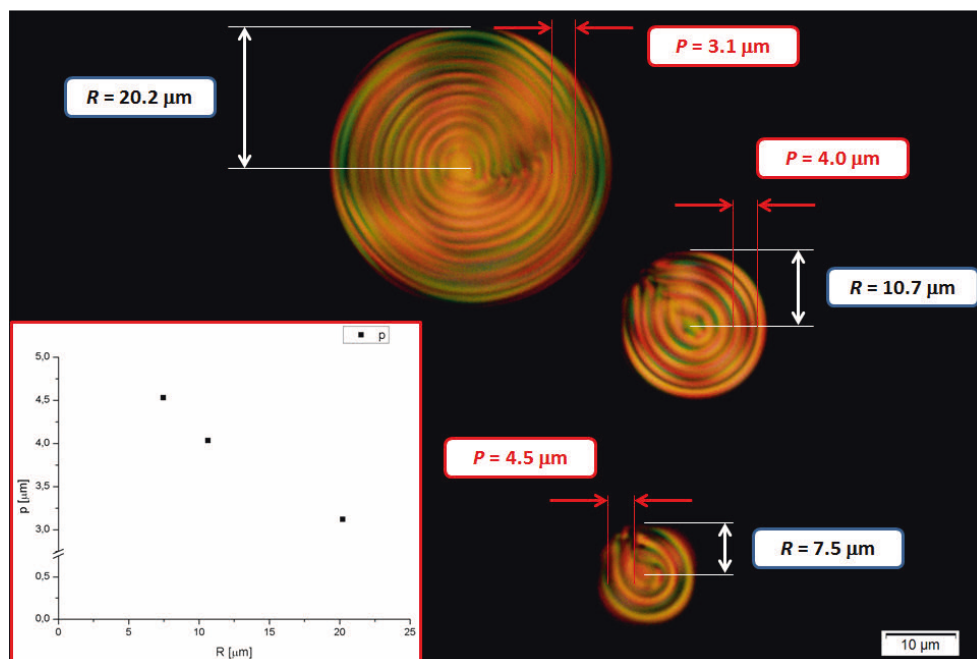
Figure 7.6 Polarized microscopy images of 1b/E7 droplets. The three radial spherical droplets show an increase in the value of radial period as the droplet size decreases. The tendency is shown by the P vs R plot ( inset ).
