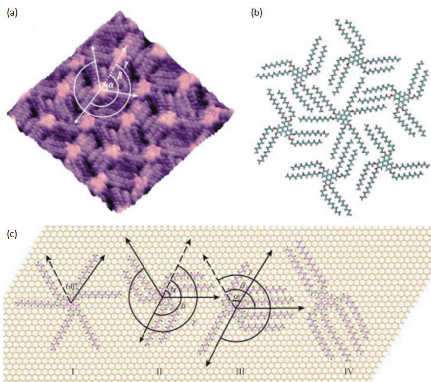
Figure 2.13 (a) High-resolution STM image ( 10 \times 10 \text{ nm}^2 ) of a H12T monolayer on HOPG and (b) the respective molecular packing model (from Ref. 111). (c) Schematic representation of 4 different molecular conformations corresponding to: H12T (I and II), H14T (III) and H16T and higher order derivatives (IV). Both triphenylene cores and alkoxy chains are commensurate with the HOPG lattice. Solid arrows represent orientations of flexible tails and dashed ones the midline of the triangle formed by aromatic core (from Ref. 111).
