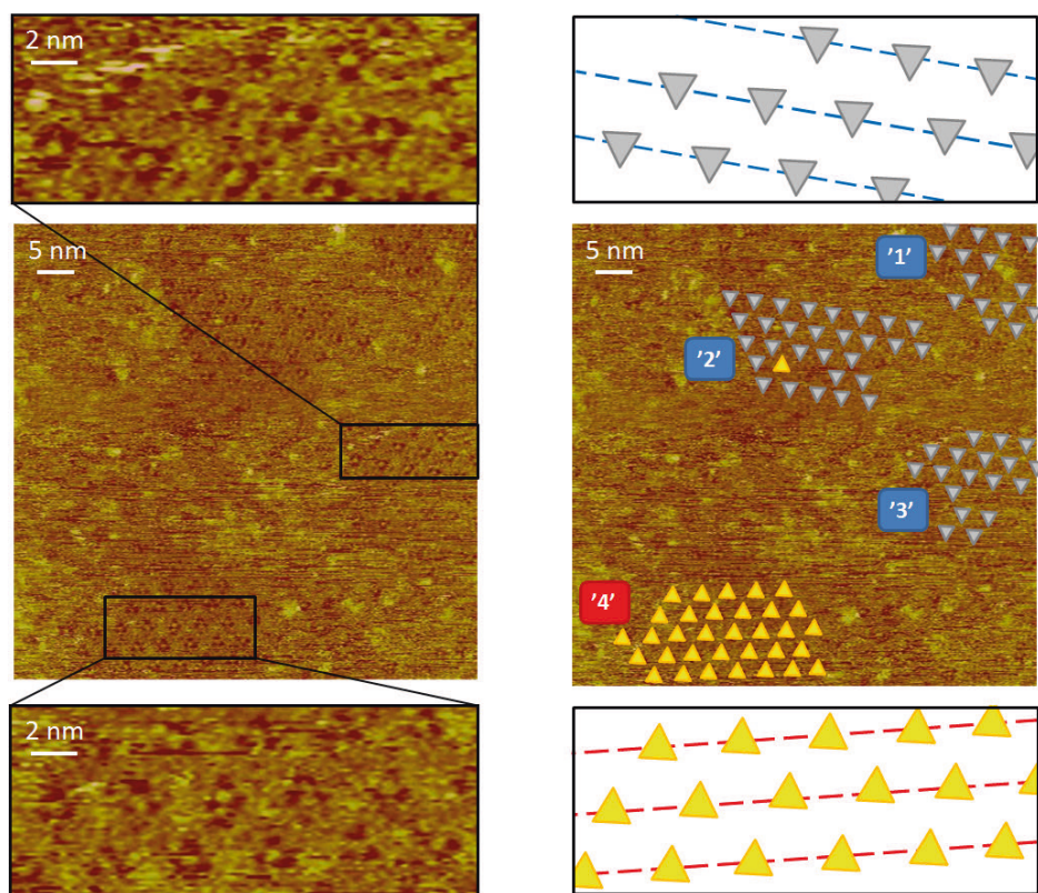
Figure 5.6 (left) STM constant current images showing peculiar triangular contrast that originate from the double-bonded oxygen group of ester linker. Top and bottom close-ups show domains with 'all-down' and 'all-up' positions of physisorbed molecules, respectively. (right) The same image with grey and yellow triangles superimposed in the lattice nodes of each domain according to tunneling contrast. The insets show the respective packing of C-12 molecules in domains '3' and '4'; I_t = 15 \text{ pA} , V_t = 250 \text{ mV} .
