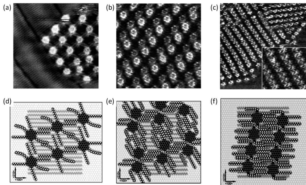
Figure 2.18 (a) STM image ( 18.7 \times 18.7 \text{ nm}^2 ) showing an HBC- C_{12} island having the \alpha -phase adsorbed on top of the \{n - C_{50}H_{102} monolayer/graphite \} system. (b) STM image ( 23.1 \times 23.1 \text{ nm}^2 ) of \beta -phase (dimer structure) on top of the n - C_{50}H_{102} monolayer. Two molecules within the dimer are not equivalent and have different STM contrast. Dodecyl chains of HBC- C_{12} occupy the space between the dimers and are aligned along preferential directions. (c) STM image ( 37 \times 37 \text{ nm}^2 ) of the final \gamma -phase with a row structure. HBC- C_{12} cores form parallel rows on top of the n - C_{50}H_{102} template. Inset shows details of packing ( 12 \times 12 \text{ nm}^2 ). Images (d), (e) and (f) represent possible packing model of the \alpha -, \beta -, and \gamma -phase, respectively. On (d), (e) and (f) n - C_{50}H_{102} molecules are depicted by gray zigzag lines on top of hexagonal graphite lattice (from Ref. 123).
