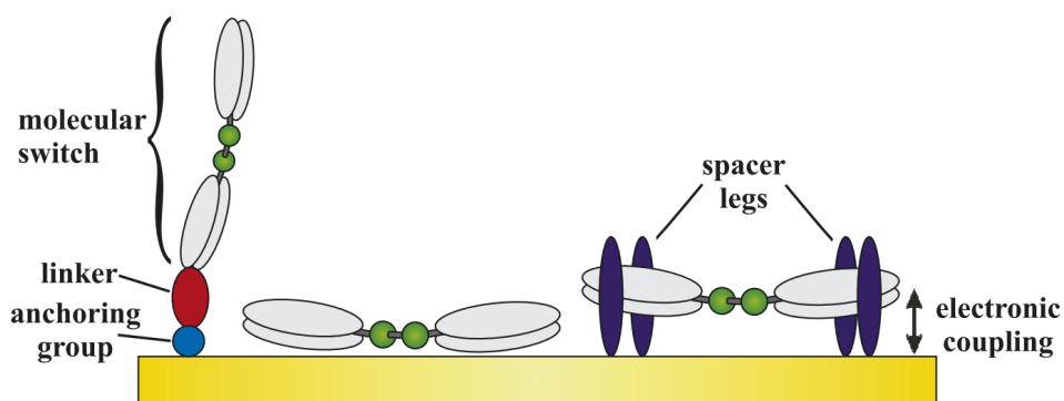
Figure 4.1 Adsorption of molecular switches via an anchoring group, leading to a vertical orientation and physisorbed systems in which the molecules are in direct contact with the substrate. Spacer groups yield a reduced electronic coupling between the molecules and the substrate (from Ref. 9).
