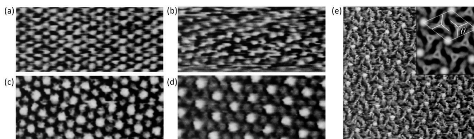
Figure 2.12 STM images ( 29 \times 13 \text{ nm}^2 ) of single domains of H n T monolayers, at the interface between the graphite and n -tetradecane solutions. (a) H5T, (b) H7T, (c) H9T and (d) H11T. (e) High-resolution STM image ( 29 \times 28 \text{ nm}^2 ) of H11T monolayer. The inset shows the corresponding symmetrized correlation averaged image together with the unit cell (from Ref. 107).
