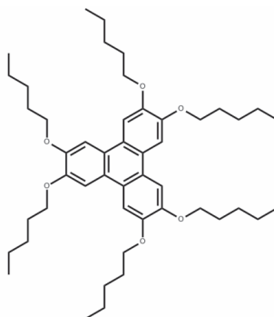
Figure 3.1 Chemical structure of investigated 2,3,6,7,10,11-hexapentylxytriphenylene (H5T), a molecule belonging to the D_{3h} point-symmetry group and a classical example of discotic liquid crystal.
