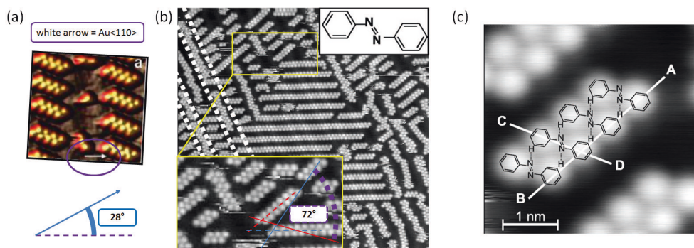
Figure 4.13 STM images of azobenzene molecules self-assembled on Au(111). (a) Supramolecular tetramers of bare azobenzene physisorbed on Au(111). The blue arrow points the direction of orientation of a single azobenzene, which is rotated by ca 28° with respect to white arrow which symbolizes Au<110> direction (from Ref. 21). (b) STM images of 0.50 monolayer coverage of azobenzene on Au(111). The inset (yellow) shows mutual rotation of azobenzenes within two types of aggregates (blue/red), equal 72°. (c) Close-up STM image of a short chain of azobenzene molecules confined by the Au(111) substrate (from Ref. 33).
