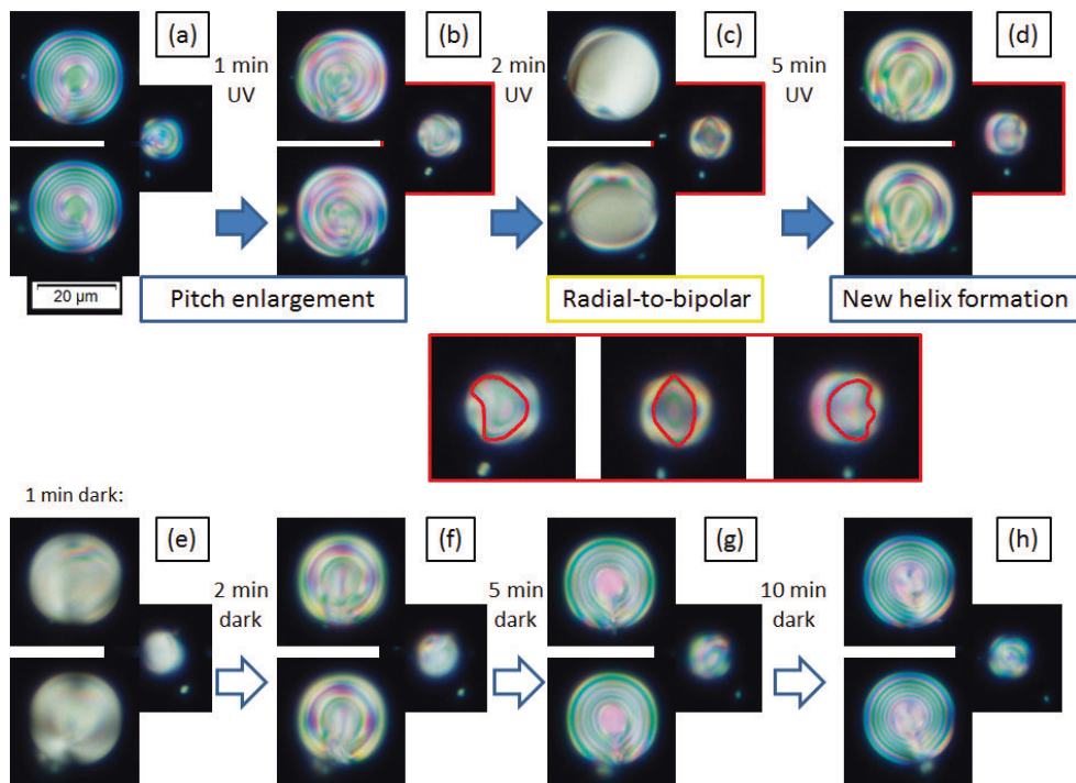
Figure 7.12 Sequence of polarized microscopy patterns (transmission mode) showing the evolution of textures of three droplets ( 1b ) under the irradiation with UV. The two droplets on the left part of each panel have similar radius equal 11.9 \mu\text{m} and the smaller droplet has radius equal 5.6 \mu\text{m} .
