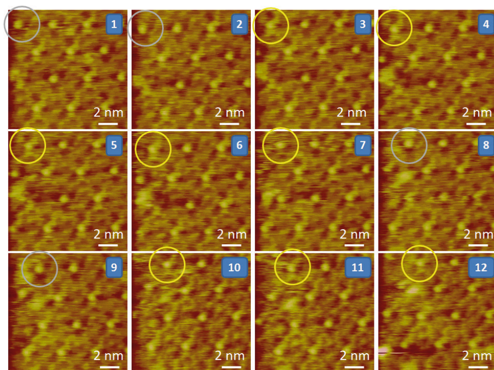
Figure 5.2 Sequence of STM images showing the multiple 'up'/'down' contrast change of a single molecule of C-12; I_t = 9 pA, V_t = 220 mV. Grey circles correspond to the 'down' state whereas yellow circles highlight the 'up' state.
