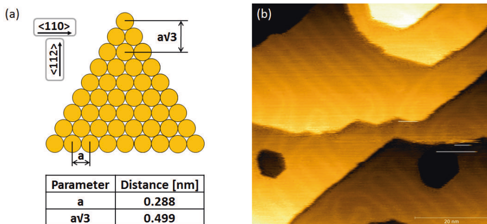
Figure 2.8 (a) Hard-sphere representation of non-reconstructed Au(111) surface with indicated crystallographic directions and distance parameters. (b) UHV-STM constant current image showing several terraces of bare, reconstructed Au(111) surface. Bright linear features that always go in pairs represent the relaxation of the surface of gold. The sample has been flame annealed in propane gas flame in ambient conditions, prior to the transfer into the STM chamber. I_t = 40 pA, V_t = 500 mV.
