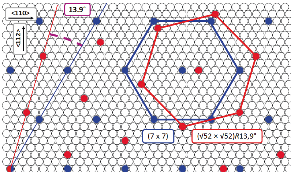
Figure 3.6 Proposed model of packing of molecular centers of HST species at a n -tetradecane/Au(111) interface for (7 \times 7) and (\sqrt{52} \times \sqrt{52})R13.9^\circ domains, indicated by blue- and red-color mesh, respectively. The two models correspond to the experimental data obtained with the assumption of the commensurability of the system.
