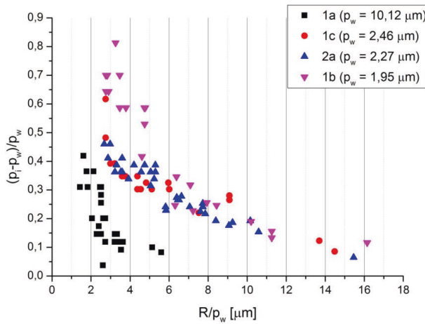
Figure 7.8 Relative period change (P-P_w)/P_w vs R/P_w for the different P_w values. One should notice that the black squares that represent the CLC mixture of low dopant concentration enables to access the radial structure for the relatively lower size, considering the geometrical confinement.
