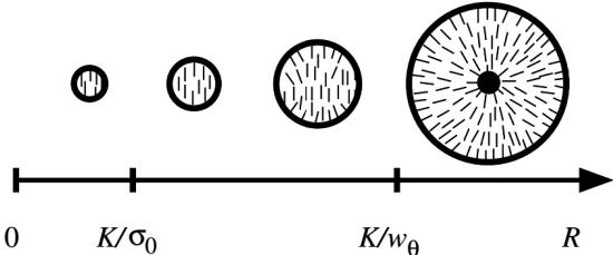
Figure 6.7 Schematic representation director configurations of nematic droplets with normal surface anchoring. While for small droplets ( R \ll K/w_\theta ) the director orientation tends to be uniform, large droplets ( R \gg K/w_\theta ) in ground state contain topological defects - here depicted by the black spot in the center of a droplet (from Ref. 12).
