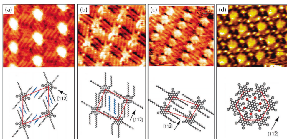
Figure 2.20 STM images ( 10 \times 9 \text{ nm}^2 ) and corresponding models of molecular packing of various phases of HBC- C_{12} at n -tetradecane/Au(111) interface. (a) The kinetically controlled \alpha -network that undergoes phase transition into \beta -phase, shown on (b). The gray circles represent out-of-plane n -dodecyl chains. Co-adsorbed n -tetradecane molecules appear in blue. (c) The following phase transition \beta \rightarrow \gamma is connected with unidirectional adsorption of peripheral C_{12} -tails and lack of the co-adsorption of solvent molecules. (d) The most compacted and thermodynamically stable \delta -phase, none of the alkyl tails are physisorbed on the substrate, and the solely repetitive units are the central HBC-moieties. The arrows indicate the \langle 112 \rangle direction of gold (from Ref. 130).
