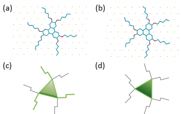
Figure 3.10 (a) and (b) represent two orientations of minimized energy H5T molecule on Au(111) : 14^\circ and 30^\circ -rotated, associated with (7 \times 7) and (\sqrt{52} \times \sqrt{52})R13.9^\circ structures, respectively. Green features on (c) and (d) emphasize the input into adsorption energy for corresponding configurations. What should be noticed is the diversification of interactions in the case of 14^\circ -rotated molecule, where both core and tails greatly contribute, contrary to the concentric character for the 30^\circ -rotated one.
