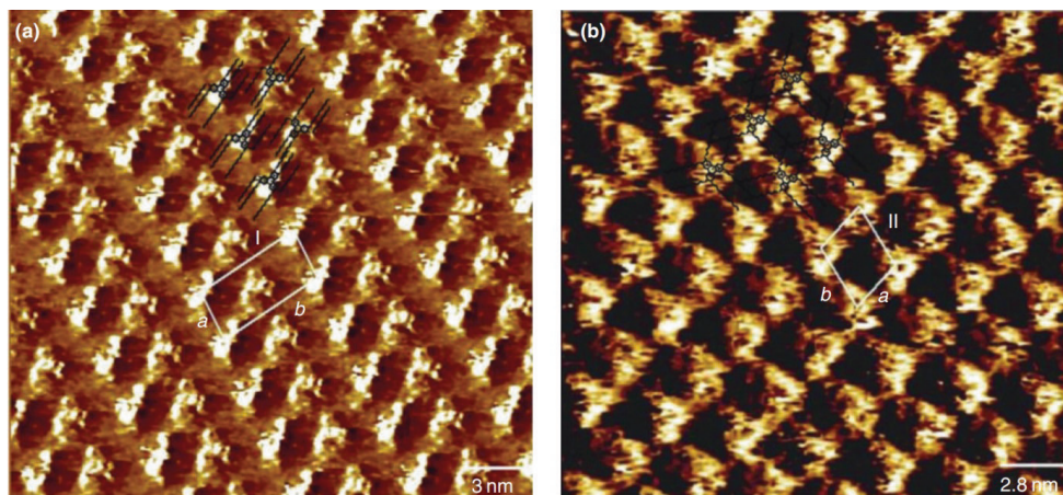
Figure 2.15 STM images of HDTT recorded at the interface between HOPG and a solution in (a) phenyl octane or (b) n -tetradecane. While in the case of phenyl octane antiparallel orientation of molecules may be remarked and associated dimer formation, such behavior is not encountered when the n -tetradecane is used as a solvent (from Ref. 115).
