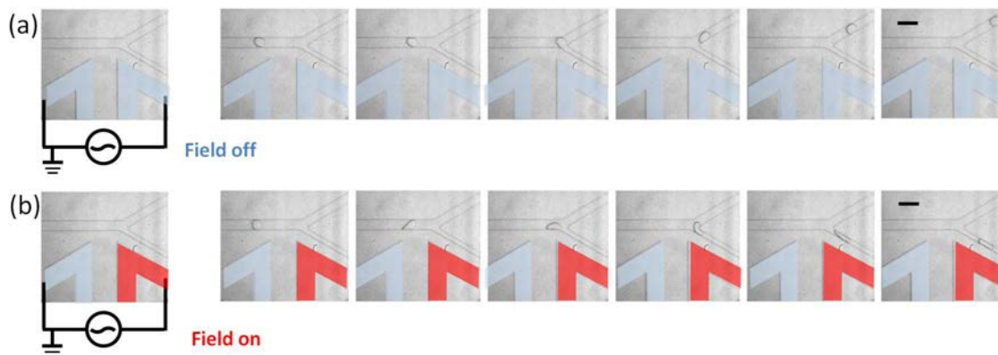
Figure 2.8: (a) When the electric field is switched off, droplet flows along the upper channel because of low flow resistance. (b) When the electric field is switched on, the droplet is driven in the the lower channel of the branch. Scale bar is 30 \mu\text{m} . The artificial added color is used to indicate the different states of electrodes.
