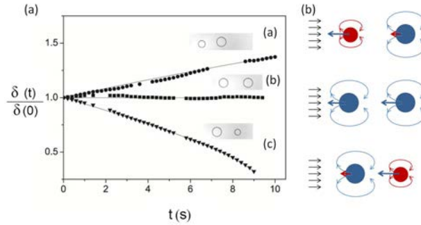
Figure 3.7: (a) Evolution of the distance between droplets as a function of time. Solid lines depict the theoretical model using an adjustment of the parameter \Delta\beta = \beta_2 - \beta_1 . PDMS system, h = 48 \mu\text{m} , w_2 = 3000 \mu\text{m} . (a): R_2 = 209 \mu\text{m} , R_1 = 155 \mu\text{m} , \Delta\beta = 0.0055 . (b): R_2 = 206 \mu\text{m} , R_1 = 201 \mu\text{m} . (c): R_2 = 131 \mu\text{m} , R_1 = 205 \mu\text{m} , \Delta\beta = -0.0157 . For identical droplets (case (b)), theory predicts that their separation remains constant (horizontal solid line). (b) Representation of the recirculations generated by each droplet in those three different cases. Forces generated by each droplet are represented by arrows of the droplet color.
