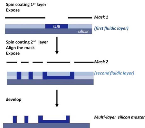
Figure 2.3: Double layer fabrication process. The multilayer structures are constructed through layer by layer exposition and alignment operations.
