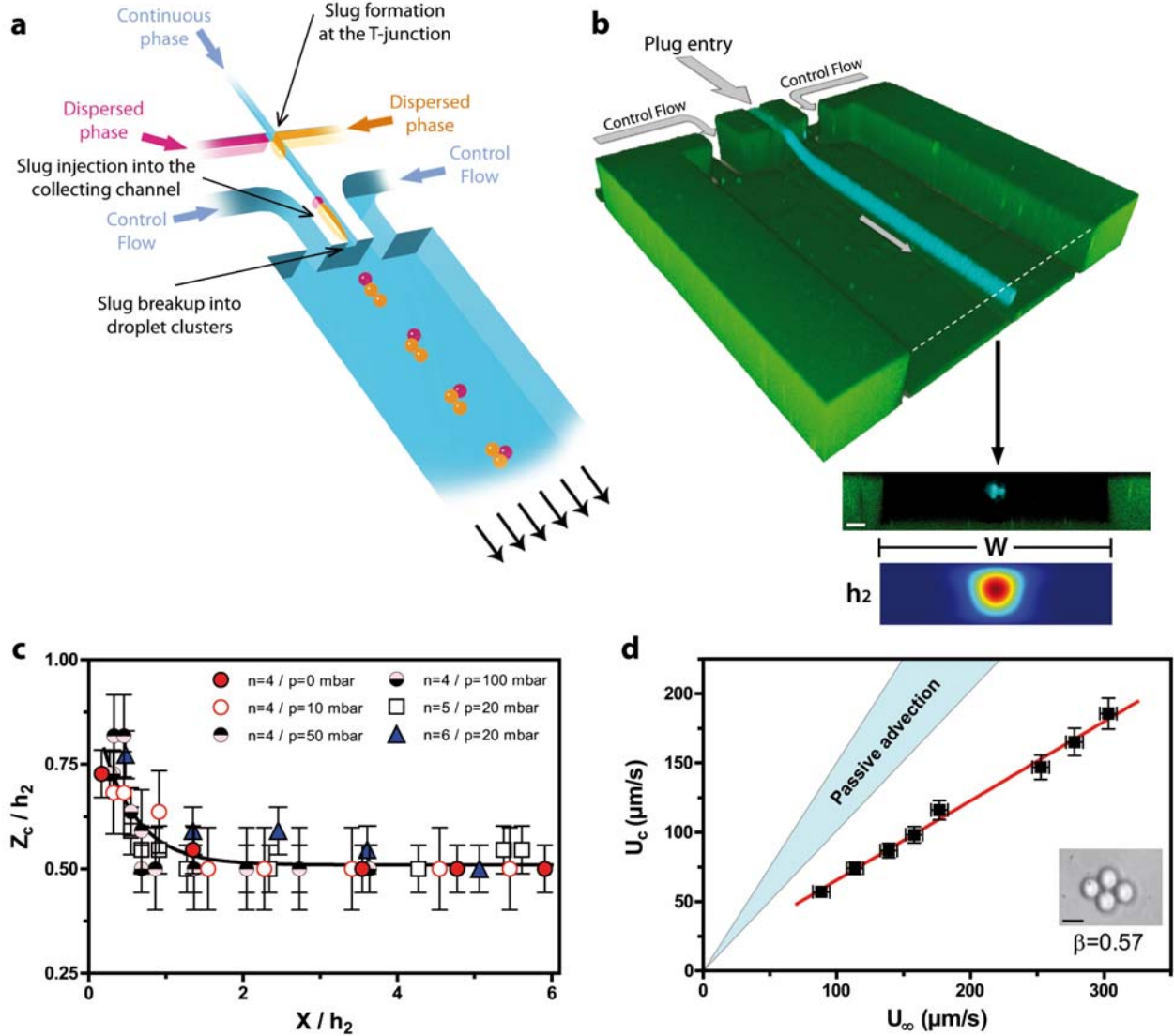
Figure 1 : Sketch of the device, flow structure and droplet positioning in the SA channel. (a) Sketch of the two-level microfluidic device. In the thinner part, located upstream, slug pairs (red and orange) are generated, and arrive at a step where they breakup into sticky droplets, forming clusters that are processed and conveyed downstream in the (deeper) SA channel. (b) Confocal image of the system, taken over long exposure times, that reveal that the clusters are confined in a tube whose center is located close to the mid plane of the SA channel and comparison with COMSOL simulations (see Supp Mat 3), that show that the flows emanating from the central inlet are confined in a tube, also located close to the SA channel symmetry axis. (c) Cluster position measurement using Adaptive Focus. Cluster position along the z axis, normal to the mean flow, normalized by the SA channel height h_2 as a function of the distance to the step x normalized in the same manner. The plot shows that, within the range of experimental conditions we considered, and after a short transient, that does not exceed two SA channel heights, the planar clusters self-center in the SA channel. All the experiments are performed in PDMS system, with h_1=1 \mu\text{m} , h_2=10 \mu\text{m} and d = 5 \mu\text{m} using fluorinated oil, water and 2 % SDS. (d) Dumbbell speed U_c as a function of the
