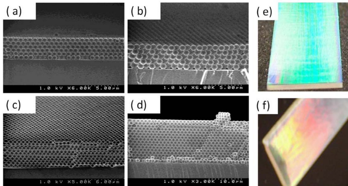
Figure 1.2: Representative SEM images of the cross sections of the silica colloidal crystal films produced by IHEISA using (a) and (c) 635 nm, (b) 850 nm, and (d) 1 \mu\text{m} spheres. (e) Photographs of the colloidal crystal films made out of 650 nm silica spheres deposited by IDEISA onto a glass slide support. (f) The films made out of 850 nm silica spheres. Images adapted from ref [10].
