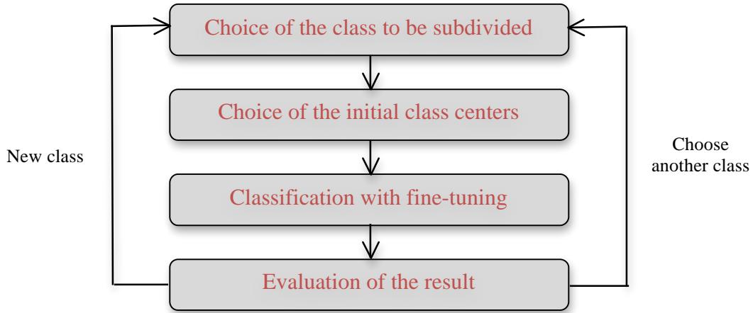
Figure 4.1: The general layout of the developed unsupervised classification approach
