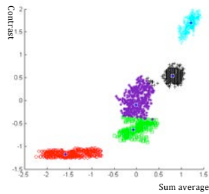
(c) FCM result, ACCR: 98.08%
