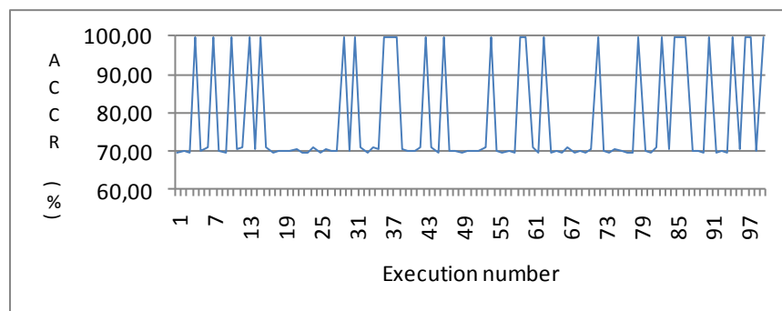
(a) LBG
