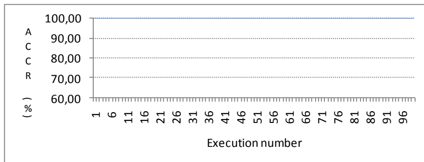
(b) AILBG
