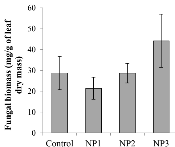
Figure 4: Fungal biomass on alder leaves incubated in microcosms exposed to CeO 2 NPs (mean values ± standard error).
