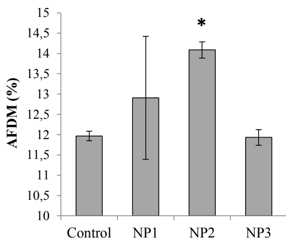
Figure 3: Remaining organic matter from leaf litter incubated in microcosms exposed to CeO 2 NPs (mean values ± standard error).
