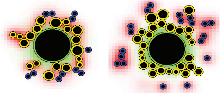
Figure 2.13: Typical structure of an erythroblastic island in the simulations : Fas-ligand produced by early-stage erythroblasts (left) or by late-stage erythroblasts (right). The large cell in the center is a macrophage, yellow cells - CFU-E/Pro-EBs and differentiating erythroblasts, blue - late-stage mature erythroblasts and reticulocytes, level of green - concentration of the growth factor ( G ) produced by the macrophage, level of red - concentration of Fas-ligand. Black circles inside cells show their incompressible parts.
