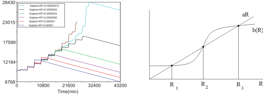
Figure 2.23: Left: number of erythrocytes in blood as a function of time for different values of feedback coefficients or without feedback (upper curve). Right: graphical solution of equation 2.2.21.
