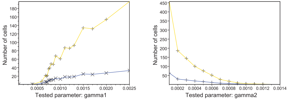
Figure 2.9: Average in time number of progenitors and reticulocytes for different values of \gamma_1 (left) and \gamma_2^0 (right) (mean values for 10 simulations).
