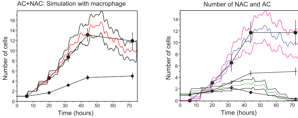
Figure 2.18: Comparison of in vitro experiments and numerical simulations with mouse cells. Left figure : the total number of erythroid cells in co-cultures (upper curve). The number erythroid cells in control cultures without macrophage (lower curve); black symbols - experiments, continuous curves - simulations. Three curves for each of the experiments represent mean value and confidence intervals for 10 simulations. Right figure : the number of cells adherent to macrophage in co-cultures (AC) - lower curve, nonadherent cells in co-cultures (NAC) - upper curve, and middle curve is control culture without macrophages. For a value of the parameters used, see Tables 3 and 4. Experimental data were originally reported in reference [124].
