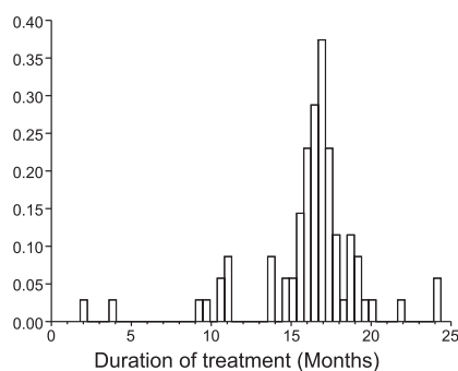
Figure 3.19: Histogram of the duration of maintenance treatment for 78 patients having T or B lymphoma.
