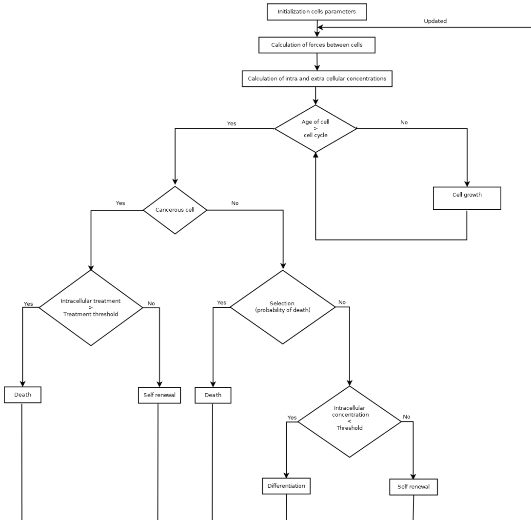
Figure 6.1: Simplification of the algorithm describing the fate of cells.
