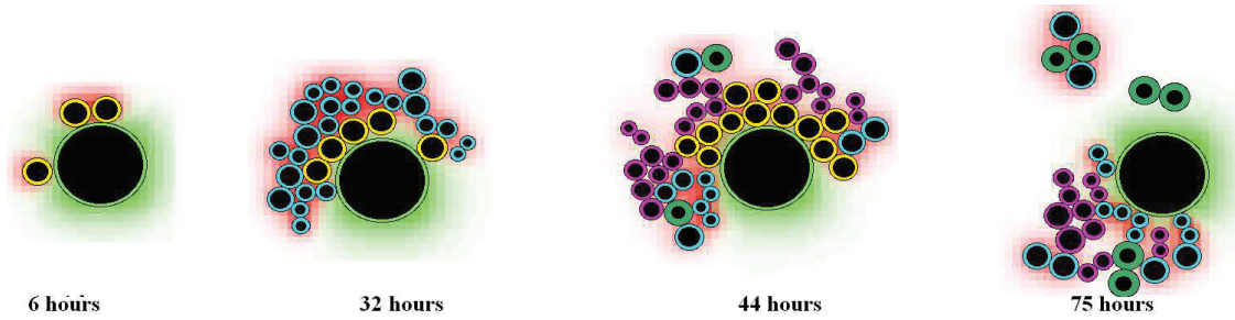
Figure 2.19: Simulation of one erythroblastic island in vitro . Large cell - macrophage, yellow cells - AC progenitors, blue - NAC progenitors, rose -NAC differentiated cells including reticulocytes, green - AC apoptotic cells. Fas-ligand is produced by early stage erythroblasts (yellow and light blue).
