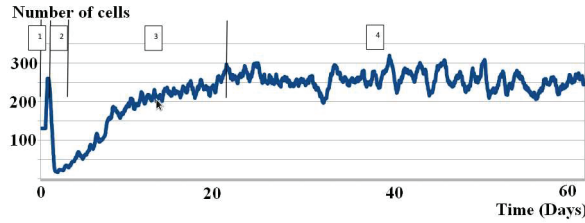
Figure 3.4: Total number of erythrocytes produced by 8 islands. After approximately 20 days it reaches a steady state level with some oscillations around it due to cell cycle.
