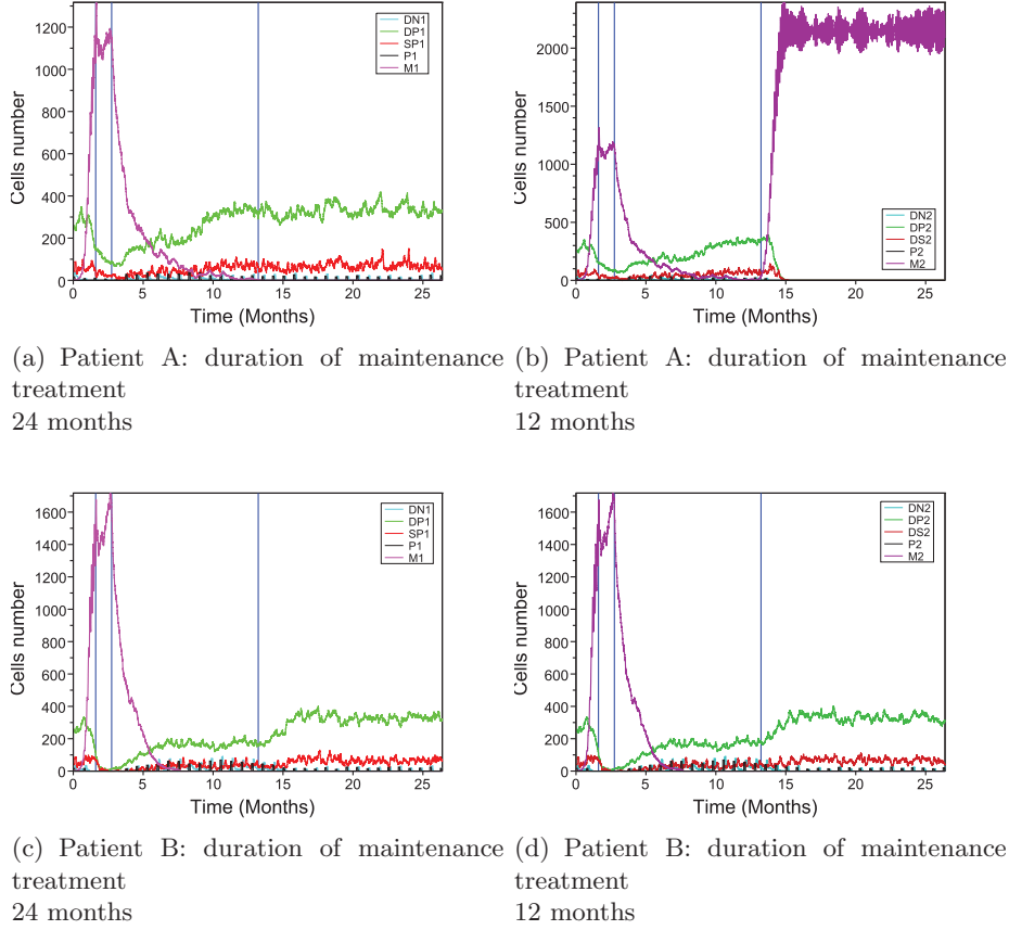
Figure 3.21: Numerical simulation of lymphoma treatment. The first vertical line shows beginning of treatment of the acute phase, the second vertical line shows the end of treatment of the acute phase and beginning the maintenance treatment, the third vertical line shows the end of maintenance treatment for the patients in figures (b) and (d). One of them relapsed. Treatment is continued for patients in figures (a) and (c). Both of them are cured.
