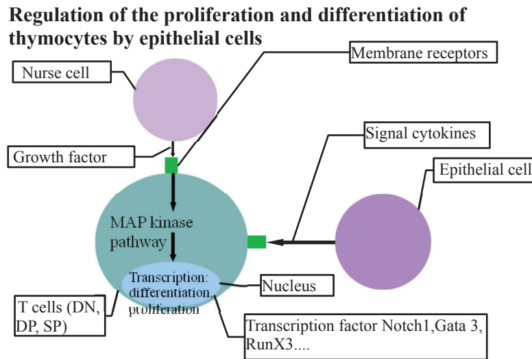
Figure 3.13: Simplified pattern of signals transduction. Each thymic cell receives signals from its microenvironnement. These signals determine the fate of cells by \beta , negative and positive selection.
