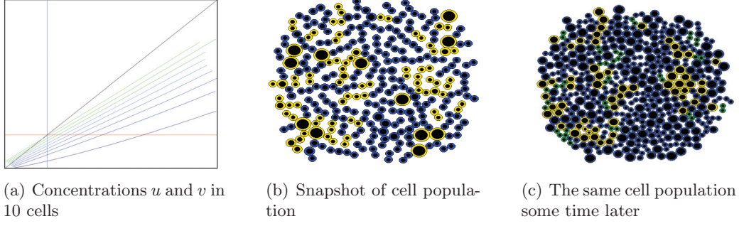
Figure 2.3: Evolution of the population of MEP cells for the values of parameters k_1^+ = 0.005 , k_1^- = 0.008 , k_2 = 0.1 , k_3^+ = 0.005 , k_3^- = 0.008 , k_4 = 0.2 . MEP cells self-renew and differentiate into BFU-E cell lineage. In Figure 2.3(a), curves of the phase space are majority located below the first bisector, there is commitment into BFU-E lineage as shown in Figure 2.1. The Figures 2.3(b) and 2.3(c) show the evolution towards BFU-E cells and gradual disappearance of self-renewal.
