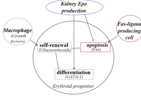
Figure 2.7: Intracellular and extracellular regulation that determine erythroid progenitor fate.
