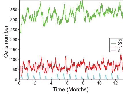
Figure 3.14: Numerical simulations of healthy thymus: a part of thymic cortex. The number of cells (DN (blue), DP (green), SP (red)) in a section of healthy thymus during one year.
