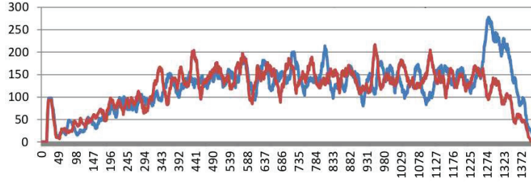
Figure 3.8: Blue curve: number of erythrocyte after injection of EPO. Red curve: number of erythrocyte without exogenous EPO.
