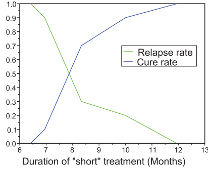
Figure 3.20: The number of relapses decreases (and number of healings increases) as a function of duration of short treatment for a constant ratio between p_{crit} and p_0 , p_{crit}=1.25p_0 .
