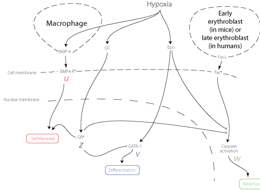
Figure 2.11: Scheme for the modeling of erythropoietic fate based on simplification of the biological scheme in Figure 6.2 (see Appendix 1). Four major variables that play a role in the intracellular regulation of CFU-E/Pro-EBs and affect the fate decisions to undergo apoptosis, terminal differentiation, or self-renewal are retained from Figure 6.2. They include : 1) the concentration of activated glucocorticosteroid receptor ( z ) that determines the rate of self-renewal in normal, steady-state erythropoiesis and in more limited hypoxia states in which adjustments of EPO concentrations maintain a stable number of circulating erythrocytes; 2) the concentration of activated BMP4 receptor ( u ) that determines the rate of expansion of the CFU-E/Pro-EB population in periods of hypoxic stress; 3) the concentration of GATA-1 ( v ) that determines the rate of terminal differentiation; and 4) the concentration of activated caspases ( w ) that determine the rate of apoptosis when elevated and the rate of terminal differentiation when reduced. The major extracellular mediators that affect the intracellular variables have been retained. These extracellular mediators include : 1) the concentration of glucocorticosteroid hormone (GC) that varies with degree of stress including that associated with hypoxia; 2) the expression of BMP4 by central macrophages that increases with hypoxia-induced stress; 3) the concentration of EPO which varies inversely with the degree of hypoxia; and 4) the expression of Fas by erythroid progenitor cells, which varies inversely with the EPO concentration and 5) Fas-ligand, which is produced by other erythroid cells in the erythroblastic island, specifically by early stage erythroblasts in mice and late-stage mature erythroblasts in humans.
