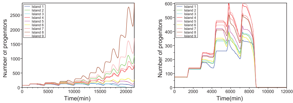
Figure 2.22: Number of progenitors in each island. Without feedback (left), some islands grow, some other disappear. In the case with feedback (right), after some time all islands disappear.
