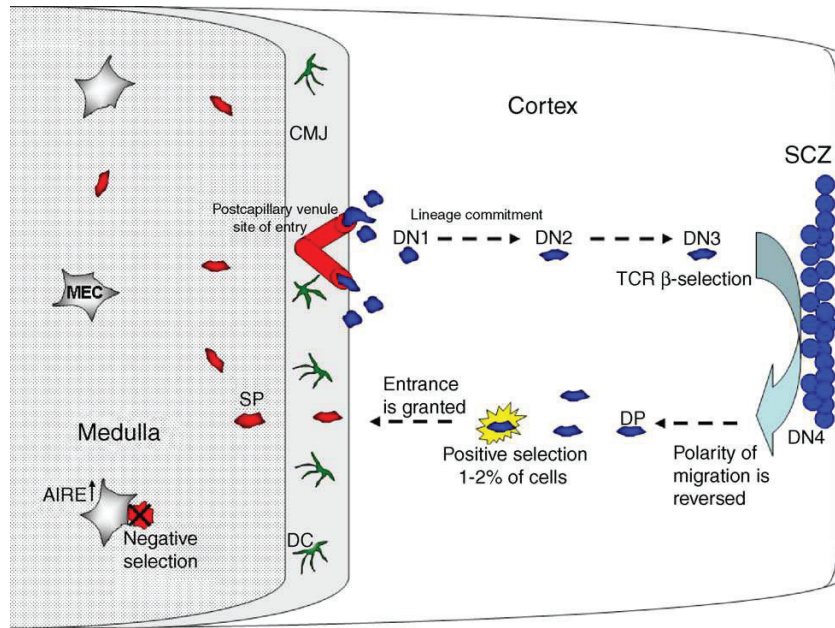
Figure 3.11: Intrathymic migration of developing thymocytes. T lineage precursors enter the thymus through post-capillary venules of the corticomedullary junction (CMJ) and then migrate outward to the subcapsular zone (SCZ) where they undergo TCR beta chain rearrangement and selection. At this time polarity of migration is reversed and CD4+CD8+ (DP) thymocytes move back into the cortex for alpha chain rearrangement and for testing of nascent TCR through positive selection. Post-selected thymocytes are granted access to the medulla where they are screened for self-reactivity through negative selection. Pattern and legend from [166].
