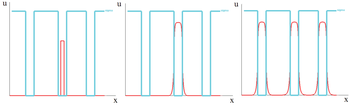
Figure 4.1: Initial condition and the snapshot of solution of equation (4.5.1) for t = 10 and t = 70 .
