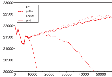
Figure 3.10: Number of erythrocytes in blood as a function of time for different values of the parameter p .
