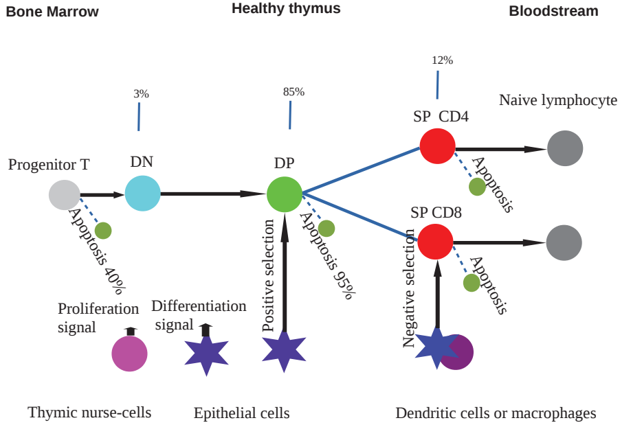
Figure 3.12: Differentiation pattern of normal cells.
