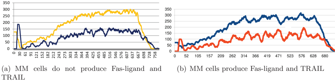
Figure 3.6: We can see the declining number of progenitors and of mature cells during the growth of tumors. Left: with cancer cells acting by mechanical actions (yellow curve - progenitors, blue curve - reticulocytes). Right: with cancer cells producing Fas-ligand and TRAIL (blue curve - progenitors, red curve - reticulocytes).
