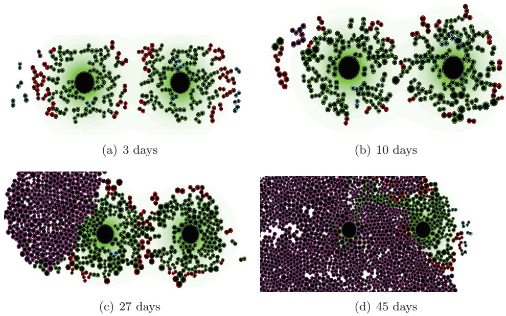
Figure 3.15: Development of tumor in the thymus. The number of malignant cells grows exponentially. They invade the thymus and push out normal cells. Cells shown in the figure: early thymocytes (gray), DN (blue), DP (green), SP (red), stromal cells (large purple cells), malignant cells (purple). Extracellular substances produced by nurse cells are shown as green halos.
