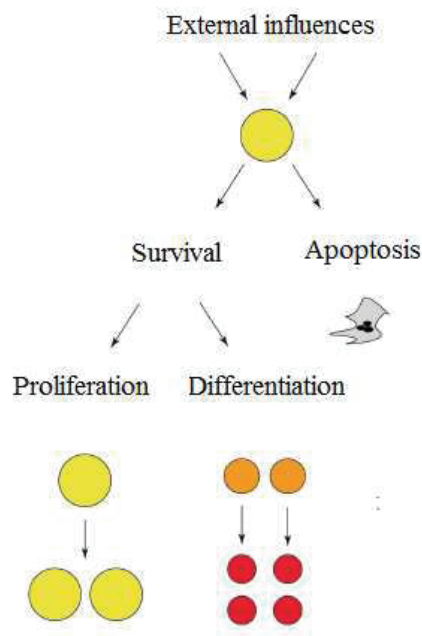
Figure 2.10: Schematic representation of erythroid progenitor cell decision making. Large yellow circles represent erythroid progenitors at the CFU-E/proerythroblast stage of differentiation. Their fate is determined by intracellular regulation which can be influenced by extracellular substances including Fas-ligand and EPO. This intracellular regulatory network is shown in greater detail in Figure 6.2. Erythroid progenitors have one of three possible fates : die by apoptosis, proliferate without differentiation (self-renewal), or terminally differentiate.
