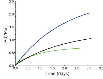
Figure 3.18: Ratio of intracellular drug concentration p(t) and the threshold p_{crit} during cellular cycle for k_+=2.10^{-3} , k_-=10^{-3} (blue), k_+=k_-=10^{-3} (black), k_+=10^{-3} , k_-=2.10^{-3} (green).
