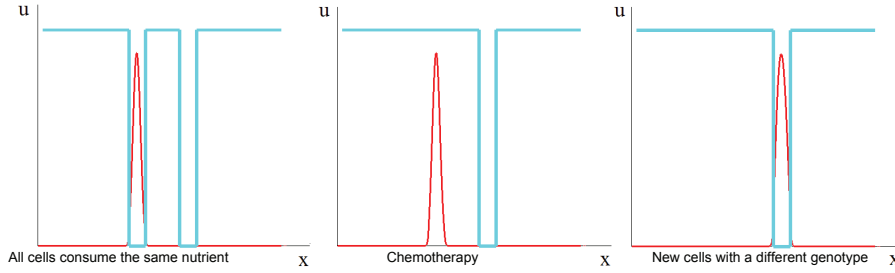
Figure 1.9: Development of the resistance to treatment. In the beginning all cells are located in the first survival gap. They do not appear in the other one because they do not have enough nutrients. If cells in the first survival gap are eliminated by chemotherapy, then more resistant cells in the second survival gap will appear.
