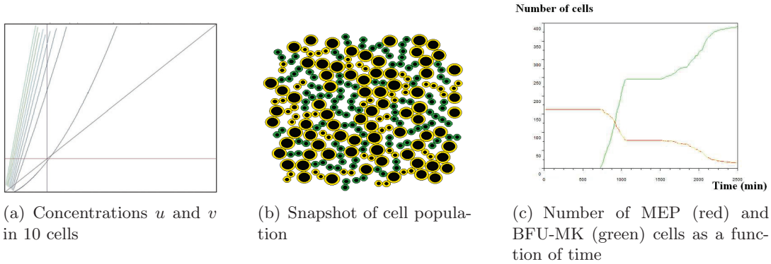
Figure 2.2: Evolution of the population of MEP cells for the values of parameters k_1^+ = 0.005 , k_1^- = 0.008 , k_2 = 0.01 , k_3^+ = 0.005 , k_3^- = 0.008 , k_4 = 0.1 . In Figure 2.2(a), curves of the phase space are majority located above the first bisector. MEP cells self-renew and differentiate into BFU-MK cell lineage as shown in Figure 2.1. The Figures 2.2(b) and 2.2(c) show the evolution towards BFU-MK cells and gradual disappearance of self-renewal.
