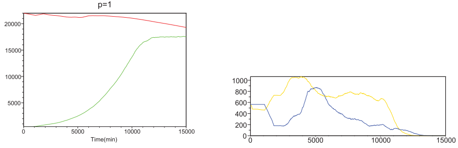
Figure 3.9: Cell number in time during multiple myeloma development: erythrocytes in blood (red), multiple myeloma cells (green), progenitors (yellow), mature cells (blue).
