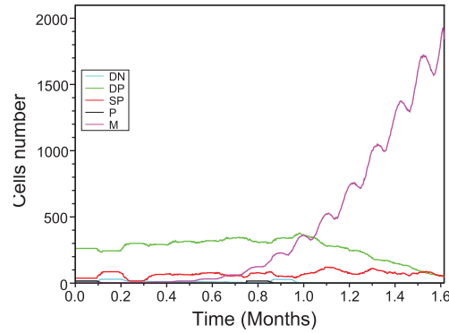
Figure 3.16: The number of cells before and during the development of tumor. The number of malignant cells grows exponentially, the number of normal cells decreases. The curve showing the number of malignant cells is purple, the corresponding curves for normal cells are blue, green and red.
