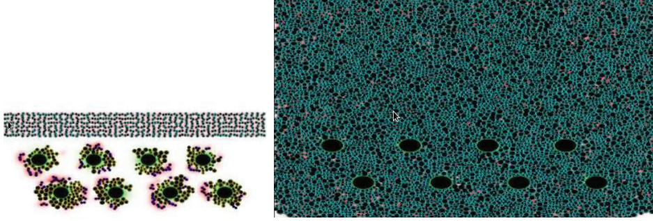
Figure 3.5: Left: appearance of the tumor (light blue cells in the top of the figure). Right: tumor invasion after 2 months.
