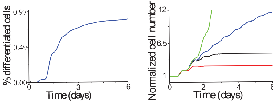
Figure 2.6: Left: proportion of differentiated cells (reticulocytes, erythrocytes) to all cells over time. Right: accumulation of total number of cells. Different curves correspond to different amplitude of stochastic variation of initial activities of ERK and Fas in newly formed cells. Blue curve corresponds to the case where the initial activity of ERK is between 0 and 0.015, Fas between 0 and 0.01, with a uniform probability distribution. Red, black and green curves correspond to \sigma=0.15, 0.01, 0.007 respectively (see the explanation in the text). Normalized cell number: the ratio of the current cell number to the initial cell number. The initial cell number is 2.10^5 for the experiment and 98 for the numerical simulations. Curves made with the mean of 3 simulations.
