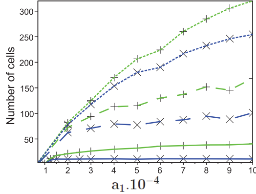
Figure 2.12: Average number of CFU-E/Pro-EBs and differentiating erythroblasts (green curves) and late-stage, pre-enucleation erythroblasts and reticulocytes (blue curves) in one erythroblastic island as a function of a_1 for different values of w_{cr} equal to 0.7 (upper pair of curves), 0.6 (middle pair of curves) and 0.509 (lower pair of curves), respectively. Fas-ligand produced by early stage erythroblasts. The average is taken with respect to time and with respect to 10 simulations.
