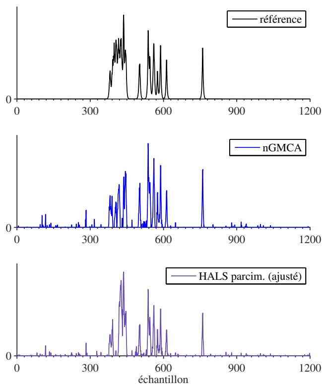
Figure IV.19 – Exemple de reconstruction (lactose, SNR_Y = 15 dB)
