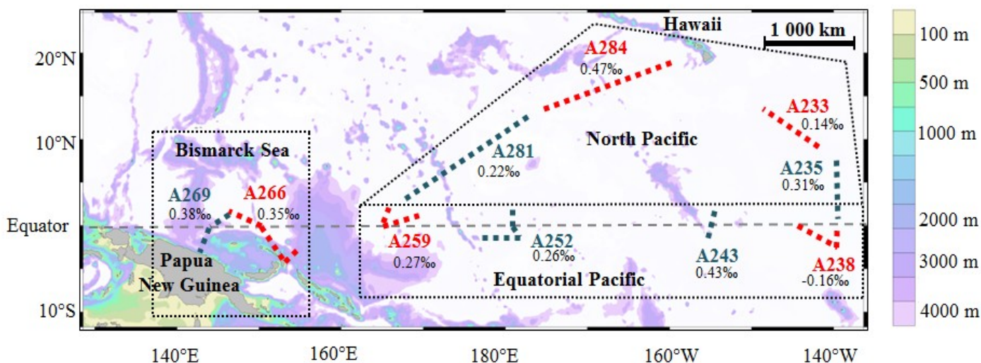
182 183 Figure 3. Maps of aerosol sampling. Depths greater than 4000m are white. Aerosols sampling 184 transects are shown by the color dotted lines. The Fe isotopic compositions are indicated 185 under the sample names. Three areas discussed in the text are shown: the North Pacific, the 186 equatorial Pacific and the Bismarck Sea.
