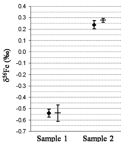
Figure 4. Results of a blind test, (◆) measurements performed following the protocol of Poitras and Freydisse. 42 Sample 1, \delta^{56}\text{Fe} = -0.540 \pm 0.034 (2SE, n = 9 ); sample 2, \delta^{56}\text{Fe} = +0.237 \pm 0.035 (2SE, n = 6 ). (–) measurement performed following the protocol presented in this study; sample 1, \delta^{56}\text{Fe} = -0.539 \pm 0.072 (2SD, n = 3 ); sample 2, \delta^{56}\text{Fe} = +0.276 \pm 0.017 (2SD, n = 3 ).
