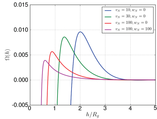
FIGURE 3.30: Thermodynamic potential, Fig.3.29, zoomed in around \Omega(x) \simeq 0 .
