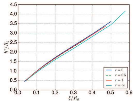
FIGURE 3.55: The SCFT barrier position calculated for spherical geometry via Eq.(3.77) as a function of the correlation length.
