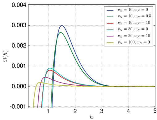
FIGURE 4.16: The thermodynamic potential, Eq.(4.7), for different values of the virial parameters, v_N , w_N . Fixed parameters: A = 61.5 and N_x = 10k , N_s = 10k .
