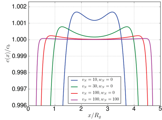
FIGURE 3.28: Concentration profiles, Fig.3.27, zoomed around c(x)/c_b \simeq 1.0 .
