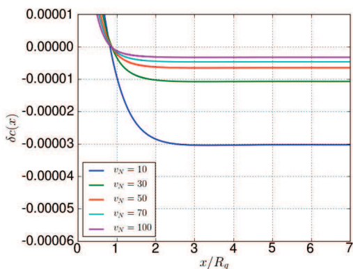
FIGURE 5.7: The relative difference between the SCFT and the analytical concentration profiles, \delta c(x) = (c(x) - f(x))/f(x) , where f(x) is the concentration profile obtained analytically, Eq.(5.17), and c(x) = \phi_f(x)/\phi_b is the solution obtained numerically, for different v_N . Fixed parameters: r_b = 1 , N_x=8k , N_s=3k .
