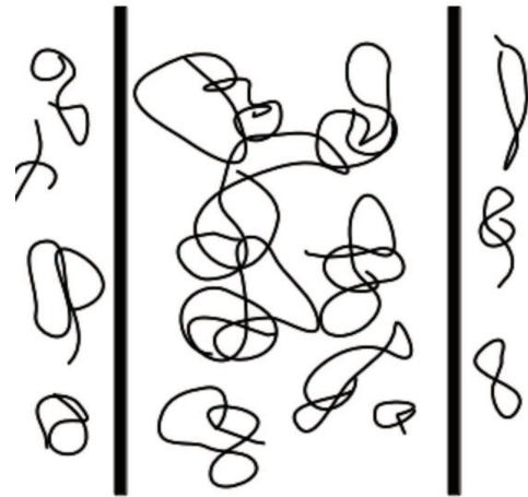
FIGURE 3.2: Representation of Derjaguin approximation.
