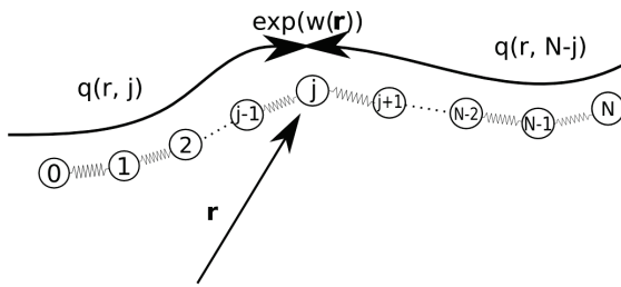
FIGURE 2.5: The statistical independence of sub-chains with j + 1 and N - j + 1 beads.
