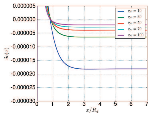
FIGURE 5.8: The relative difference between the SCFT and the analytical concentration profiles, \delta c(x) = (c(x) - f(x))/f(x) , where f(x) is the concentration profile obtained analytically, Eq.(5.17), and c(x) = \phi_f(x)/\phi_b is the solution obtained numerically, for different v_N . Fixed parameters: r_b = 1 , N_x=15k , N_s=5k .
