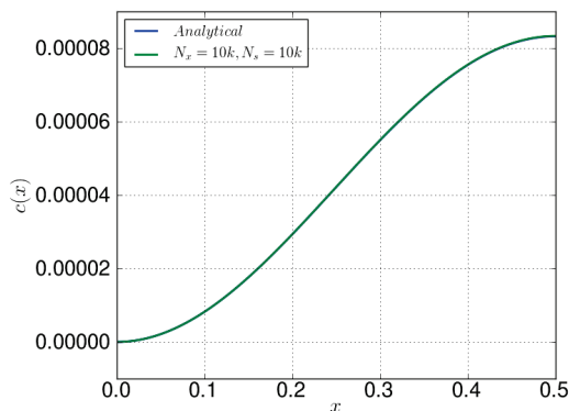
FIGURE 3.15: The concentration profile calculated for h_m = 0.5 , N_x = 10k , N_s = 10k .
