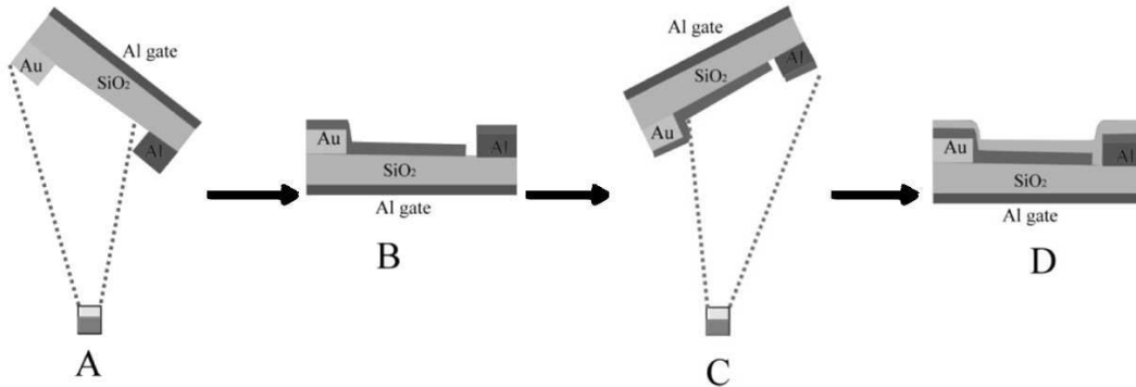
Figure 1.22: Schematic illustration of the laterally arranged heterojunction fabrication process. A: the substrate is tilted with respect to the horizontal plane and pentacene is evaporated resulting in the layer deposition shown in B. C: the substrate is inclined in the opposite direction and \text{Alq}_3 is evaporated resulting in the final configuration shown in D. Source: [79].
