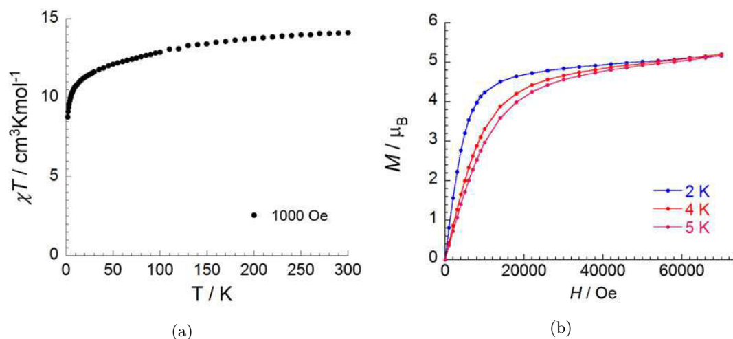
Figure 6.11: (a) Plot of \chi T versus T for [\text{Dy}(\text{Op})_2\text{Cl}(\text{HOp})(\text{EtOH})] 32 in the range of 1.8-300 K at 1000 Oe. (b) Plot of M versus H for [\text{Dy}(\text{Op})_2\text{Cl}(\text{HOp})(\text{EtOH})] 32 at 2 K, 4 K and 5 K.
