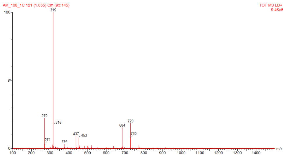
Figure B.56: MALDI-TOF of Al(q 2 Acac) 28 .
