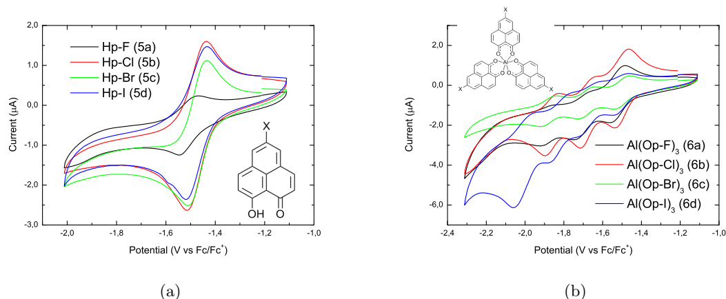
Figure 3.39: (a) Cathodic cyclic voltammogram at room temperature in DCM of the halogenated ligands HO p -X 5a-d . Electrolyte: TBAPF 6 . Scan rate: 100 mV s -1 . (b) Cathodic cyclic voltammogram at room temperature in DCM of the halogenated complexes Al(Op-X) 3 6a-d . Electrolyte: TBAPF 6 . Scan rate: 100 mV s -1 .
