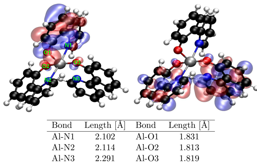
Figure 4.4: Molecular orbital surfaces of the HOMO (left) and LUMO (right) and list of the bond lengths of mer\text{-Al}(\text{Op-py})_3 . The labels of the atoms are exemplary shown in green on the atoms in the molecule on the left-hand side (HOMO).
