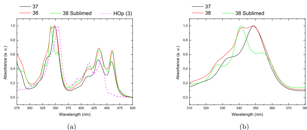
Figure 6.9: (a) Absorption spectra at room temperature of diluted DMSO solutions of 37 , 38 , before and after the sublimation process, and HOOp 3 (for comparison). (b) Magnification of the absorption spectra in the region between 310 and 380 nm. All the spectra are normalized.
