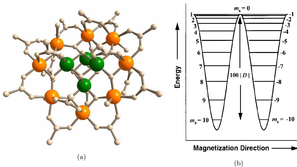
Figure 1.31: (a) Crystal structure of the first SMM [\text{Mn}_{12}\text{O}_{12}(\text{OAc})_{16}(\text{H}_2\text{O})_4] ( \text{Mn}_{12}\text{Ac} ). The total spin of the molecule is S= 10 given by 4 \text{Mn}^{4+} ions, S= 6 ( \text{Mn}^{4+} : S= 3/2 ) plus 8 \text{Mn}^{3+} ions, S= 16 ( \text{Mn}^{3+} : S= 2 ). (b) Plot of the potential energy versus the magnetization for a SMM with S= 10 ground state. The diagram is for zero external magnetic field. Source: [118, 122, 123].
