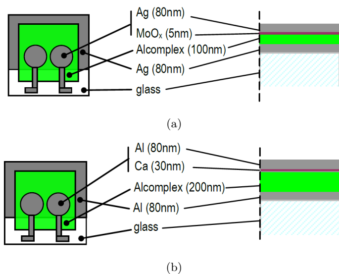
Figure 4.18: (a) Schematic representation of a hole AS setup: Ag [80 nm]/Al-complex [100 nm]/ \text{MoO}_x [5 nm]/Ag [80 nm]. (b) Schematic representation of an electron AS setup: Al [80 nm]/Al-complex [200 nm]/Ca [30 nm]/Al [80 nm].
