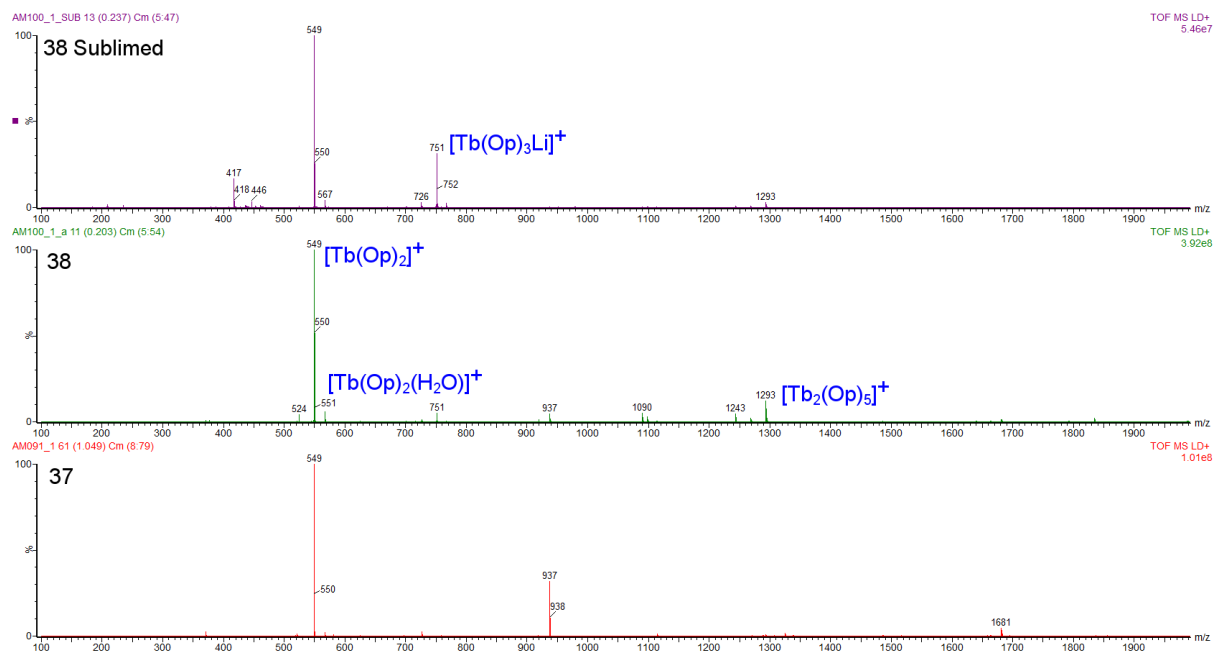
Figure 6.7: MALDI-TOF spectra of the phenalenyl-based terbium complexes 37 and 38 before and after the sublimation process. The corresponding fragments are reported next to peak. In Table 6.2 are listed the fragments and their relative intensities.
