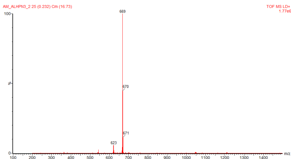
Figure B.37: MALDI-TOF of \text{Al}(\text{Op-n})_3 16b .
