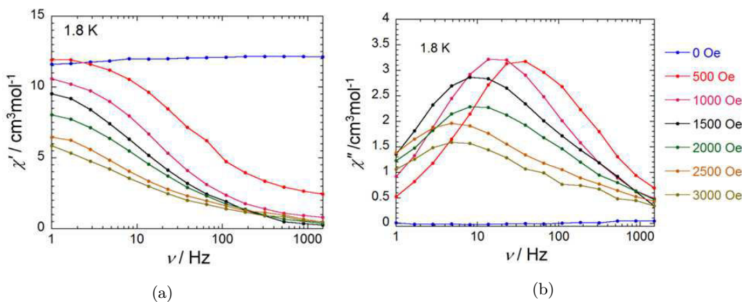
Figure 6.18: Frequency dependence of the in-phase \chi' (a) and of the out-of-phase \chi'' (b) ac magnetic susceptibility at 1.8 K and different dc fields for [\text{Dy}(\text{Op})_3(\text{HOOp})] 33 - [\text{Dy}(\text{Op})_3(\text{EtOH})] 34 .
