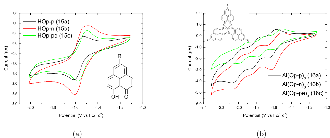
Figure 3.40: (a) Cathodic cyclic voltammogram at room temperature in DCM of the substituted ligands HO p -R 15a-c . Electrolyte: TBAPF 6 . Scan rate: 100 mV s -1 . (b) Cathodic cyclic voltammogram at room temperature in DCM of Al(Op-R) 3 16a-c . Electrolyte: TBAPF 6 . Scan rate: 100 mV s -1 .
