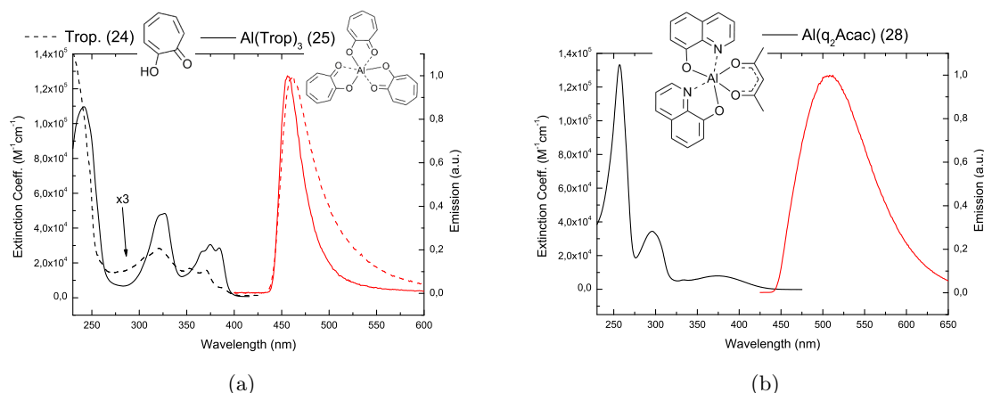
Figure 3.33: (a) Absorption (black) and fluorescence (red) spectra at room temperature in diluted DCM solution of Tropolone 24 and \text{Al}(\text{Trop})_3 25 . (b) Absorption (black) and fluorescence (red) spectra at room temperature in diluted DCM solution of \text{Al}(\text{q}_2\text{Acac}) 28 .
