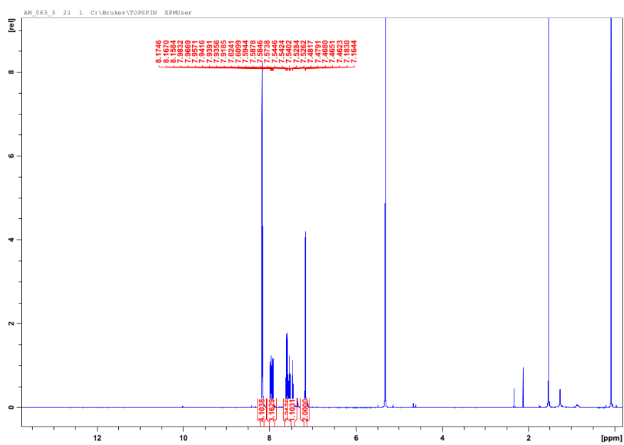
Figure B.35: ^1\text{H} -NMR of \text{Al}(\text{Op}-n)_3 16b .
