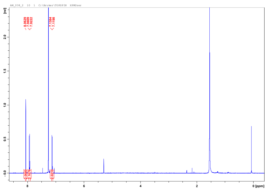
Figure B.21: ^1\text{H} -NMR of \text{Al}(\text{Op}-\text{Br})_3 6c .
