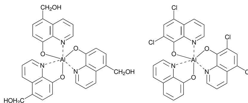
Figure 1.11: Chemical structure of \text{AlOq}_3 (tris-(5-hydroxymethyl-8-quinolinato)aluminum) on the left hand side and \text{Alq}(\text{Clq})_2 (bis-(5,7-dichloro-8-quinolinato)-(8-quinolinato)aluminum) on the right hand side. Sources: [58, 59].
