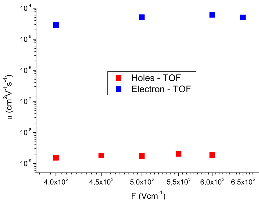
Figure 4.19: Charge carrier mobility of electrons and holes measured for the sample ITO/FI3 [200 nm]/Alq 3 [2 μm]/Al [100 nm]. Applied field F for electron mobility: 4.0 \times 10^5 \text{ V cm}^{-1} - 6.5 \times 10^5 \text{ V cm}^{-1} ; for hole mobility: 4.0 \times 10^5 \text{ V cm}^{-1} - 6.0 \times 10^5 \text{ V cm}^{-1} .
