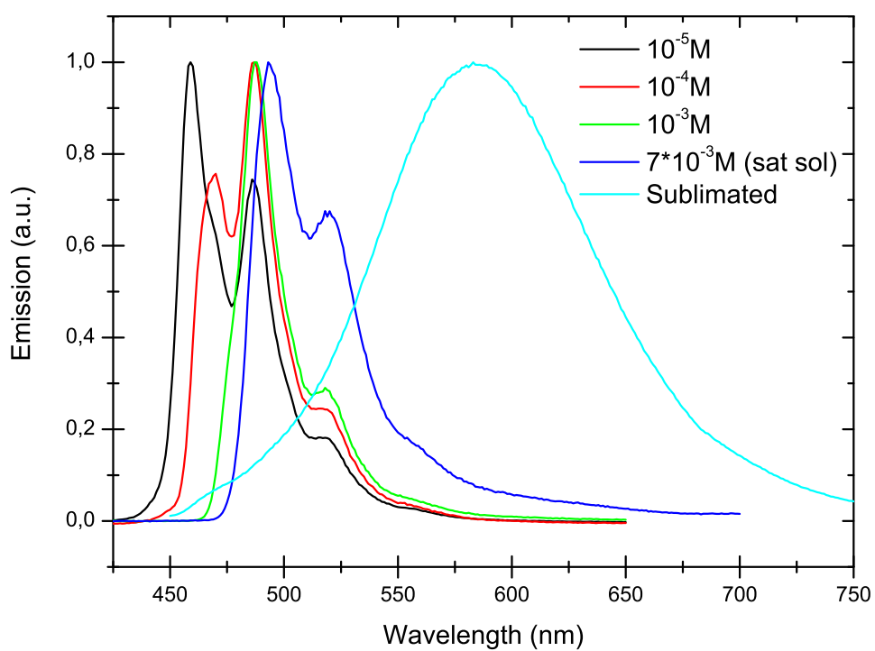
Figure D.2: Emission in function of the concentration of Al(OP)_3 4.
