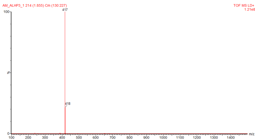
Figure B.3: MALDI-TOF of \text{Al}(\text{Op})_3 4.
