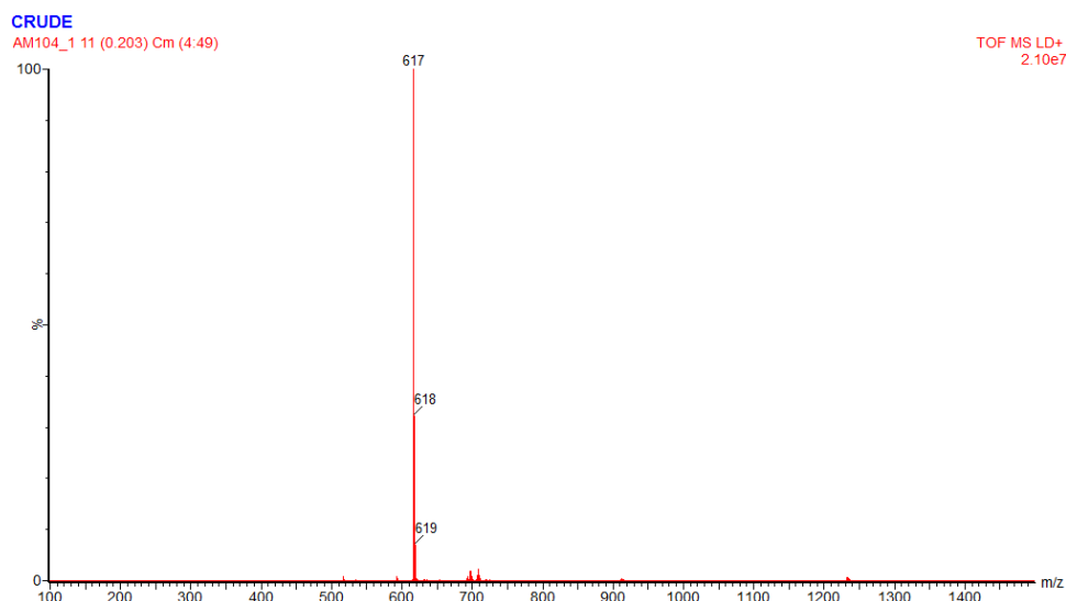
Figure B.42: MALDI-TOF of \text{Al}(\text{Op-pe})_3 16c .
