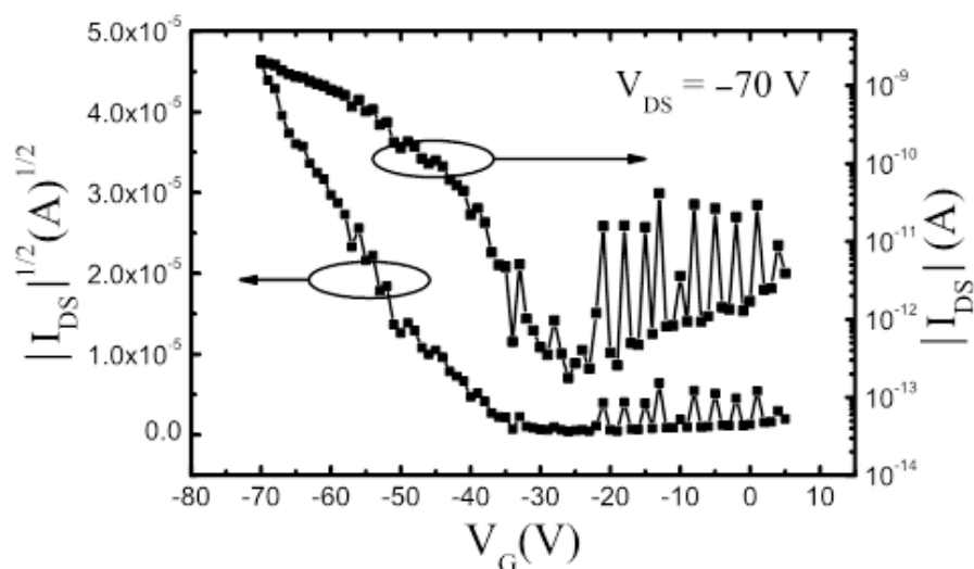
Figure 4.14: Holes transfer curve of the \text{Al}(\text{Op})_3 -based TFT with a channel length of 100 \mu\text{m} . In this image, I_{DS} and V_{DS} are the source-drain currents. V_G refers to the gate voltage. The hole mobility extrapolated by the transfer characteristics range between 0.6 \times 10^{-6} and 2.1 \times 10^{-6} \text{ cm}^2 \text{ V}^{-1} \text{ s}^{-1}
