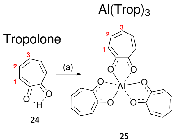
Scheme 3.7: Al(Tropolone) 3 25 . (a) AlCl 3 , toluene, reflux, overnight, yield: 83%.
