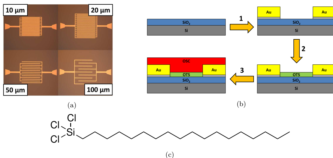
Figure 4.16: (a) Scanning electron microscopy images of the patterned source and drain electrodes. The channel length vary from 10 \mu\text{m} (width to length ratio, W/L = 2000 ) to 100 \mu\text{m} ( W/L = 50 ). (b) Schematic procedure of the TFT fabrication. Step 1: Source and drain electrodes patterning. Step 2: OTS modification. Step 3: OSC deposition. (c) Chemical structure of OTS (trichlorooctadecylsilane).
