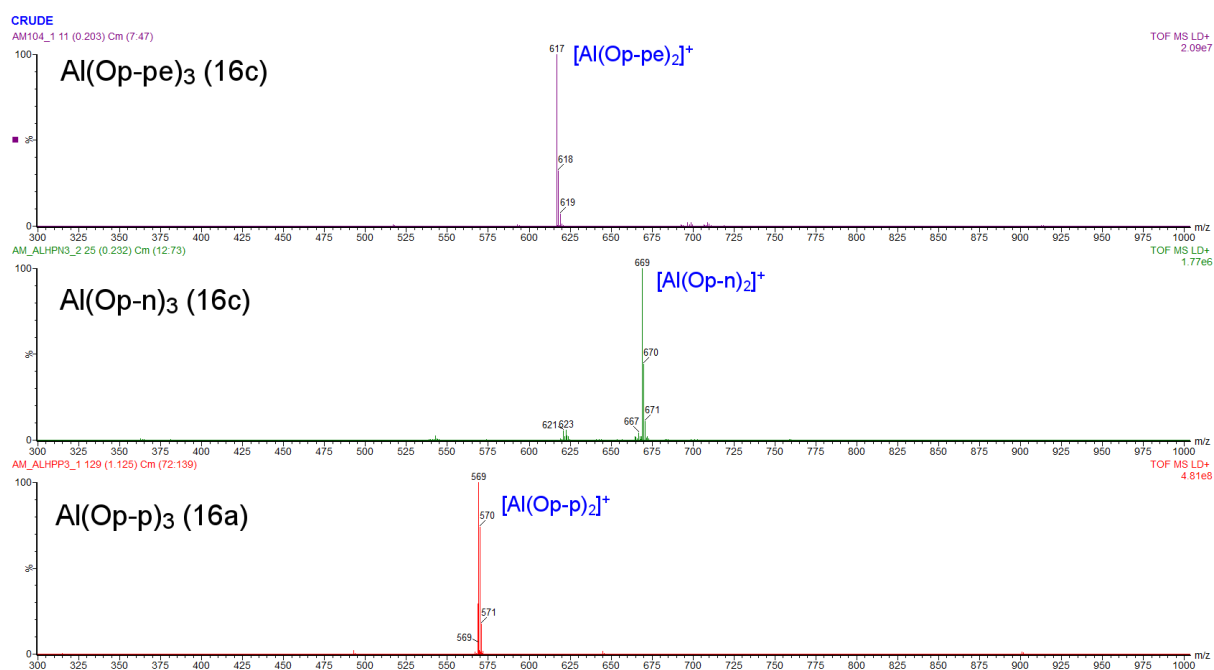
Figure 3.12: MALDI-TOF spectra of Al(O p -R) _3 16a-c . The main fragments are marked in the figure.
