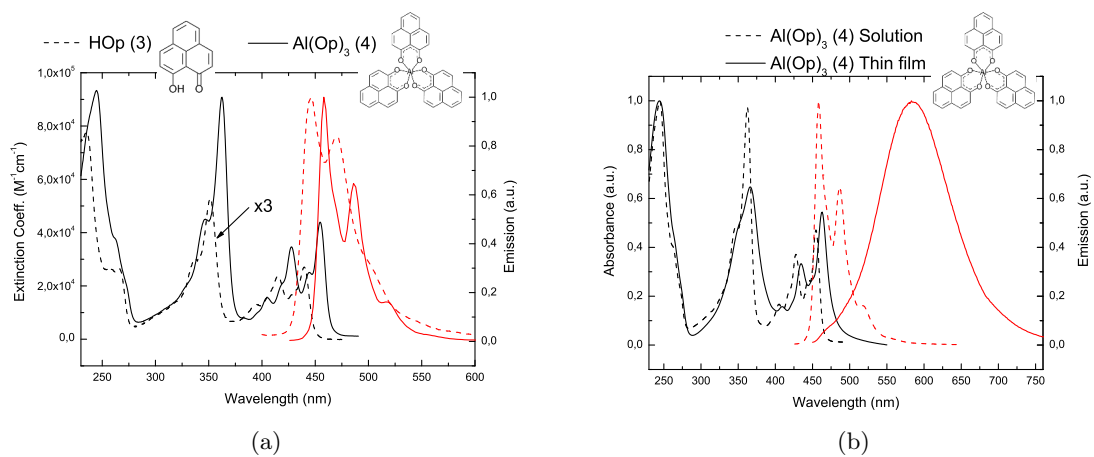
Figure 3.26: (a) Absorption (black) and fluorescence (red) spectra at room temperature in diluted DCM solution of Hp 3 and Al(Op) 3 4 . (b) Absorption (black) and fluorescence (red) spectra at room temperature in solution and in thin film of Al(Op) 3 4 .
