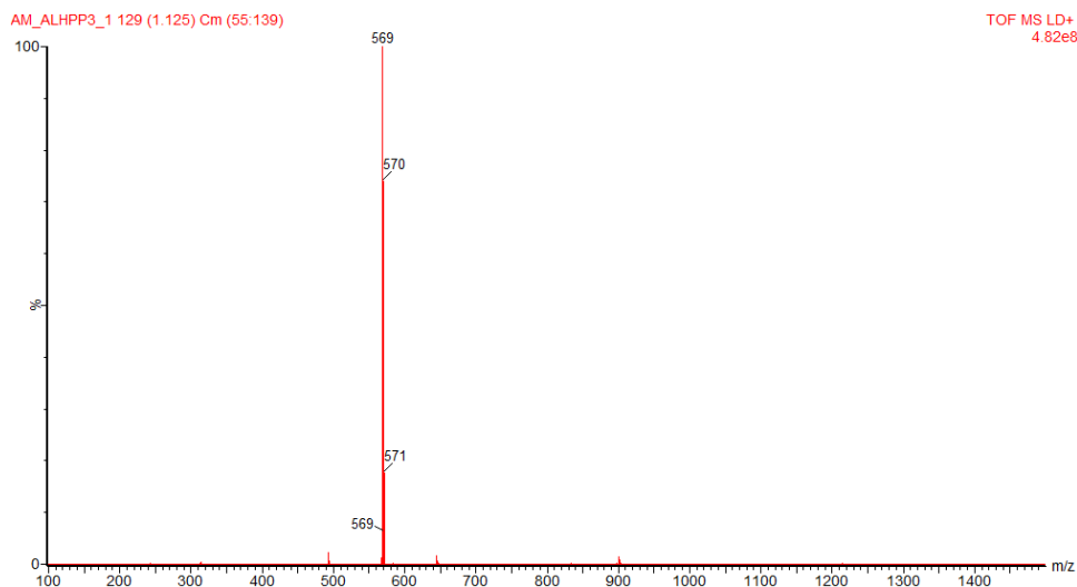
Figure B.32: MALDI-TOF of \text{Al}(\text{Op-p})_3 16a .
