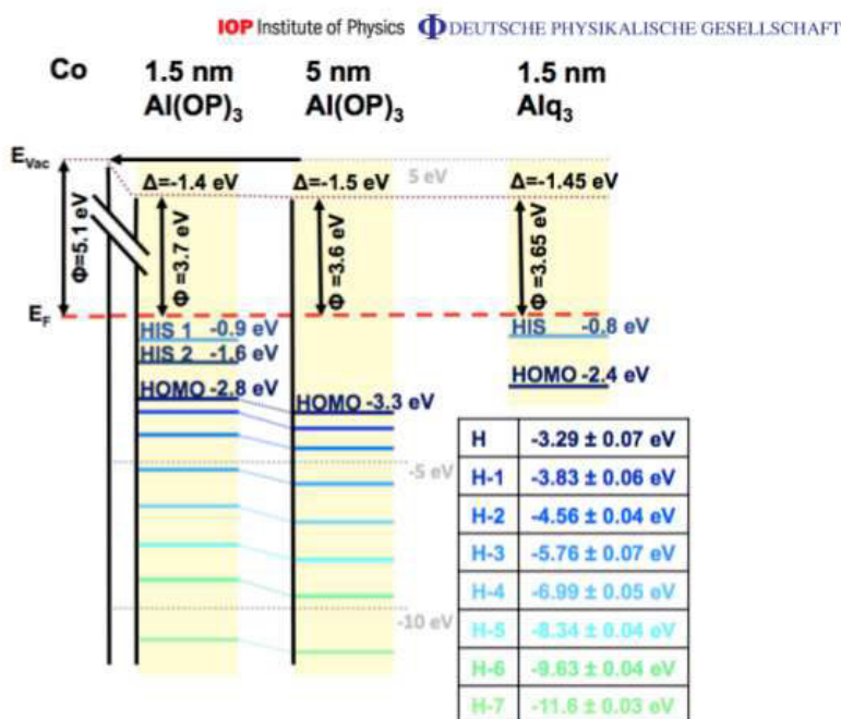
Figure 6. Energy level alignment of the Co/[ x nm]Al(OP) 3 system for x = 1.5 and 5 nm compared to the energy level alignment of the Co/Alq 3 interface. The energy level alignment for x = 1.5 nm is extracted from the NT-PS spectra and reflects the alignment of the Co/Al(OP) 3 spinterface. The alignment for x = 5 nm reflects the occupied manifold of bulk Al(OP) 3 and is extracted from the UPS spectra. The alignment at the Co/Alq 3 interface is taken from [11].
