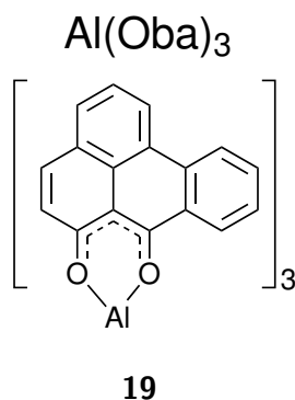
Scheme 8.21: \text{Al}(\text{Oba})_3 19 .
