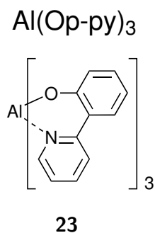
Scheme 8.23: \text{Al}(\text{Op-py})_3 23 .
