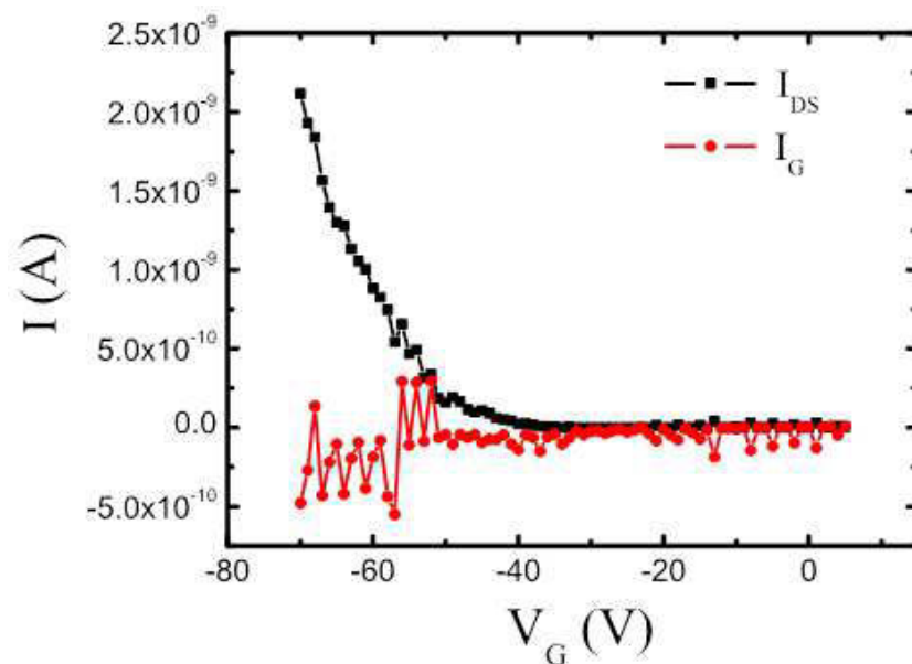
Figure 4.15: Comparison of the source-drain current I_{DS} and the leakage gate current I_G from transfer characterization of the \text{Al}(\text{Op})_3 based TFT with a channel length of 100 \mu\text{m} . The source-drain bias V_{DS} for this measurement is -70 \text{ V} .
