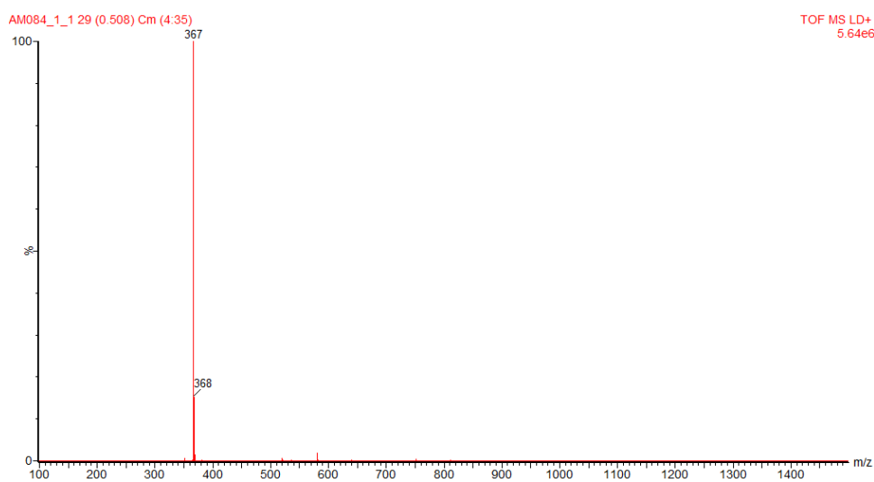
Figure B.49: MALDI-TOF of \text{Al}(\text{Op-py})_3 23 .
