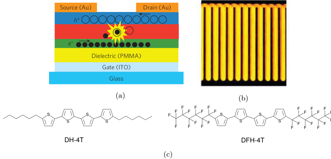
Figure 1.23: (a) Schematic representation of the trilayer LE-OFET device. Field-effect charge transport and light-generation processes are illustrated. (b) Optical micrograph of the light emission from the trilayer LE-OFET ( V_{SD} = V_G = 90 V). (c) Chemical structure of the p -type OSC DH-4T (blue layer) and of the n -type OSC DFH-4T (green layer). Source:[80].
