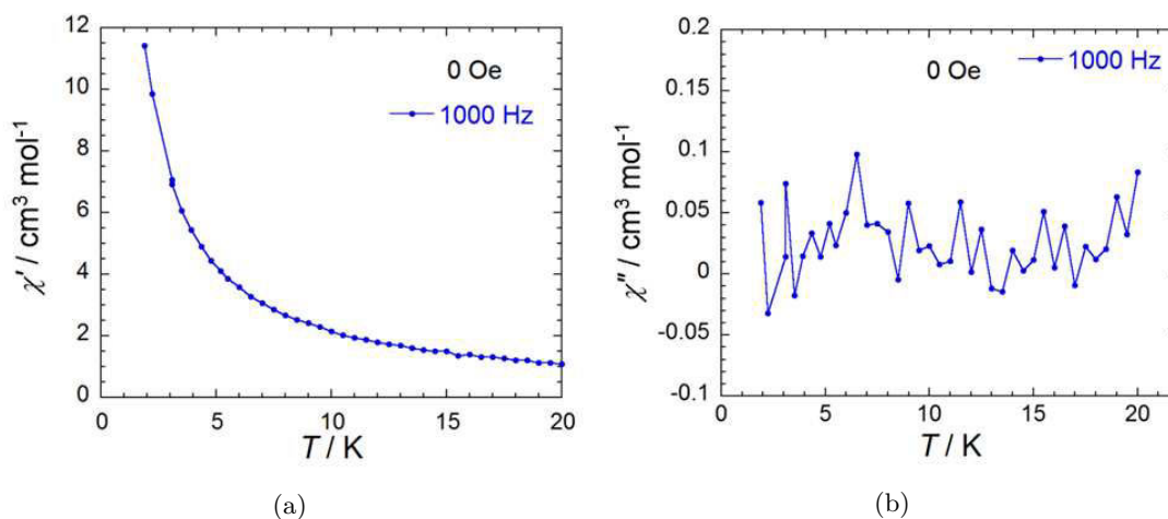
Figure 6.17: ac magnetic susceptibility measurements under zero dc field for [\text{Dy}(\text{Op})_3(\text{HOOp})] 33 - [\text{Dy}(\text{Op})_3(\text{EtOH})] 34 . Temperature dependence of the in-phase \chi' (a) and of the out-of-phase \chi'' (b) ac magnetic susceptibility.
