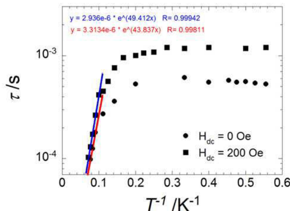
Figure 6.13: Arrhenius semilogarithmic plots of the relaxation time \tau versus 1/T for [\text{Dy}(\text{Op})_2\text{Cl}(\text{HOp})(\text{EtOH})] 32 from ac susceptibility measurements under a zero dc field and a dc field of 200 Oe. The solid lines represent a linear fit in the thermally activated range of temperature.
