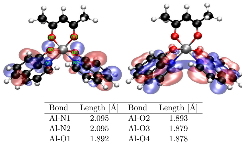
Figure 4.7: Molecular orbital surfaces of the HOMO (left) and LUMO (right) and list of the bond lengths of \text{Al}(\text{q}_2\text{Acac}) . The labels of the atoms are exemplary shown in green on the atoms in the molecule on the left-hand side (HOMO orbital).
