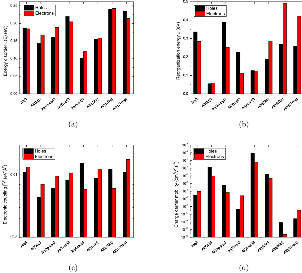
Figure 4.13: Microscopic parameters computed for holes and electrons of the OSCs in the morphologies. (a) Energy disorder \sigma(E) . (b) Reorganization energy \lambda . (c) Electronic coupling J^2r^2 . (d) Charge carriers mobility \mu .
