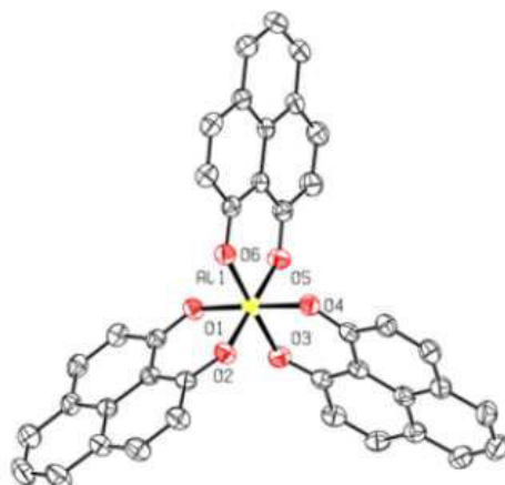
Figure 1. Molecular structure of Al(OP) 3 (hydrogen atoms and solvent molecules are omitted for clarity).
