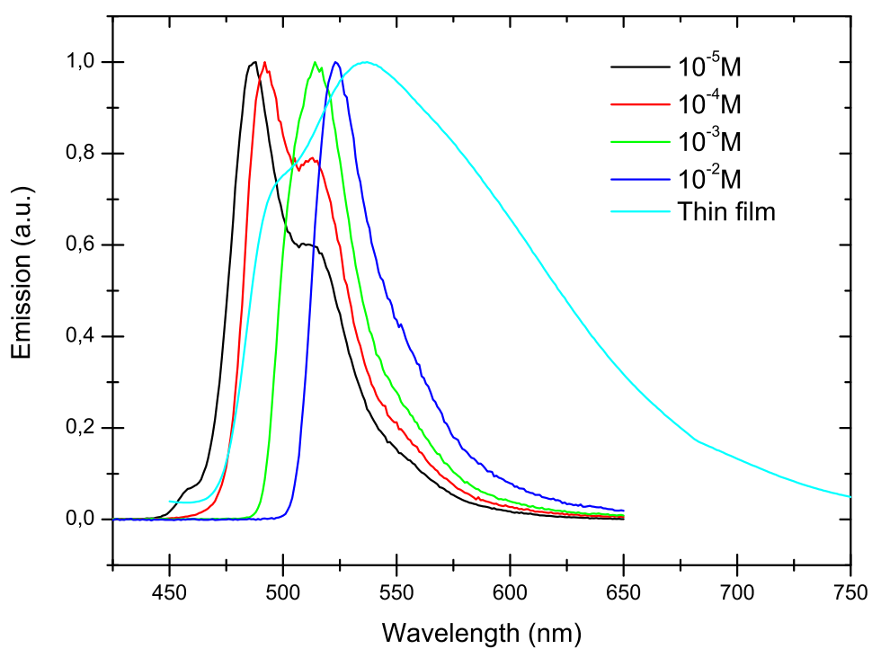
Figure D.3: Emission in function of the concentration of \text{Al}(\text{Op-p})_3 16a .
