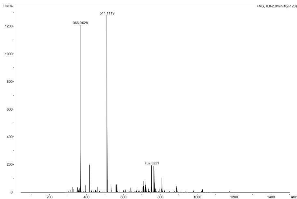
Figure B.58: ESI-TOF of Al(q 2 Op) 29 .
