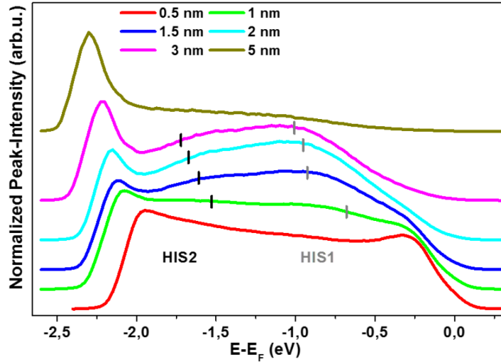
Figure 5.3: Normalized NT-PS spectra of the Co/[ x nm] Al(Op) 3 system ( x=0 nm, 0.5 nm, 1 nm, 1.5 nm, 2 nm, 3 nm and 5 nm). The energetic positions of the two interface states HIS1 and HIS2, detectable for 1 \leq x \leq 3 are marked in the spectra.
