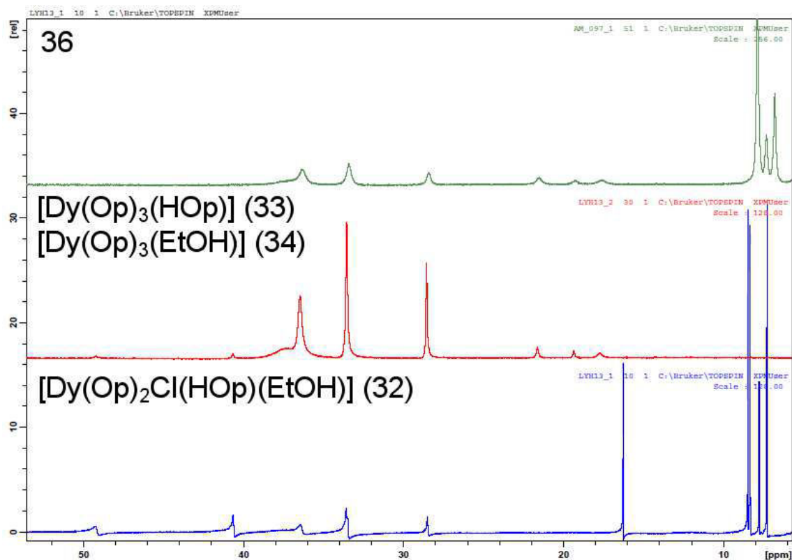
Figure 6.4: Paramagnetic ^1\text{H-NMR} spectra in \text{DMSO-}d_6 of the phenalenyl-based dysprosium complexes [\text{Dy}(\text{Op})_2\text{Cl}(\text{HOpe})(\text{EtOH})] , 32 [\text{Dy}(\text{Op})_3(\text{HOpe})] 33 - [\text{Dy}(\text{Op})_3(\text{EtOH})] 34 and 36 .
