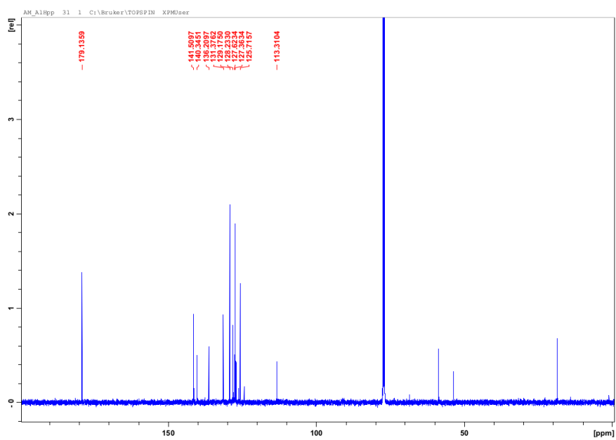
Figure B.31: ^{13}\text{C-NMR} of \text{Al}(\text{Op-p})_3 16a .
