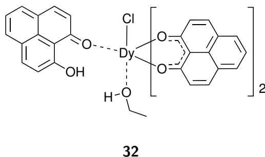
Scheme 8.29: [Dy(Op) 2 Cl(HOp)(EtOH)] 32 .
