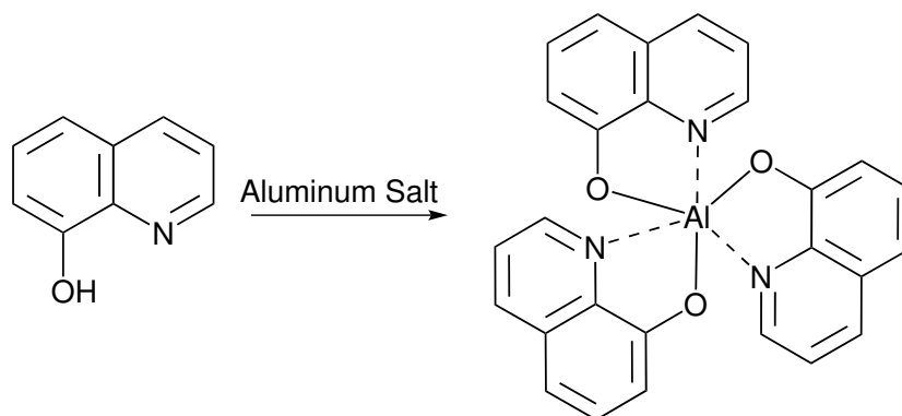
Scheme 1.1: Synthesis of mer - Alq_3 . Aluminum salt: AlCl_3 , Al(NO_3)_3 \cdot 9H_2O or Al(SO_4)_3 \cdot 6H_2O .
