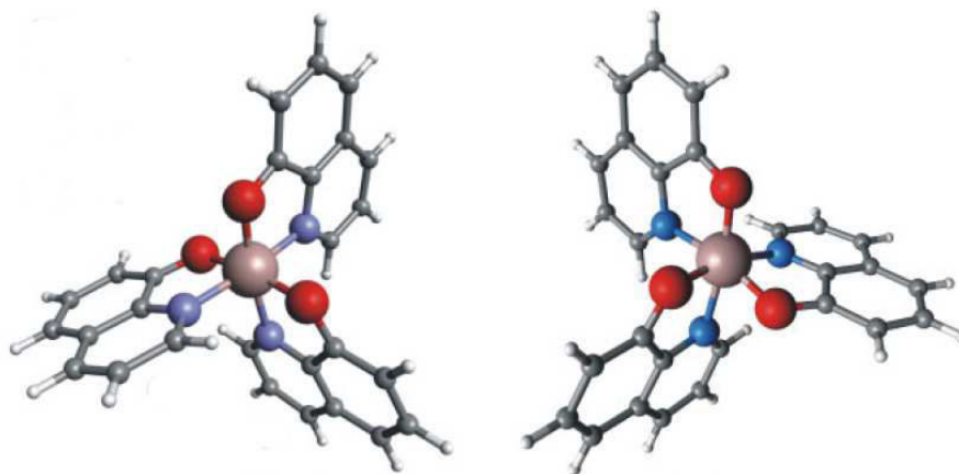
Figure 1.6: Molecular structures of the meridional isomer ( mer-Alq_3 ) on the left hand side, and of the facial isomer ( fac-Alq_3 ) on the right end side. Source: [27].
