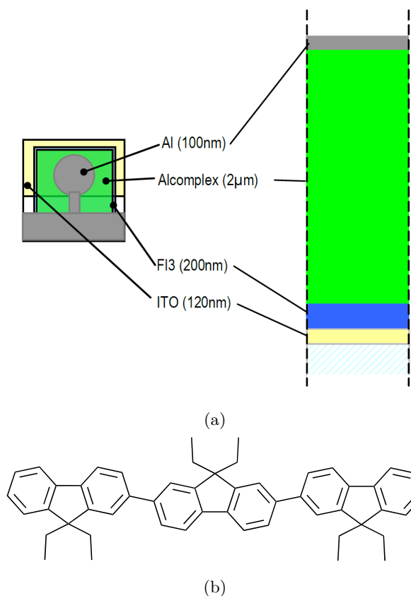
Figure 4.17: (a) Schematic representation of the ambipolar sample used in our experiments ITO/FI3 [200 nm]/Al-complex [2 \mu\text{m} ]/Al [100 nm]. The OSC was sandwiched between a transparent ITO electrode and an aluminum electrode. A charge generation layer (CGL) of FI3 (ter(9,9'-diethylfluorene)) was inserted to increase the absorption at the \text{N}_2 laser emission wavelength (337 nm). (b) Chemical structure of FI3.
