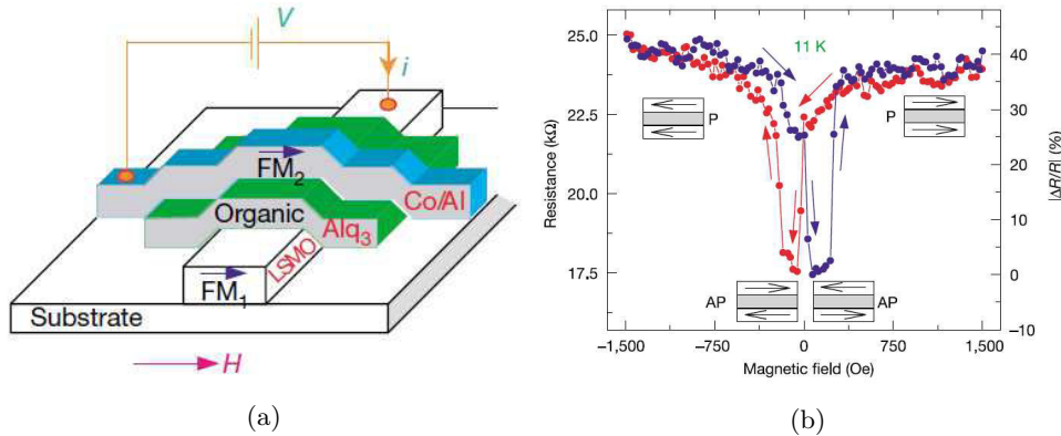
Figure 1.17: (a) Schematic representation of a typical vertical Alq_3 -based OSPD. Alq_3 is sandwiched between LSMO, bottom electrode, and cobalt, top electrode. (b) MR loop of a LSMO [100 nm]/ Alq_3 [130 nm]/Co [3.5 nm] OSPD measured at 11 K. The magnetization configuration of the electrodes is indicated. Source: [69].
