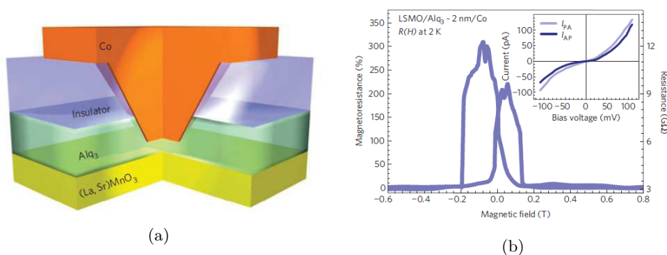
Figure 1.18: (a) Schematic representation of the AlQ 3 -based OSPD device. A nanoindent is realized in the AlQ 3 layer to control the organic tunnel barrier thickness. The nanohole is then filled with cobalt. LSMO is the bottom electrode and cobalt the top electrode. (b) MR curve of a LSMO/AlQ 3 [2 nm]/Co OSPD measured at 2 K and -5 mV. In the inset, I(V) curves recorded at 2 K in the parallel ( I_{PA} ) and antiparallel ( I_{AP} ) configurations. Source: [74].
