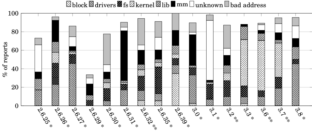
Figure 3.16: Top 6 services containing invalid pointer references
