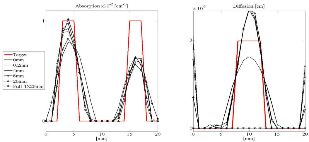
Fig. 4-28 : Influence of the sources shape: cross-plots extracted from Fig. 4-27 of reconstructed perturbation absorption \delta\mu_a and diffusion \mathcal{D} coefficient maps with with 4 points sources; 4 line sources with a length of 0.2 mm; 4 mm; 8 mm; 26 mm and full field of view probing with one single source composed of 4 lines of 26 mm length.
