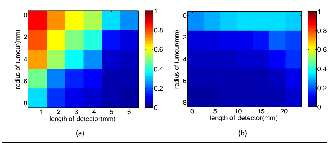
Fig. 4- 8 quadratic error map of (a) sparse detectors, (b) intense detectors.
